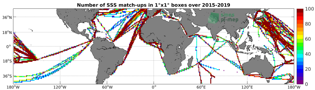
Figure 4: Number of SSS match-ups between TSG (LEGOS-DM) SSS and the SMAP SSS L3 v4 - Monthly (RSS) SSS product for the Mid-Low Latitudes 45N-45S Pi-MEP region over 1°x1° boxes and for the full satellite product period.
