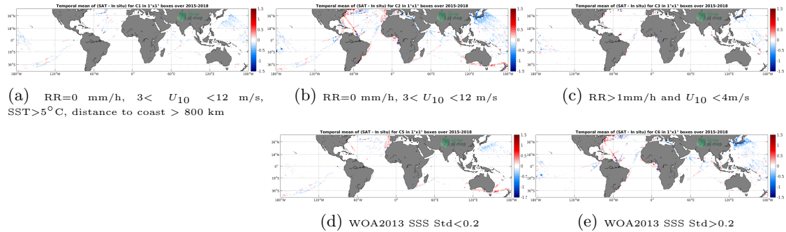
Figure 12: Temporal mean gridded over spatial boxes of size 1^\circ \times 1^\circ of \Delta SSS (SMAP-L3-RSS-V4-MONTHLY - TSG-LEGOS-DM) for 5 different subdatasets corresponding to: RR=0 mm/h, 3 < U_{10} < 12 m/s, SST > 5^\circ\text{C} , distance to coast > 800 km (a), RR=0 mm/h, 3 < U_{10} < 12 m/s (b), RR > 1 mm/h and U_{10} < 4 m/s (c), WOA2013 SSS Std < 0.2 (d), WOA2013 SSS Std > 0.2 (e).
