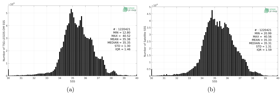
Figure 2: Histograms of SSS from TSG-LEGOS-DM (a) and SMAP-L3-RSS-V4-MONTHLY (b) considering all match-up pairs per bins of 0.1 over the Mid-Low Latitudes 45N-45S Pi-MEP region and for the full satellite product period.
