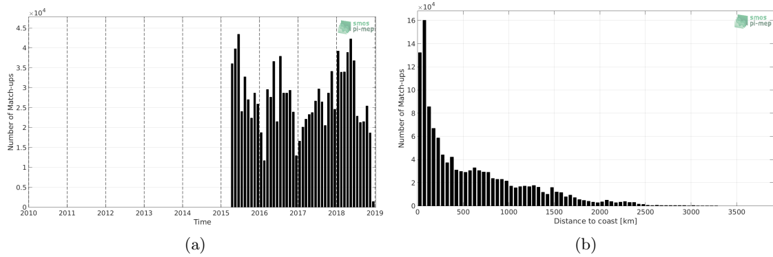
Figure 1: Number of match-ups between TSG-LEGOS-DM and SMAP-L3-RSS-V4-MONTHLY SSS as a function of time (a) and as function of the distance to coast (b) over the Mid-Low Latitudes 45N-45S Pi-MEP region and for the full satellite product period.
