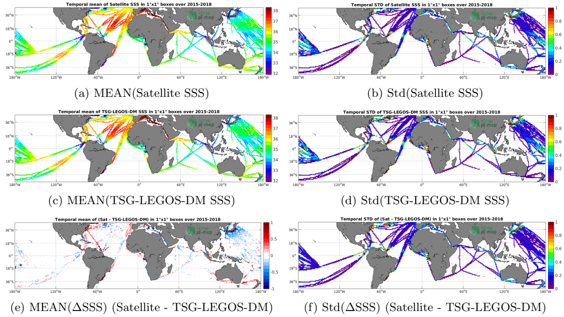
Figure 6: Temporal mean (left) and Std (right) of SSS from SMAP-L3-RSS-V4-MONTHLY (top), TSG-LEGOS-DM (middle), and of \Delta SSS (Satellite - TSG-LEGOS-DM). Only match-up pairs are used to generate these maps.
