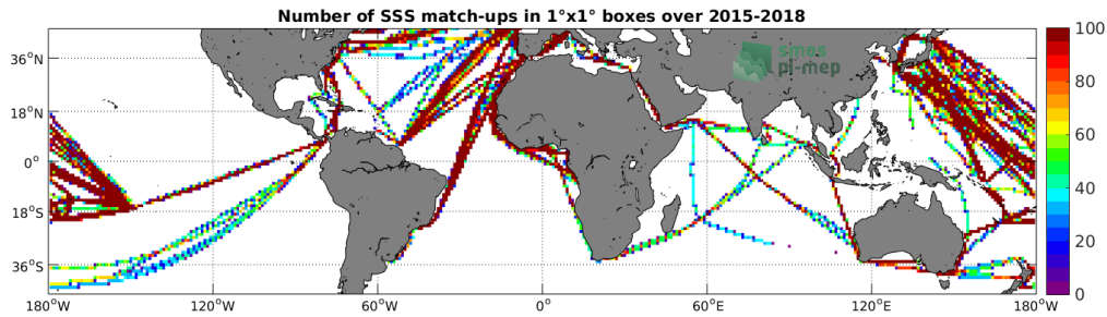
Figure 4: Number of SSS match-ups between TSG-LEGOS-DM SSS and the SMAP-L3-RSS-V4-MONTHLY SSS product for the Mid-Low Latitudes 45N-45S Pi-MEP region over 1°x1° boxes and for the full satellite product period.
