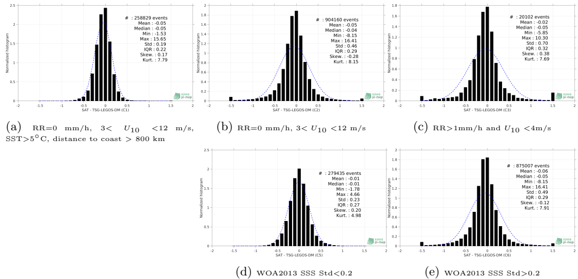
Figure 13: Normalized histogram of \Delta SSS (SMAP-L3-RSS-V4-MONTHLY - TSG-LEGOS-DM) for 5 different subdatasets corresponding to: RR=0 mm/h, 3 < U_{10} < 12 m/s, SST > 5^\circ\text{C} , distance to coast > 800 km (a), RR=0 mm/h, 3 < U_{10} < 12 m/s (b), RR > 1 mm/h and U_{10} < 4 m/s (c), WOA2013 SSS Std < 0.2 (d), WOA2013 SSS Std > 0.2 (e).
