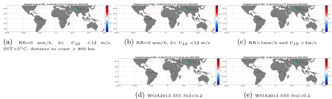
Figure 12: Temporal mean gridded over spatial boxes of size 1^\circ \times 1^\circ of \Delta\text{SSS} (SMAP SSS L3 v4 - Monthly (RSS) - TSG (GOSUD-Sailing-ship)) for 5 different subdatasets corresponding to:RR=0 mm/h, 3 < U_{10} < 12 m/s, SST>5°C, distance to coast > 800 km (a), RR=0 mm/h, 3 < U_{10} < 12 m/s (b), RR>1mm/h and U_{10} < 4 m/s (c), WOA2013 SSS Std<0.2 (d), WOA2013 SSS Std>0.2 (e).
