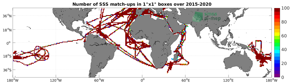
Figure 4: Number of SSS match-ups between TSG (GOSUD-Research-vessel) SSS and the SMAP SSS L3 v4 - Monthly (RSS) SSS product for the Mid-Low Latitudes 45N-45S Pi-MEP region over 1^\circ \times 1^\circ boxes and for the full satellite product period.
