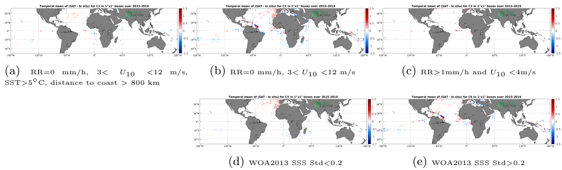
Figure 12: Temporal mean gridded over spatial boxes of size 1°x1° of \Delta SSS (SMAP SSS L3 v4 - Monthly (RSS) - TSG (GOSUD-Research-vessel)) for 5 different subdatasets corresponding to:RR=0 mm/h, 3 < U_{10} < 12 m/s, SST > 5°C, distance to coast > 800 km (a), RR=0 mm/h, 3 < U_{10} < 12 m/s (b), RR > 1mm/h and U_{10} < 4 m/s (c), WOA2013 SSS Std < 0.2 (d), WOA2013 SSS Std > 0.2 (e).
