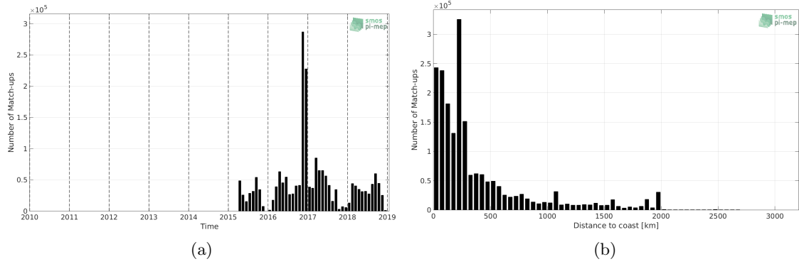
Figure 1: Number of match-ups between TSG-GOSUD-Research-vessel and SMAP-L3-RSS-V4-MONTHLY SSS as a function of time (a) and as function of the distance to coast (b) over the Mid-Low Latitudes 45N-45S Pi-MEP region and for the full satellite product period.
