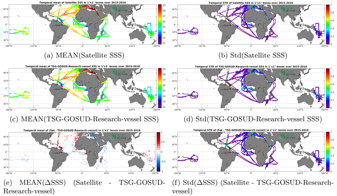
Figure 6: Temporal mean (left) and Std (right) of SSS from SMAP-L3-RSS-V4-MONTHLY (top), TSG-GOSUD-Research-vessel (middle), and of \Delta SSS (Satellite - TSG-GOSUD-Research-vessel). Only match-up pairs are used to generate these maps.
