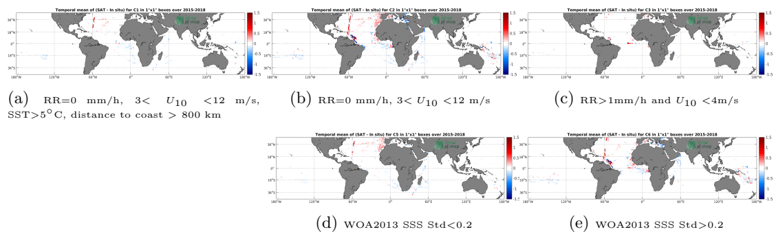
Figure 12: Temporal mean gridded over spatial boxes of size 1^\circ \times 1^\circ of \Delta SSS (SMAP-L3-RSS-V4-MONTHLY - TSG-GOSUD-Research-vessel) for 5 different subdatasets corresponding to: RR=0 mm/h, 3 < U_{10} < 12 m/s, SST > 5°C, distance to coast > 800 km (a), RR=0 mm/h, 3 < U_{10} < 12 m/s (b), RR > 1mm/h and U_{10} < 4 m/s (c), WOA2013 SSS Std < 0.2 (d), WOA2013 SSS Std > 0.2 (e).
