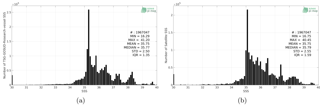
Figure 2: Histograms of SSS from TSG-GOSUD-Research-vessel (a) and SMAP-L3-RSS-V4-MONTHLY (b) considering all match-up pairs per bins of 0.1 over the Mid-Low Latitudes 45N-45S Pi-MEP region and for the full satellite product period.
