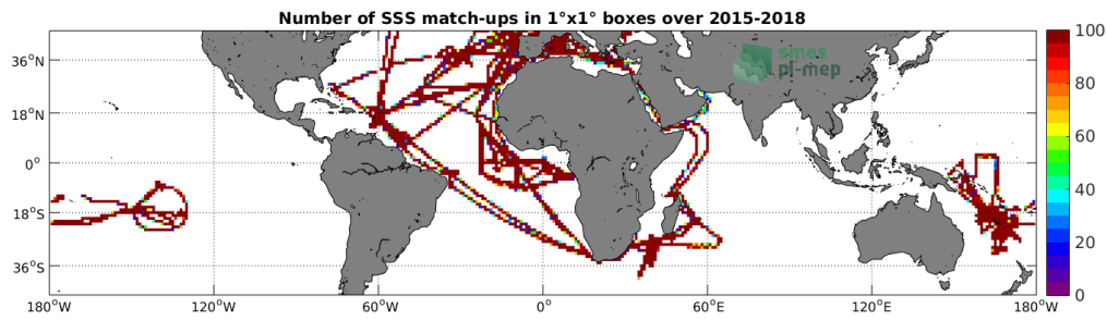
Figure 4: Number of SSS match-ups between TSG-GOSUD-Research-vessel SSS and the SMAP-L3-RSS-V4-MONTHLY SSS product for the Mid-Low Latitudes 45N-45S Pi-MEP region over 1^\circ \times 1^\circ boxes and for the full satellite product period.
