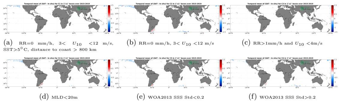
Figure 12: Temporal mean gridded over spatial boxes of size 1^\circ \times 1^\circ of \Delta SSS (SMAP SSS L3 v4 - Monthly (RSS) - Marine mammals) for 6 different subdatasets corresponding to:RR=0 mm/h, 3 < U_{10} < 12 m/s, SST >5^\circ\text{C} , distance to coast > 800 km (a), RR=0 mm/h, 3 < U_{10} < 12 m/s (b), RR >1 mm/h and U_{10} < 4 m/s (c),MLD <20 m (d),WOA2013 SSS Std <0.2 (e),WOA2013 SSS Std >0.2 (f).
