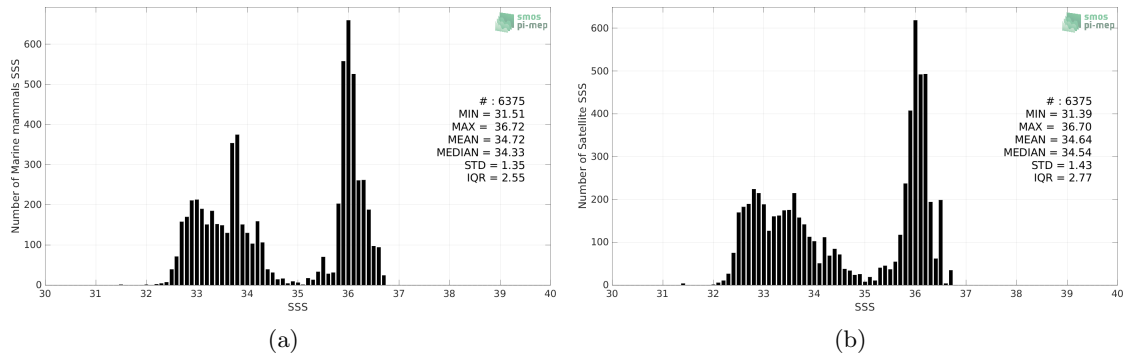
Figure 2: Histograms of SSS from Marine mammals (a) and SMAP SSS L3 v4 - Monthly (RSS) (b) considering all match-up pairs per bins of 0.1 over the Mid-Low Latitudes 45N-45S Pi-MEP region and for the full satellite product period.
