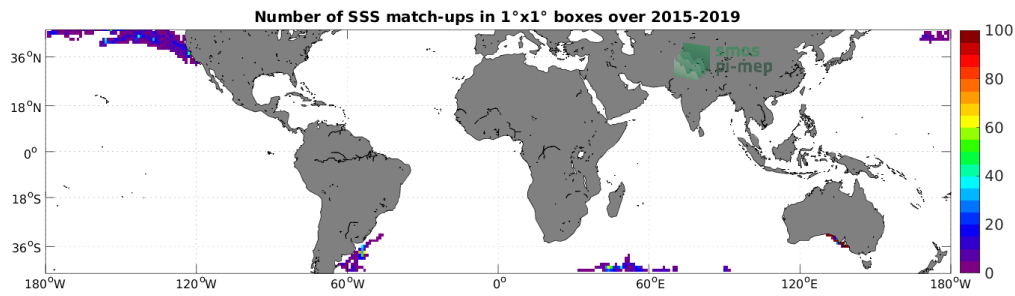
Figure 4: Number of SSS match-ups between Marine mammals SSS and the SMAP SSS L3 v4 - Monthly (RSS) SSS product for the Mid-Low Latitudes 45N-45S Pi-MEP region over 1^\circ \times 1^\circ boxes and for the full satellite product period.
