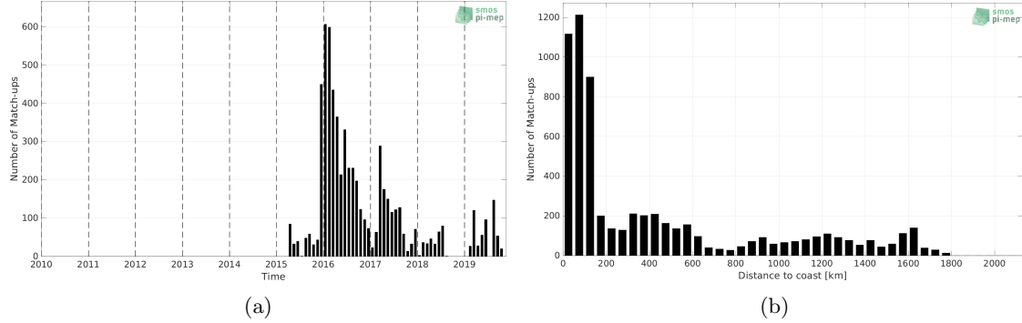
Figure 1: Number of match-ups between Marine mammals and SMAP SSS L3 v4 - Monthly (RSS) SSS as a function of time (a) and as function of the distance to coast (b) over the Mid-Low Latitudes 45N-45S Pi-MEP region and for the full satellite product period.
