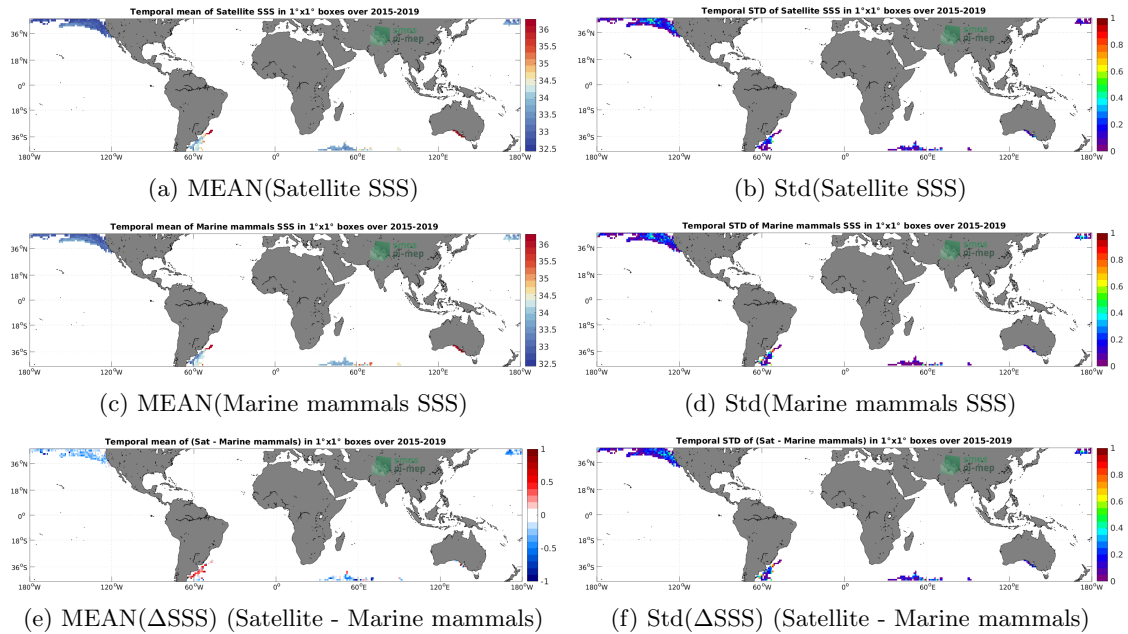
Figure 6: Temporal mean (left) and Std (right) of SSS from SMAP SSS L3 v4 - Monthly (RSS) (top), Marine mammals (middle), and of \Delta SSS (Satellite - Marine mammals). Only match-up pairs are used to generate these maps.
