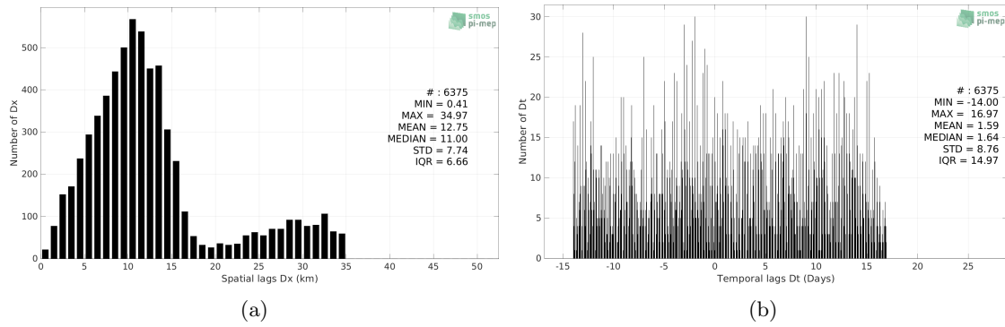
Figure 5: Histograms of the spatial (a) and temporal (b) lags between the location/time of the Marine mammals measurement and the date of the corresponding SMAP SSS L3 v4 - Monthly (RSS) SSS pixel.
