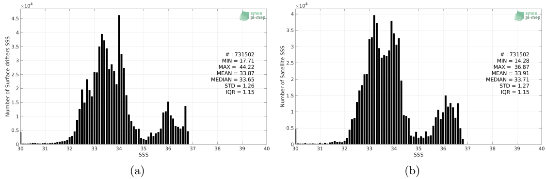
Figure 2: Histograms of SSS from Surface drifters (a) and SMAP SSS L3 v4 - Monthly (RSS) (b) considering all match-up pairs per bins of 0.1 over the Mid-Low Latitudes 45N-45S Pi-MEP region and for the full satellite product period.
