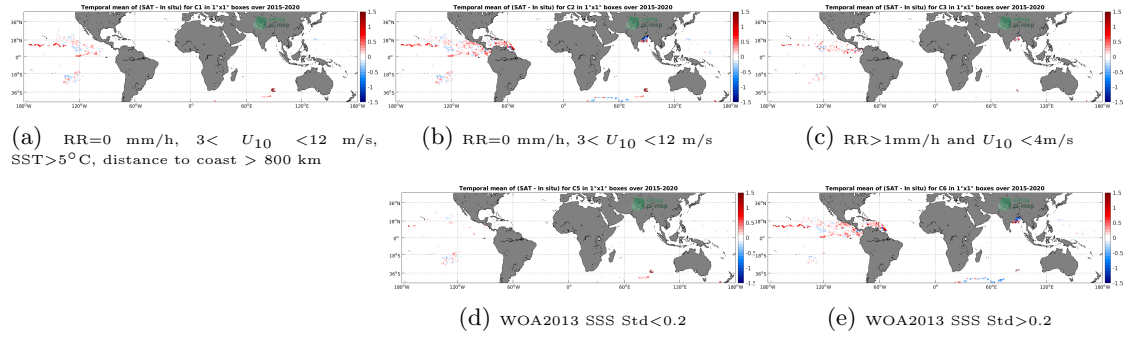
Figure 11: Temporal mean gridded over spatial boxes of size 1^\circ \times 1^\circ of \Delta SSS (SMAP SSS L3 v4 - Monthly (RSS) - Surface drifters) for 5 different subdatasets corresponding to: RR=0 mm/h, 3 < U_{10} < 12 m/s, SST > 5^\circ C , distance to coast > 800 km (a), RR=0 mm/h, 3 < U_{10} < 12 m/s (b), RR > 1 mm/h and U_{10} < 4 m/s (c), WOA2013 SSS Std < 0.2 (d), WOA2013 SSS Std > 0.2 (e).
