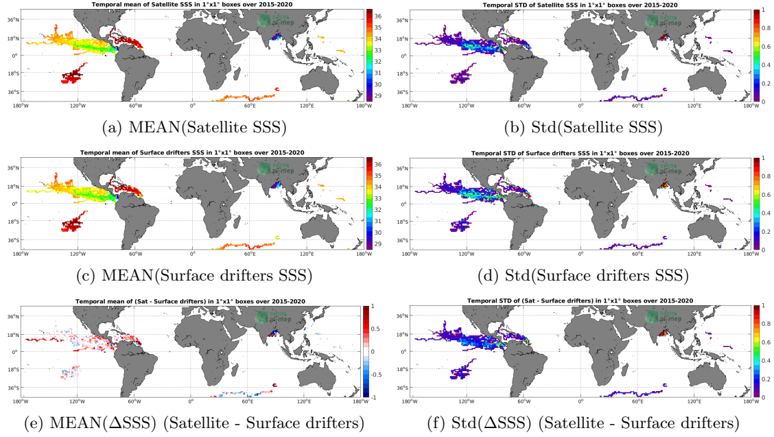
Figure 5: Temporal mean (left) and Std (right) of SSS from SMAP SSS L3 v4 - Monthly (RSS) (top), Surface drifters (middle), and of \Delta SSS (Satellite - Surface drifters). Only match-up pairs are used to generate these maps.
