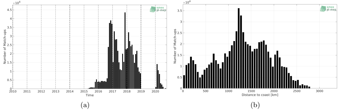
Figure 1: Number of match-ups between Surface drifters and SMAP SSS L3 v4 - Monthly (RSS) SSS as a function of time (a) and as function of the distance to coast (b) over the Mid-Low Latitudes 45N-45S Pi-MEP region and for the full satellite product period.
