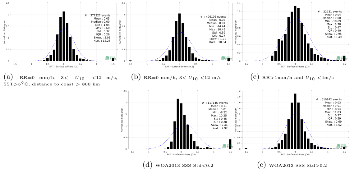
Figure 12: Normalized histogram of \Delta SSS (SMAP SSS L3 v4 - Monthly (RSS) - Surface drifters) for 5 different subdatasets corresponding to: RR=0 mm/h, 3 < U_{10} < 12 m/s, SST > 5^\circ C , distance to coast > 800 km (a), RR=0 mm/h, 3 < U_{10} < 12 m/s (b), RR > 1 mm/h and U_{10} < 4 m/s (c), WOA2013 SSS Std < 0.2 (d), WOA2013 SSS Std > 0.2 (e).
