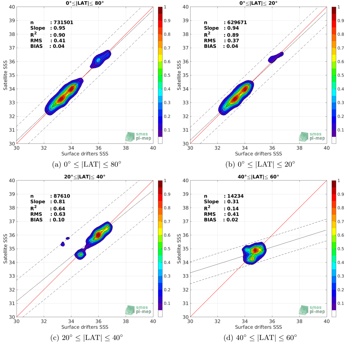
Figure 8: Contour maps of the concentration of SMAP SSS L3 v4 - Monthly (RSS) SSS (y-axis) versus Surface drifters SSS (x-axis) at match-up pairs for different latitude bands. For each plot, the red line shows x=y . The black thin and dashed lines indicate a linear fit through the data cloud and the \pm 95\% confidence levels, respectively. The number match-up pairs n , the slope and R^2 coefficient of the linear fit, the root mean square (RMS) and the mean bias between satellite and in situ data are indicated for each latitude band in each plots.
