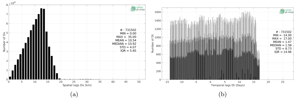
Figure 4: Histograms of the spatial (a) and temporal (b) lags between the location/time of the Surface drifters measurement and the date of the corresponding SMAP SSS L3 v4 - Monthly (RSS) SSS pixel.
