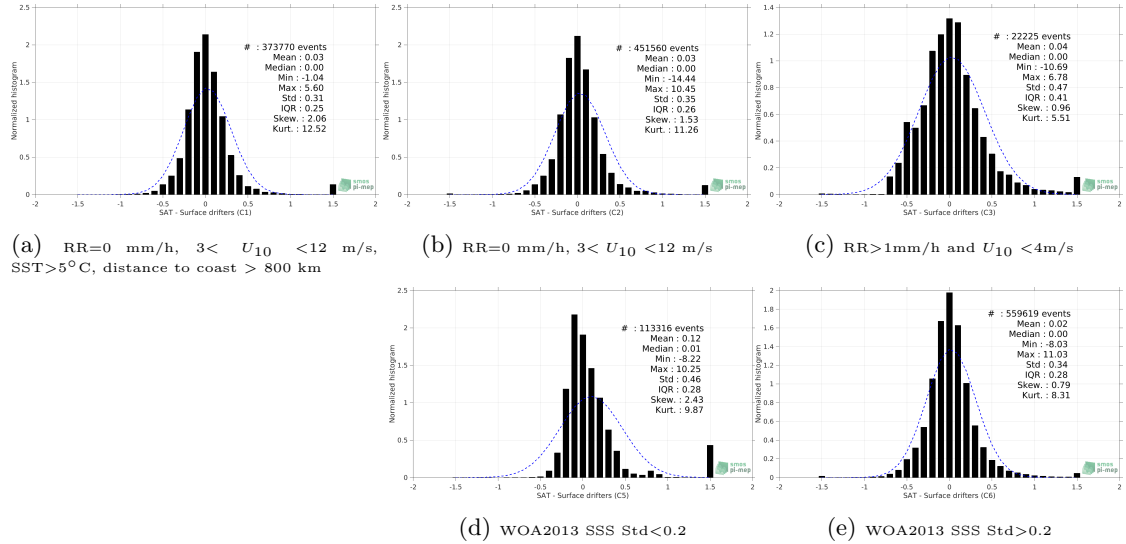
Figure 12: Normalized histogram of \Delta SSS (SMAP SSS L3 v4 - Monthly (RSS) - Surface drifters) for 5 different subdatasets corresponding to: RR=0 mm/h, 3 < U_{10} < 12 m/s, SST>5°C, distance to coast > 800 km (a), RR=0 mm/h, 3 < U_{10} < 12 m/s (b), RR>1mm/h and U_{10} < 4 m/s (c), WOA2013 SSS Std<0.2 (d), WOA2013 SSS Std>0.2 (e).
