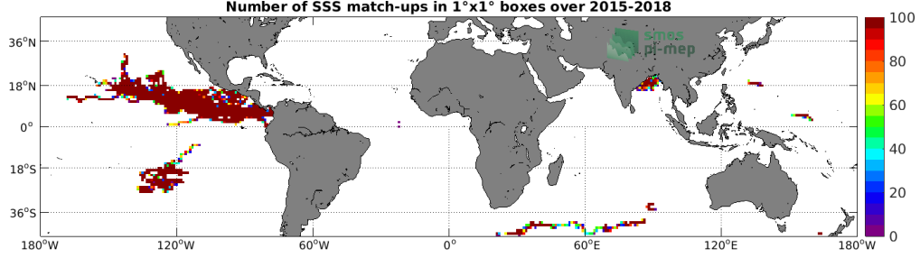
Figure 3: Number of SSS match-ups between Surface drifters SSS and the SMAP SSS L3 v4 - Monthly (RSS) SSS product for the Mid-Low Latitudes 45N-45S Pi-MEP region over 1°x1° boxes and for the full satellite product period.
