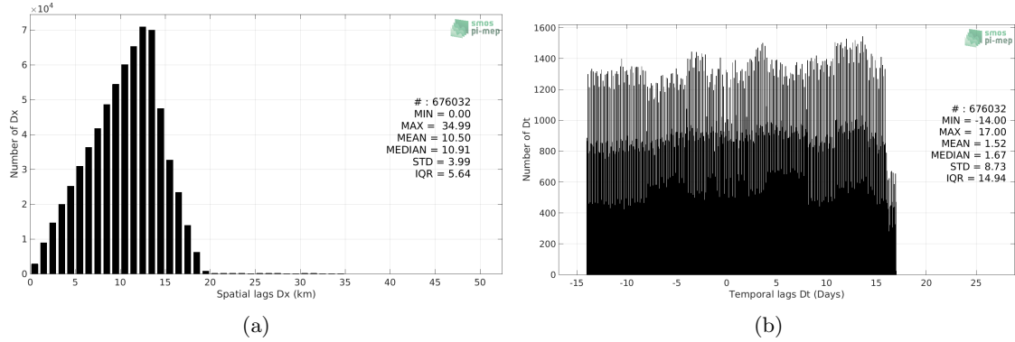
Figure 4: Histograms of the spatial (a) and temporal (b) lags between the time of the Surface drifters measurements and the date of the corresponding SMAP SSS L3 v4 - Monthly (RSS) SSS product.
