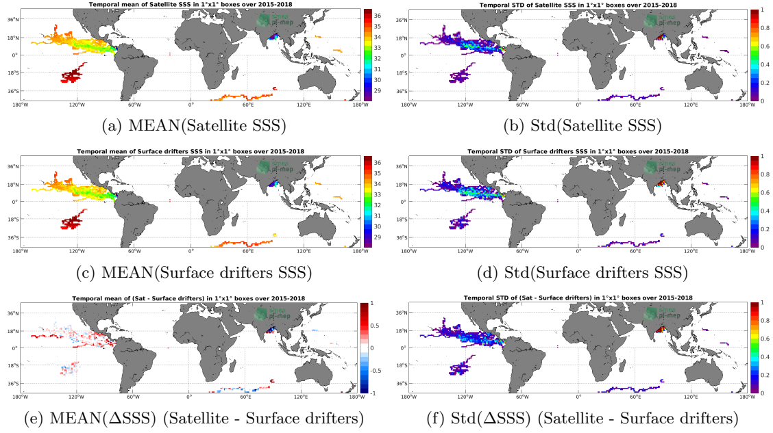
Figure 5: Temporal mean (left) and Std (right) of SSS from SMAP SSS L3 v4 - Monthly (RSS) (top), Surface drifters (middle), and of \Delta SSS (Satellite - Surface drifters). Only match-up pairs are used to generate these maps.
