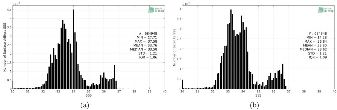
Figure 2: Histograms of SSS from Surface drifters (a) and SMAP-L3-RSS-V4-MONTHLY (b) considering all match-up pairs per bins of 0.1 over the Mid-Low Latitudes 45N-45S Pi-MEP region and for the full satellite product period.
