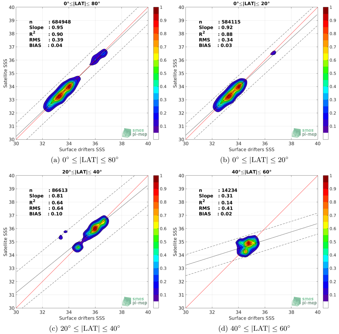
Figure 8: Contour maps of the concentration of SMAP-L3-RSS-V4-MONTHLY SSS (y-axis) versus Surface drifters SSS (x-axis) at match-up pairs for different latitude bands. For each plot, the red line shows x=y . The black thin and dashed lines indicate a linear fit through the data cloud and the \pm 95\% confidence levels, respectively. The number match-up pairs n , the slope and R^2 coefficient of the linear fit, the root mean square (RMS) and the mean bias between satellite and in situ data are indicated for each latitude band in each plots.
