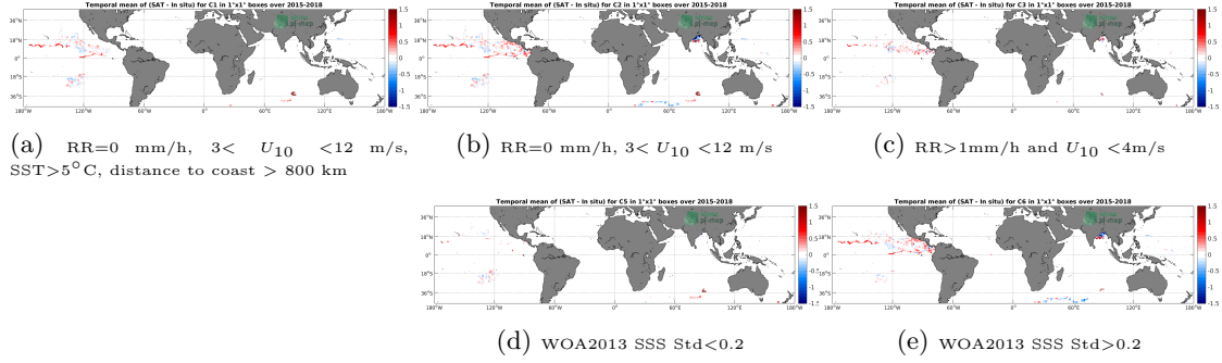
Figure 11: Temporal mean gridded over spatial boxes of size 1^\circ \times 1^\circ of \Delta SSS (SMAP-L3-RSS-V4-MONTHLY - Surface drifters) for 5 different subdatasets corresponding to: RR=0 mm/h, 3 < U_{10} < 12 m/s, SST > 5^\circ C , distance to coast > 800 km (a), RR=0 mm/h, 3 < U_{10} < 12 m/s (b), RR > 1 mm/h and U_{10} < 4 m/s (c), WOA2013 SSS Std < 0.2 (d), WOA2013 SSS Std > 0.2 (e).
