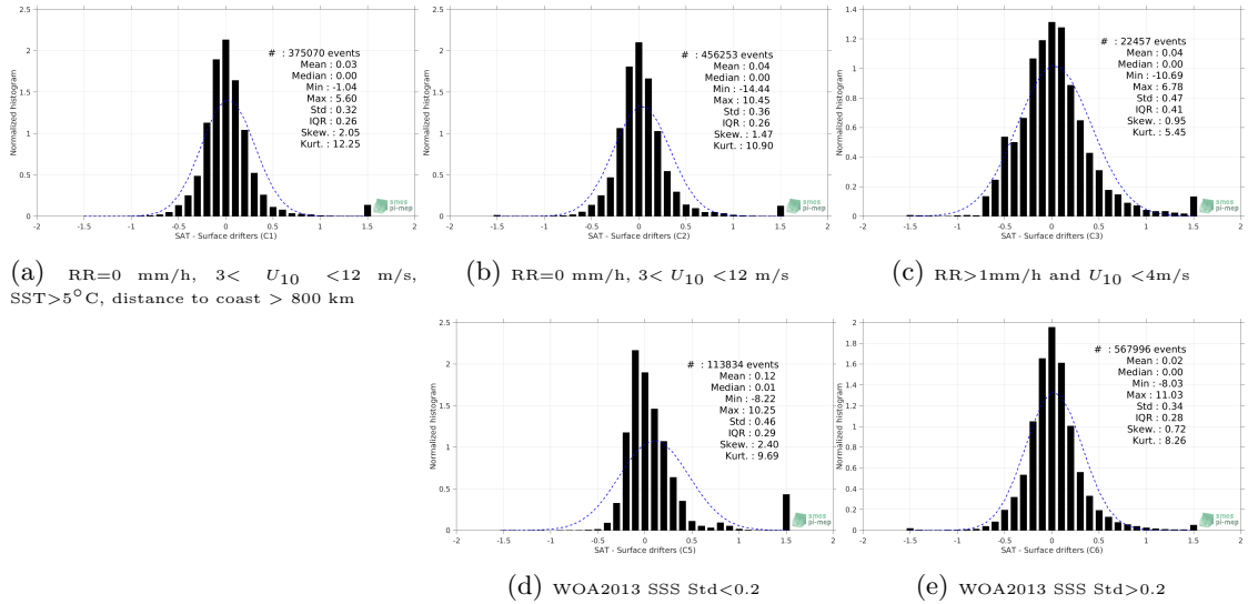
Figure 12: Normalized histogram of \Delta SSS (SMAP-L3-RSS-V4-MONTHLY - Surface drifters) for 5 different subdatasets corresponding to: RR=0 mm/h, 3 < U_{10} < 12 m/s, SST > 5^\circ C , distance to coast > 800 km (a), RR=0 mm/h, 3 < U_{10} < 12 m/s (b), RR > 1 mm/h and U_{10} < 4 m/s (c), WOA2013 SSS Std < 0.2 (d), WOA2013 SSS Std > 0.2 (e).
