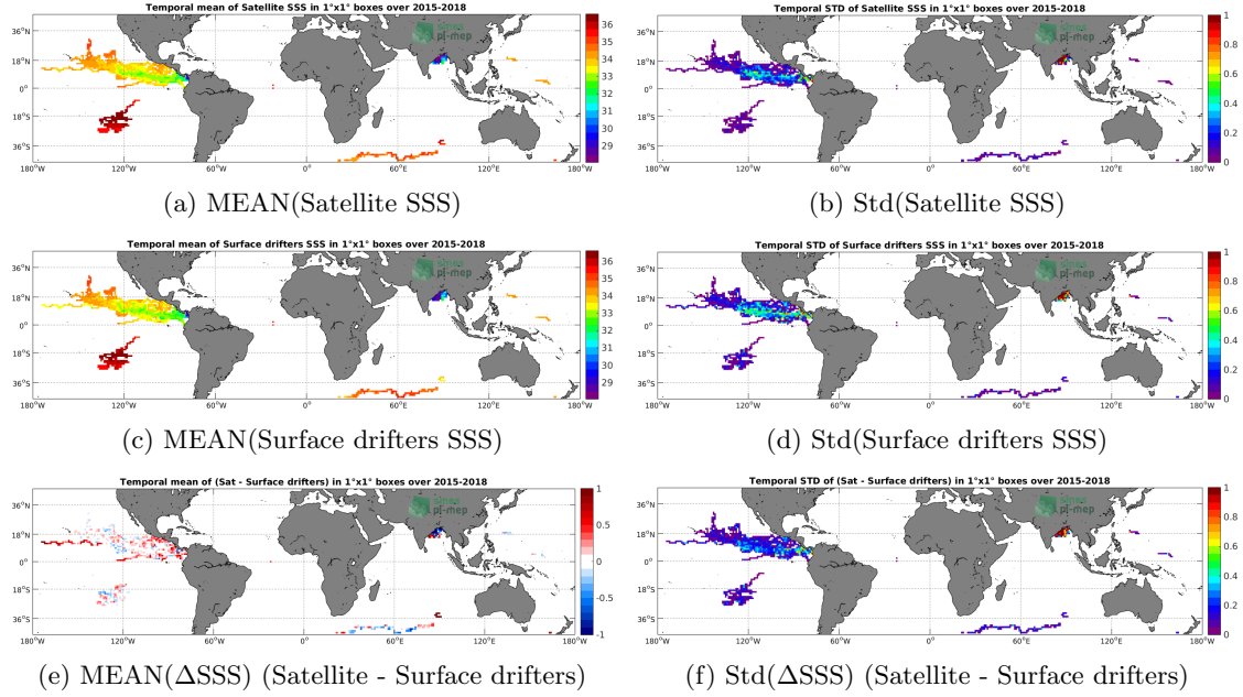
Figure 5: Temporal mean (left) and Std (right) of SSS from SMAP-L3-RSS-V4-MONTHLY (top), Surface drifters (middle), and of \Delta SSS (Satellite - Surface drifters). Only match-up pairs are used to generate these maps.
