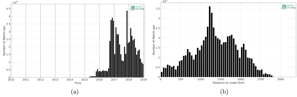
Figure 1: Number of match-ups between Surface drifters and SMAP-L3-RSS-V4-MONTHLY SSS as a function of time (a) and as function of the distance to coast (b) over the Mid-Low Latitudes 45N-45S Pi-MEP region and for the full satellite product period.
