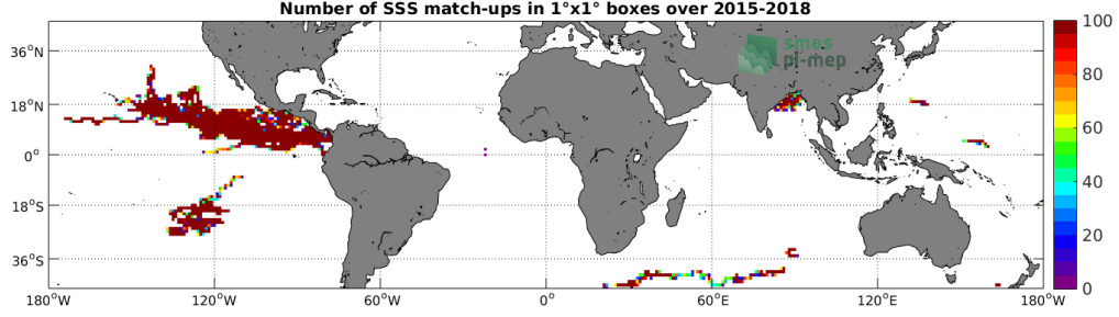
Figure 3: Number of SSS match-ups between Surface drifters SSS and the SMAP-L3-RSS-V4-MONTHLY SSS product for the Mid-Low Latitudes 45N-45S Pi-MEP region over 1^\circ \times 1^\circ boxes and for the full satellite product period.
