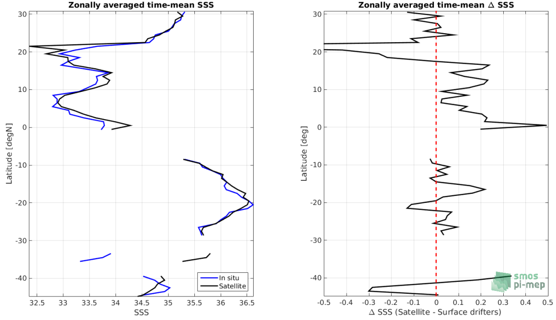
Figure 7: Left panel: Zonal mean SSS from SMAP-L3-RSS-V4-MONTHLY satellite product (black) and from Surface drifters (blue). Right panel: Zonal mean of \Delta SSS (Satellite - Surface drifters) for all the collected Pi-MEP match-up pairs estimated over the full satellite product period.
