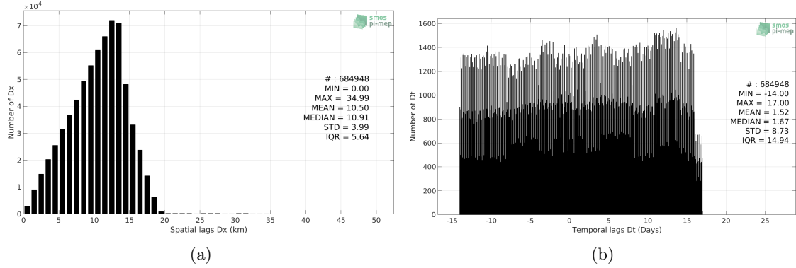
Figure 4: Histograms of the spatial (a) and temporal (b) lags between the time of the Surface drifters measurements and the date of the corresponding SMAP-L3-RSS-V4-MONTHLY SSS product.
