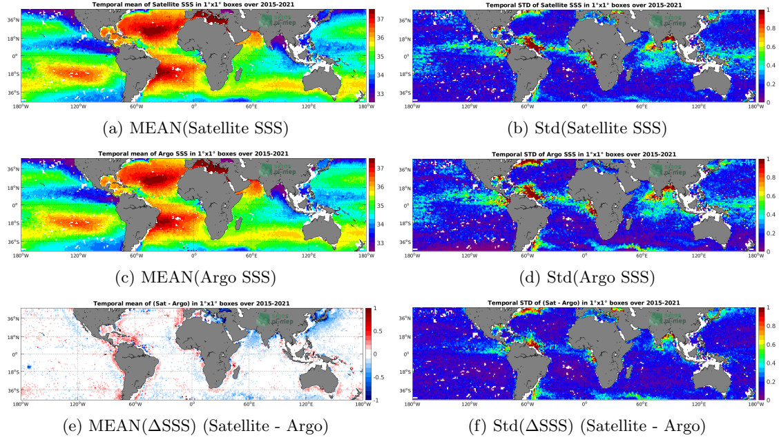
Figure 6: Temporal mean (left) and Std (right) of SSS from SMAP SSS L3 v4 - Monthly (RSS) (top), Argo (middle), and of \Delta SSS (Satellite - Argo). Only match-up pairs are used to generate these maps.
