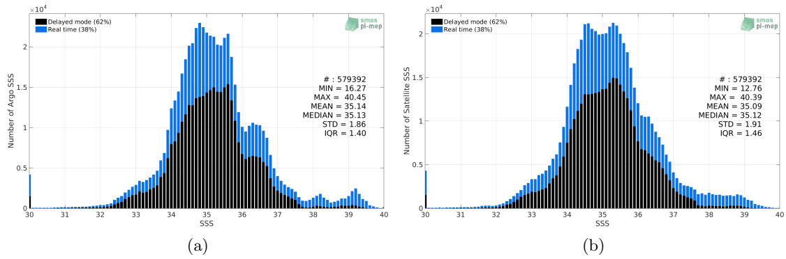
Figure 2: Histograms of SSS from Argo (a) and SMAP SSS L3 v4 - Monthly (RSS) (b) considering all match-up pairs per bins of 0.1 over the Mid-Low Latitudes 45N-45S Pi-MEP region and for the full satellite product period.
