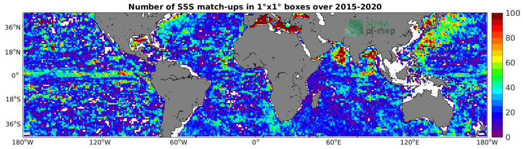
Figure 4: Number of SSS match-ups between Argo SSS and the SMAP SSS L3 v4 - Monthly (RSS) SSS product for the Mid-Low Latitudes 45N-45S Pi-MEP region over 1^\circ \times 1^\circ boxes and for the full satellite product period.
