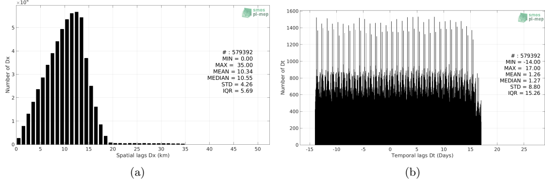
Figure 5: Histograms of the spatial (a) and temporal (b) lags between the time of the Argo measurements and the date of the corresponding SMAP SSS L3 v4 - Monthly (RSS) SSS product.
