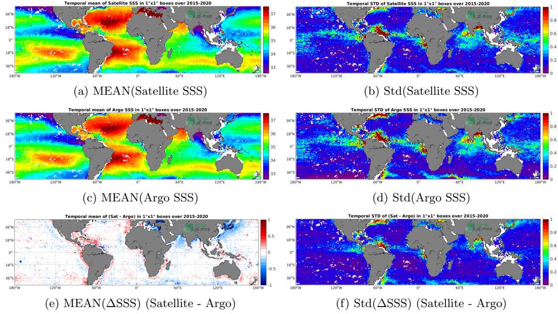
Figure 6: Temporal mean (left) and Std (right) of SSS from SMAP SSS L3 v4 - Monthly (RSS) (top), Argo (middle), and of \Delta SSS (Satellite - Argo). Only match-up pairs are used to generate these maps.
