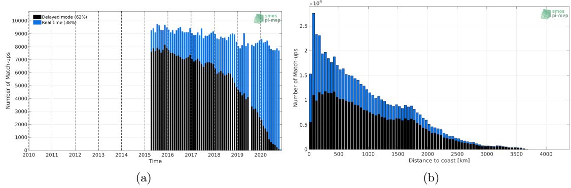
Figure 1: Number of match-ups between Argo and SMAP SSS L3 v4 - Monthly (RSS) SSS as a function of time (a) and as function of the distance to coast (b) over the Mid-Low Latitudes 45N-45S Pi-MEP region and for the full satellite product period.
