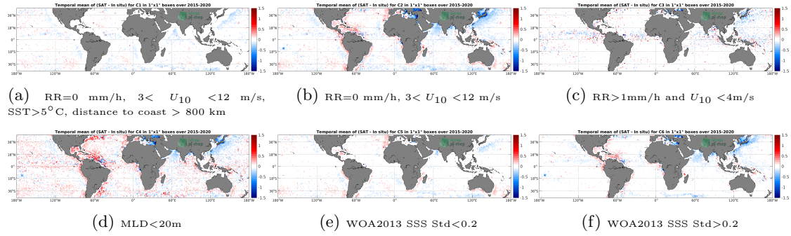
Figure 12: Temporal mean gridded over spatial boxes of size 1^\circ \times 1^\circ of \Delta SSS (SMAP SSS L3 v4 - Monthly (RSS) - Argo) for 6 different subdatasets corresponding to: RR=0 mm/h, 3 < U_{10} < 12 m/s, SST > 5^\circ C , distance to coast > 800 km (a), RR=0 mm/h, 3 < U_{10} < 12 m/s (b), RR > 1 mm/h and U_{10} < 4 m/s (c), MLD < 20 m (d), WOA2013 SSS Std < 0.2 (e), WOA2013 SSS Std > 0.2 (f).
