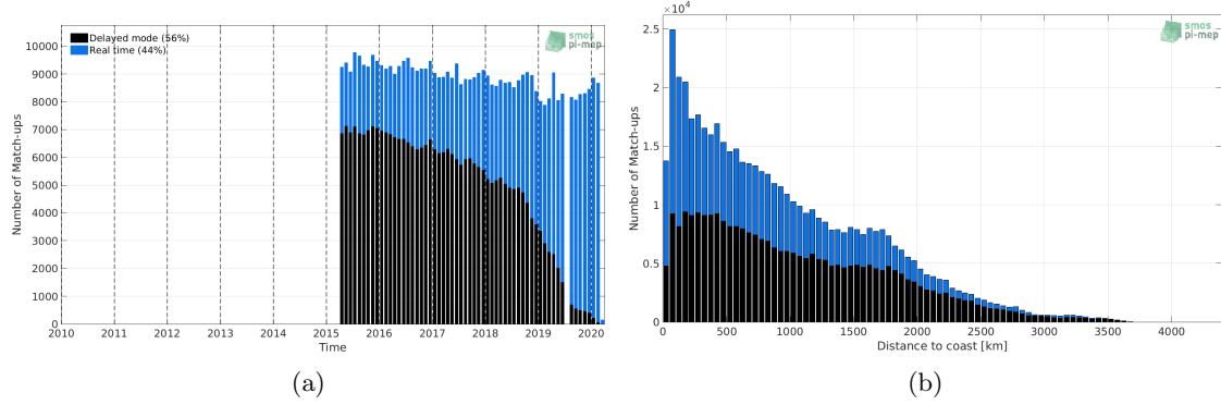
Figure 1: Number of match-ups between Argo and SMAP-L3-RSS-V4-MONTHLY SSS as a function of time (a) and as function of the distance to coast (b) over the Mid-Low Latitudes 45N-45S Pi-MEP region and for the full satellite product period.
