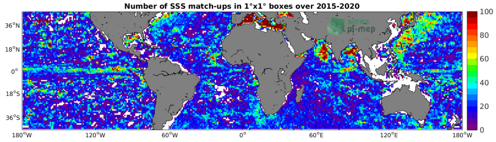
Figure 4: Number of SSS match-ups between Argo SSS and the SMAP-L3-RSS-V4-MONTHLY SSS product for the Mid-Low Latitudes 45N-45S Pi-MEP region over 1^\circ \times 1^\circ boxes and for the full satellite product period.
