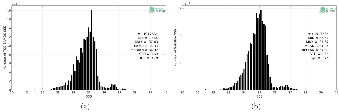
Figure 2: Histograms of SSS from TSG-SAMOS (a) and SMAP-L3-RSS-V3-8DAY-RUNNING-70KM (b) considering all match-up pairs per bins of 0.1 over the Mid-Low Latitudes 45N-45S Pi-MEP region and for the full satellite product period.
