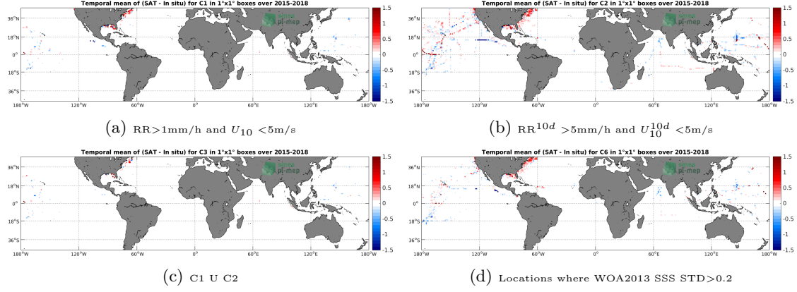
Figure 12: Temporal mean gridded over spatial boxes of size 1^\circ \times 1^\circ of \Delta SSS (SMAP-L3-RSS-V3-8DAY-RUNNING-70KM - TSG-SAMOS) for 4 different subdatasets corresponding to: RR > 1\text{mm/h} and U_{10} < 5\text{m/s} (a), RR^{10d} > 5\text{mm/h} and U_{10}^{10d} < 5\text{m/s} (b), C1 U C2 (c), Locations where WOA2013 SSS STD > 0.2 (d).
