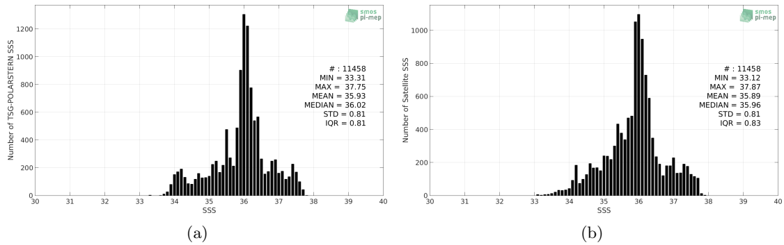
Figure 2: Histograms of SSS from TSG-POLARSTERN (a) and SMAP-L3-RSS-V3-8DAY-RUNNING-70KM (b) considering all match-up pairs per bins of 0.1 over the Mid-Low Latitudes 45N-45S Pi-MEP region and for the full satellite product period.
