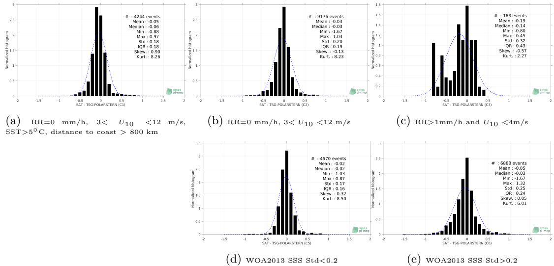
Figure 13: Normalized histogram of \Delta SSS (SMAP-L3-RSS-V3-8DAY-RUNNING-70KM - TSG-POLARSTERN) for 5 different subdatasets corresponding to: RR=0 mm/h, 3 < U_{10} < 12 m/s, SST >5^\circ\text{C} , distance to coast > 800 km (a), RR=0 mm/h, 3 < U_{10} < 12 m/s (b), RR >1 mm/h and U_{10} < 4 m/s (c), WOA2013 SSS Std <0.2 (d), WOA2013 SSS Std >0.2 (e).
