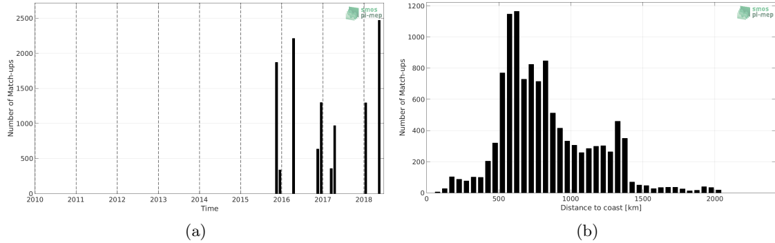
Figure 1: Number of match-ups between TSG-POLARSTERN and SMAP-L3-RSS-V3-8DAY-RUNNING-70KM SSS as a function of time (a) and as function of the distance to coast (b) over the Mid-Low Latitudes 45N-45S Pi-MEP region and for the full satellite product period.
