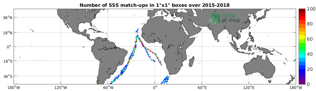
Figure 4: Number of SSS match-ups between TSG-POLARSTERN SSS and the SMAP-L3-RSS-V3-8DAY-RUNNING-70KM SSS product for the Mid-Low Latitudes 45N-45S Pi-MEP region over 1^\circ \times 1^\circ boxes and for the full satellite product period.
