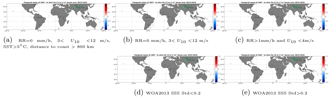
Figure 12: Temporal mean gridded over spatial boxes of size 1^\circ \times 1^\circ of \Delta SSS (SMAP-L3-RSS-V3-8DAY-RUNNING-70KM - TSG-POLARSTERN) for 5 different subdatasets corresponding to: RR=0 mm/h, 3 < U_{10} < 12 m/s, SST >5^\circ\text{C} , distance to coast > 800 km (a), RR=0 mm/h, 3 < U_{10} < 12 m/s (b), RR >1 mm/h and U_{10} < 4 m/s (c), WOA2013 SSS Std <0.2 (d), WOA2013 SSS Std >0.2 (e).
