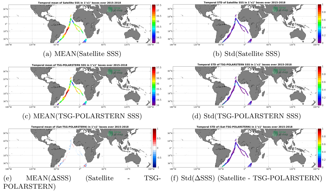
Figure 6: Temporal mean (left) and Std (right) of SSS from SMAP-L3-RSS-V3-8DAY-RUNNING-70KM (top), TSG-POLARSTERN (middle), and of \Delta SSS (Satellite - TSG-POLARSTERN). Only match-up pairs are used to generate these maps.
