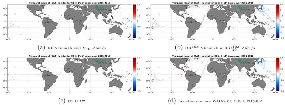
Figure 12: Temporal mean gridded over spatial boxes of size 1^\circ \times 1^\circ of \Delta SSS (SMAP-L3-RSS-V3-8DAY-RUNNING-70KM - TSG-LEGOS-DM) for 4 different subdatasets corresponding to: RR > 1\text{mm/h} and U_{10} < 5\text{m/s} (a), RR^{10d} > 5\text{mm/h} and U_{10}^{10d} < 5\text{m/s} (b), C1 U C2 (c), Locations where WOA2013 SSS STD > 0.2 (d).
