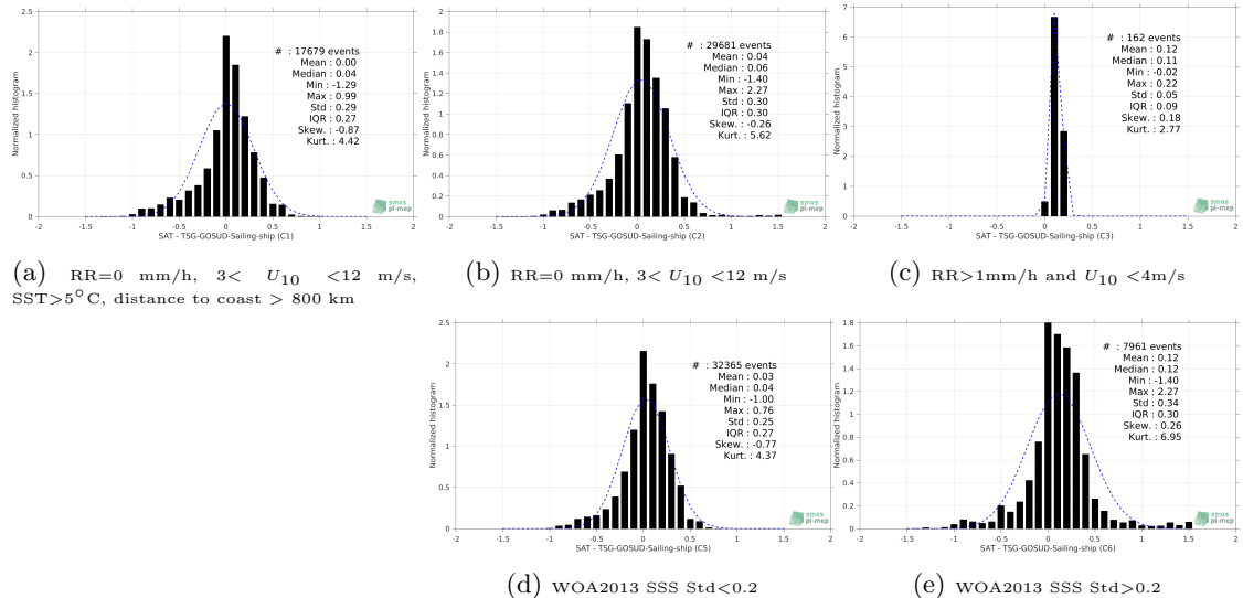
Figure 13: Normalized histogram of \Delta SSS (SMAP-L3-RSS-V3-8DAY-RUNNING-70KM - TSG-GOSUD-Sailing-ship) for 5 different subdatasets corresponding to: RR=0 mm/h, 3 < U_{10} < 12 m/s, SST >5^\circ C, distance to coast > 800 km (a), RR=0 mm/h, 3 < U_{10} < 12 m/s (b), RR >1 mm/h and U_{10} < 4 m/s (c), WOA2013 SSS Std <0.2 (d), WOA2013 SSS Std >0.2 (e).
