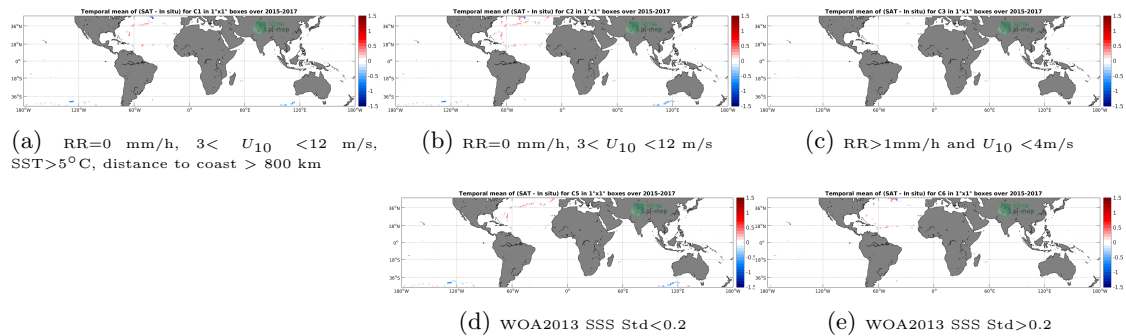
Figure 12: Temporal mean gridded over spatial boxes of size 1^\circ \times 1^\circ of \Delta SSS (SMAP-L3-RSS-V3-8DAY-RUNNING-70KM - TSG-GOSUD-Sailing-ship) for 5 different subdatasets corresponding to: RR=0 mm/h, 3 < U_{10} < 12 m/s, SST >5^\circ C, distance to coast > 800 km (a), RR=0 mm/h, 3 < U_{10} < 12 m/s (b), RR >1 mm/h and U_{10} < 4 m/s (c), WOA2013 SSS Std <0.2 (d), WOA2013 SSS Std >0.2 (e).
