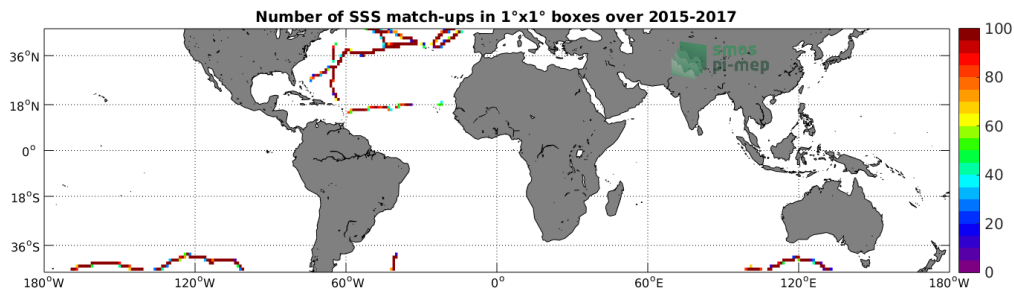
Figure 4: Number of SSS match-ups between TSG-GOSUD-Sailing-ship SSS and the SMAP-L3-RSS-V3-8DAY-RUNNING-70KM SSS product for the Mid-Low Latitudes 45N-45S Pi-MEP region over 1^\circ \times 1^\circ boxes and for the full satellite product period.
