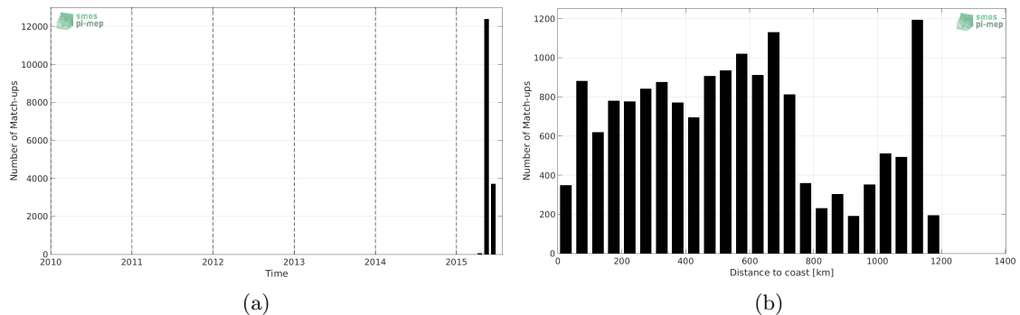
Figure 1: Number of match-ups between TSG-GOSUD-Sailing-ship and SMAP-L3-RSS-V3-8DAY-RUNNING-70KM SSS as a function of time (a) and as function of the distance to coast (b) over the Mid-Low Latitudes 45N-45S Pi-MEP region and for the full satellite product period.
