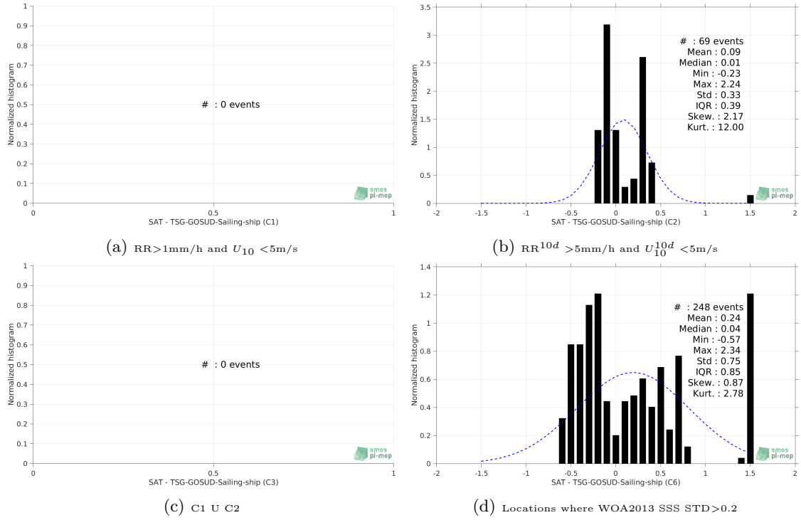
Figure 13: Normalized histogram of \Delta\text{SSS} (SMAP-L3-RSS-V3-8DAY-RUNNING-70KM - TSG-GOSUD-Sailing-ship) for 6 different subdatasets corresponding to: RR > 1\text{mm/h} and U_{10} < 5\text{m/s} (a), RR^{10d} > 5\text{mm/h} and U_{10}^{10d} < 5\text{m/s} (b), C1 \cup C2 (c), Locations where WOA2013 SSS STD > 0.2 (d).
