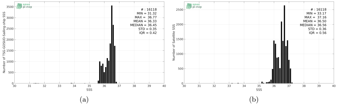
Figure 2: Histograms of SSS from TSG-GOSUD-Sailing-ship (a) and SMAP-L3-RSS-V3-8DAY-RUNNING-70KM (b) considering all match-up pairs per bins of 0.1 over the Mid-Low Latitudes 45N-45S Pi-MEP region and for the full satellite product period.
