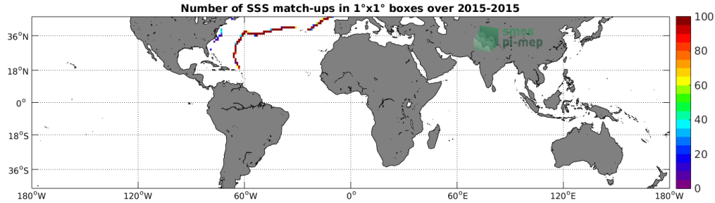
Figure 4: Number of SSS match-ups between TSG-GOSUD-Sailing-ship SSS and the SMAP-L3-RSS-V3-8DAY-RUNNING-70KM SSS product for the Mid-Low Latitudes 45N-45S Pi-MEP region over 1°x1° boxes and for the full satellite product period.
