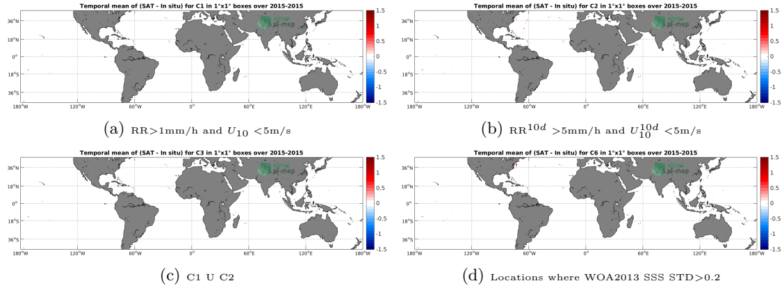
Figure 12: Temporal mean gridded over spatial boxes of size 1^\circ \times 1^\circ of \Delta SSS (SMAP-L3-RSS-V3-8DAY-RUNNING-70KM - TSG-GOSUD-Sailing-ship) for 4 different subdatasets corresponding to: RR > 1\text{mm/h} and U_{10} < 5\text{m/s} (a), RR^{10d} > 5\text{mm/h} and U_{10}^{10d} < 5\text{m/s} (b), C1 U C2 (c), Locations where WOA2013 SSS STD > 0.2 (d).
