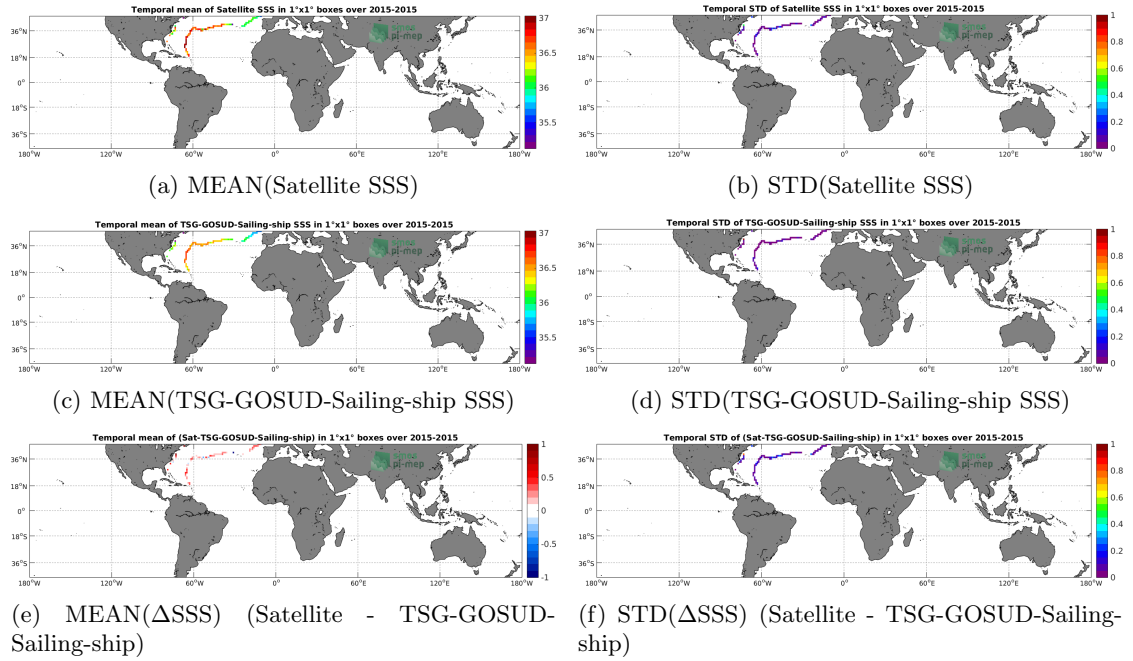
Figure 6: Temporal mean (left) and STD (right) of SSS from SMAP-L3-RSS-V3-8DAY-RUNNING-70KM (top), TSG-GOSUD-Sailing-ship (middle), and of \Delta SSS (Satellite - TSG-GOSUD-Sailing-ship). Only match-up pairs are used to generate these maps.
