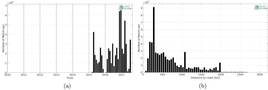
Figure 1: Number of match-ups between TSG-GOSUD-Research-vessel and SMAP-L3-RSS-V3-8DAY-RUNNING-70KM SSS as a function of time (a) and as function of the distance to coast (b) over the Mid-Low Latitudes 45N-45S Pi-MEP region and for the full satellite product period.
