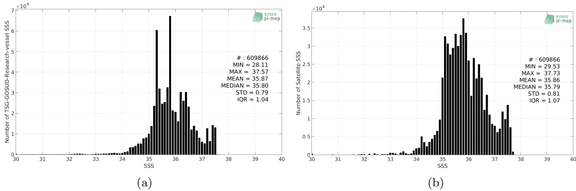
Figure 2: Histograms of SSS from TSG-GOSUD-Research-vessel (a) and SMAP-L3-RSS-V3-8DAY-RUNNING-70KM (b) considering all match-up pairs per bins of 0.1 over the Mid-Low Latitudes 45N-45S Pi-MEP region and for the full satellite product period.
