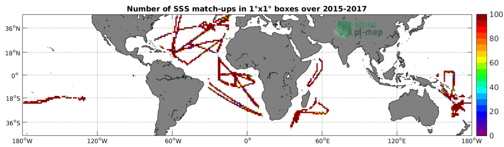
Figure 4: Number of SSS match-ups between TSG-GOSUD-Research-vessel SSS and the SMAP-L3-RSS-V3-8DAY-RUNNING-70KM SSS product for the Mid-Low Latitudes 45N-45S Pi-MEP region over 1^\circ \times 1^\circ boxes and for the full satellite product period.
