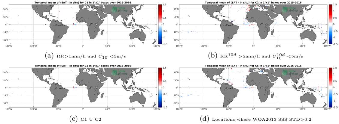
Figure 12: Temporal mean gridded over spatial boxes of size 1^\circ \times 1^\circ of \Delta SSS (SMAP-L3-RSS-V3-8DAY-RUNNING-70KM - TSG-GOSUD-Research-vessel) for 4 different subdatasets corresponding to: RR > 1\text{mm/h} and U_{10} < 5\text{m/s} (a), RR^{10d} > 5\text{mm/h} and U_{10}^{10d} < 5\text{m/s} (b), C1 U C2 (c), Locations where WOA2013 SSS STD > 0.2 (d).
