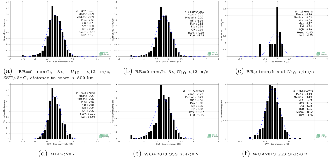
Figure 13: Normalized histogram of \Delta SSS (SMAP-L3-RSS-V3-8DAY-RUNNING-70KM - Sea mammals) for 6 different subdatasets corresponding to: RR=0 mm/h, 3 < U_{10} < 12 m/s, SST>5°C, distance to coast > 800 km (a), RR=0 mm/h, 3 < U_{10} < 12 m/s (b), RR>1mm/h and U_{10} < 4 m/s (c), MLD<20m (d), WOA2013 SSS Std<0.2 (e), WOA2013 SSS Std>0.2 (f).
