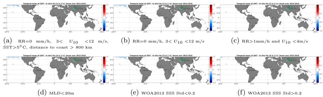
Figure 12: Temporal mean gridded over spatial boxes of size 1^\circ \times 1^\circ of \Delta SSS (SMAP-L3-RSS-V3-8DAY-RUNNING-70KM - Sea mammals) for 6 different subdatasets corresponding to:RR=0 mm/h, 3 < U_{10} < 12 m/s, SST >5^\circ C, distance to coast > 800 km (a), RR=0 mm/h, 3 < U_{10} < 12 m/s (b), RR >1 mm/h and U_{10} < 4 m/s (c),MLD <20 m (d),WOA2013 SSS Std <0.2 (e),WOA2013 SSS Std >0.2 (f).
