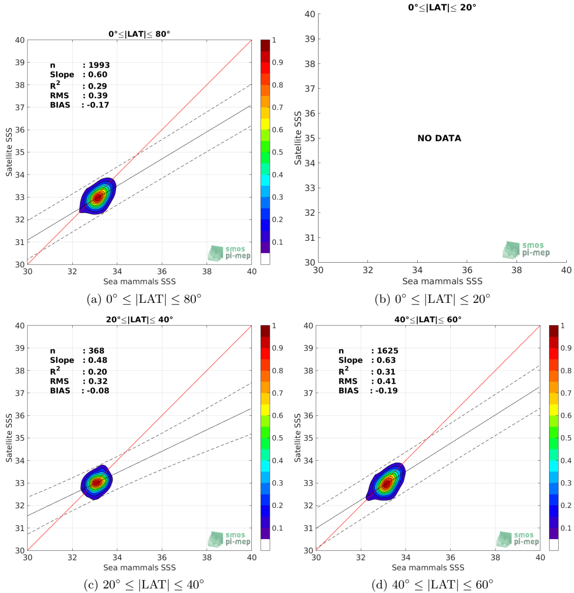
Figure 9: Contour maps of the concentration of SMAP-L3-RSS-V3-8DAY-RUNNING-70KM SSS (y-axis) versus Sea mammals SSS (x-axis) at match-up pairs for different latitude bands. For each plot, the red line shows x=y . The black thin and dashed lines indicate a linear fit through the data cloud and the \pm 95\% confidence levels, respectively. The number match-up pairs n , the slope and R^2 coefficient of the linear fit, the root mean square (RMS) and the mean bias between satellite and in situ data are indicated for each latitude band in each plots.
