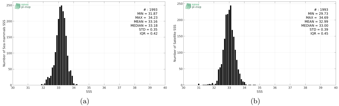
Figure 2: Histograms of SSS from Sea mammals (a) and SMAP-L3-RSS-V3-8DAY-RUNNING-70KM (b) considering all match-up pairs per bins of 0.1 over the Mid-Low Latitudes 45N-45S Pi-MEP region and for the full satellite product period.
