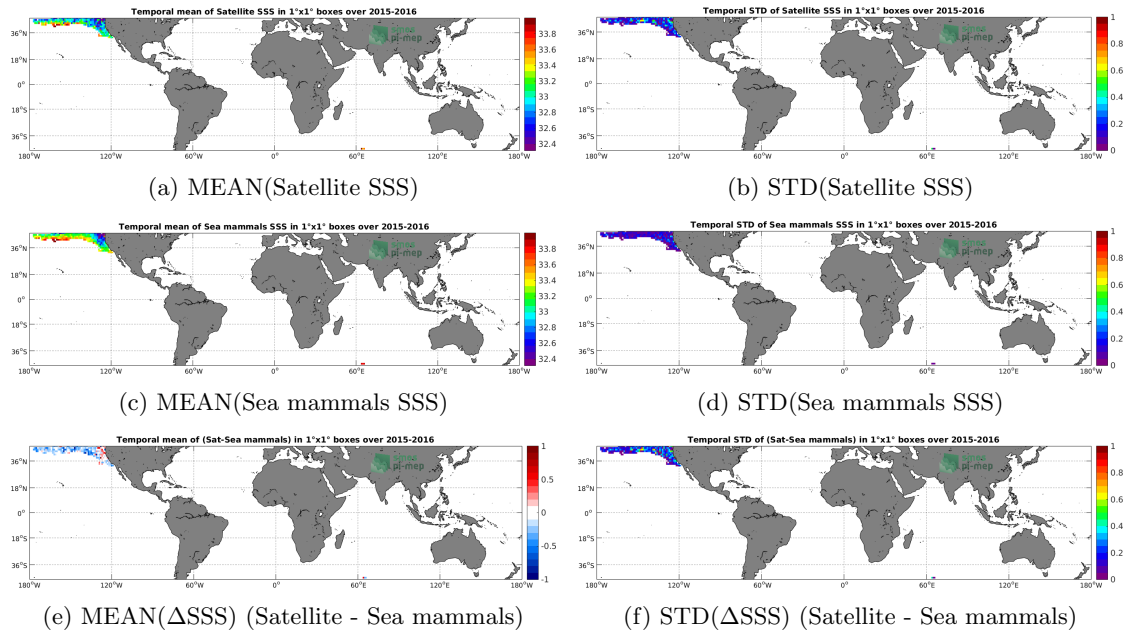
Figure 6: Temporal mean (left) and STD (right) of SSS from SMAP-L3-RSS-V3-8DAY-RUNNING-70KM (top), Sea mammals (middle), and of \Delta SSS (Satellite - Sea mammals). Only match-up pairs are used to generate these maps.
