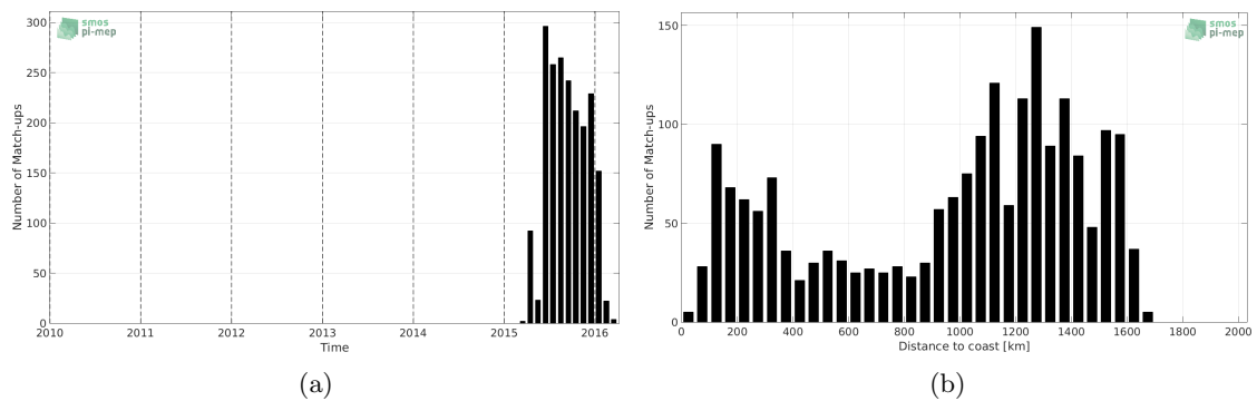
Figure 1: Number of match-ups between Sea mammals and SMAP-L3-RSS-V3-8DAY-RUNNING-70KM SSS as a function of time (a) and as function of the distance to coast (b) over the Mid-Low Latitudes 45N-45S Pi-MEP region and for the full satellite product period.
