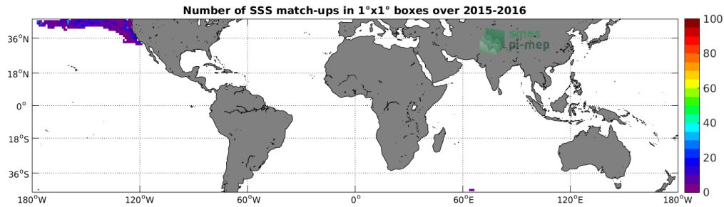
Figure 4: Number of SSS match-ups between Sea mammals SSS and the SMAP-L3-RSS-V3-8DAY-RUNNING-70KM SSS product for the Mid-Low Latitudes 45N-45S Pi-MEP region over 1^\circ \times 1^\circ boxes and for the full satellite product period.
