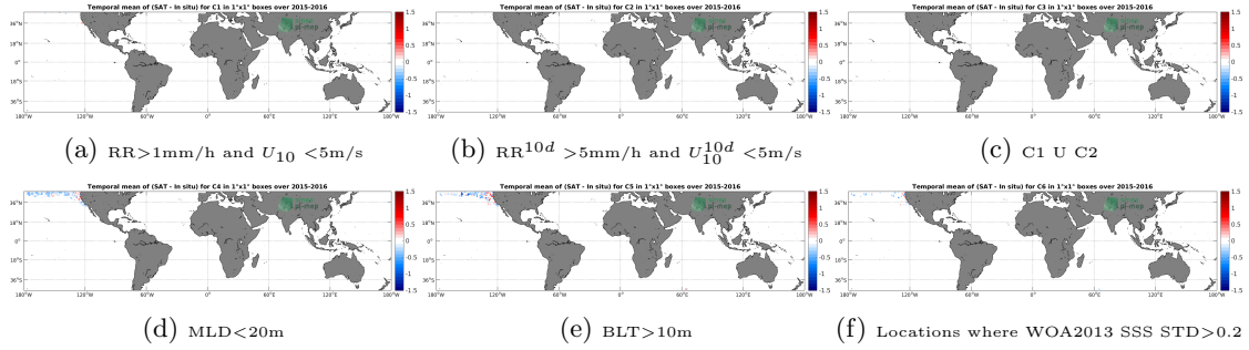
Figure 12: Temporal mean gridded over spatial boxes of size 1°x1° of \Delta SSS (SMAP-L3-RSS-V3-8DAY-RUNNING-70KM - Sea mammals) for 6 different subdatasets corresponding to:RR>1mm/h and U_{10} < 5m/s (a), RR^{10d} > 5mm/h and U_{10}^{10d} < 5m/s (b), C1 U C2 (c),MLD<20m (d),BLT>10m (e),Locations where WOA2013 SSS STD>0.2 (f).
