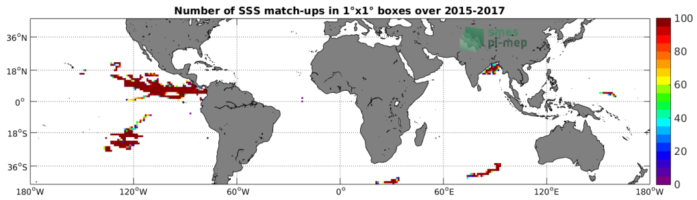
Figure 3: Number of SSS match-ups between Surface drifters SSS and the SMAP-L3-RSS-V3-8DAY-RUNNING-70KM SSS product for the Mid-Low Latitudes 45N-45S Pi-MEP region over 1°x1° boxes and for the full satellite product period.
