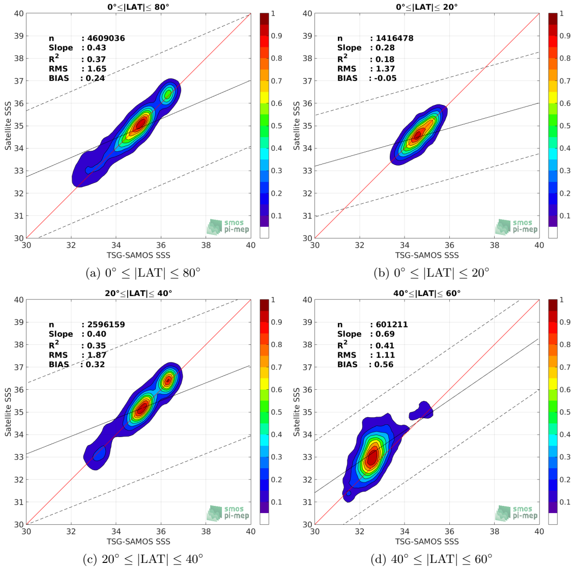
Figure 9: Contour maps of the concentration of SMAP-L3-RSS-V3-8DAY-RUNNING-40KM SSS (y-axis) versus TSG-SAMOS SSS (x-axis) at match-up pairs for different latitude bands. For each plot, the red line shows x=y . The black thin and dashed lines indicate a linear fit through the data cloud and the \pm 95\% confidence levels, respectively. The number match-up pairs n , the slope and R^2 coefficient of the linear fit, the root mean square (RMS) and the mean bias between satellite and in situ data are indicated for each latitude band in each plots.
