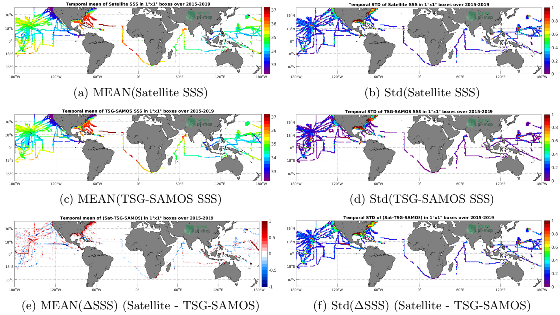
Figure 6: Temporal mean (left) and Std (right) of SSS from SMAP-L3-RSS-V3-8DAY-RUNNING-40KM (top), TSG-SAMOS (middle), and of \Delta SSS (Satellite - TSG-SAMOS). Only match-up pairs are used to generate these maps.
