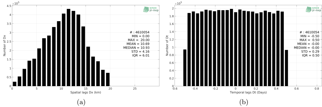
Figure 5: Histograms of the spatial (a) and temporal (b) lags between the time of the TSG-SAMOS measurements and the date of the corresponding SMAP-L3-RSS-V3-8DAY-RUNNING-40KM SSS product.
