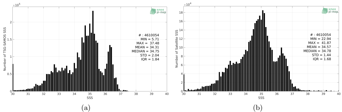
Figure 2: Histograms of SSS from TSG-SAMOS (a) and SMAP-L3-RSS-V3-8DAY-RUNNING-40KM (b) considering all match-up pairs per bins of 0.1 over the Mid-Low Latitudes 45N-45S Pi-MEP region and for the full satellite product period.
