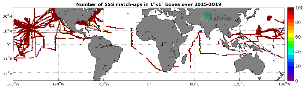
Figure 4: Number of SSS match-ups between TSG-SAMOS SSS and the SMAP-L3-RSS-V3-8DAY-RUNNING-40KM SSS product for the Mid-Low Latitudes 45N-45S Pi-MEP region over 1^\circ \times 1^\circ boxes and for the full satellite product period.
