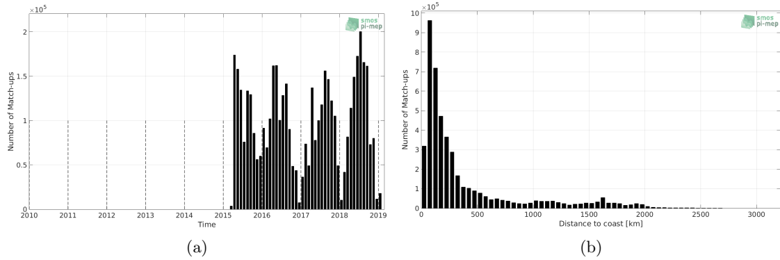
Figure 1: Number of match-ups between TSG-SAMOS and SMAP-L3-RSS-V3-8DAY-RUNNING-40KM SSS as a function of time (a) and as function of the distance to coast (b) over the Mid-Low Latitudes 45N-45S Pi-MEP region and for the full satellite product period.
