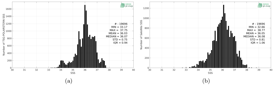
Figure 2: Histograms of SSS from TSG-POLARSTERN (a) and SMAP-L3-RSS-V3-8DAY-RUNNING-40KM (b) considering all match-up pairs per bins of 0.1 over the Mid-Low Latitudes 45N-45S Pi-MEP region and for the full satellite product period.
