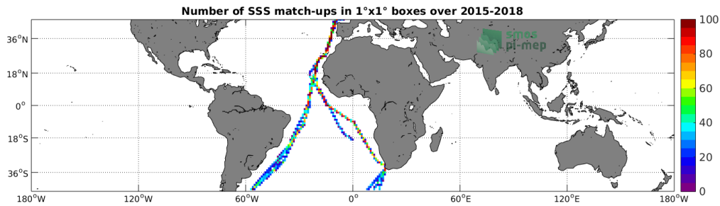
Figure 4: Number of SSS match-ups between TSG-POLARSTERN SSS and the SMAP-L3-RSS-V3-8DAY-RUNNING-40KM SSS product for the Mid-Low Latitudes 45N-45S Pi-MEP region over 1^\circ \times 1^\circ boxes and for the full satellite product period.
