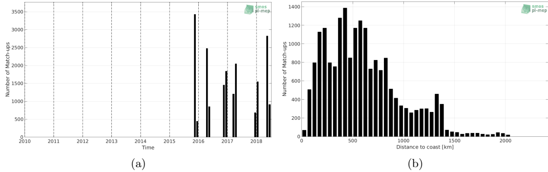
Figure 1: Number of match-ups between TSG-POLARSTERN and SMAP-L3-RSS-V3-8DAY-RUNNING-40KM SSS as a function of time (a) and as function of the distance to coast (b) over the Mid-Low Latitudes 45N-45S Pi-MEP region and for the full satellite product period.
