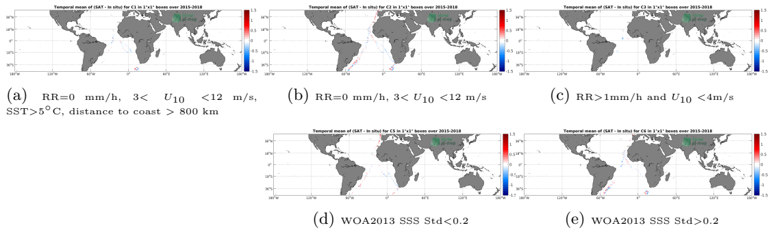
Figure 12: Temporal mean gridded over spatial boxes of size 1^\circ \times 1^\circ of \Delta SSS (SMAP-L3-RSS-V3-8DAY-RUNNING-40KM - TSG-POLARSTERN) for 5 different subdatasets corresponding to: RR=0 mm/h, 3 < U_{10} < 12 m/s, SST >5^\circ\text{C} , distance to coast > 800 km (a), RR=0 mm/h, 3 < U_{10} < 12 m/s (b), RR >1 mm/h and U_{10} < 4 m/s (c), WOA2013 SSS Std <0.2 (d), WOA2013 SSS Std >0.2 (e).
