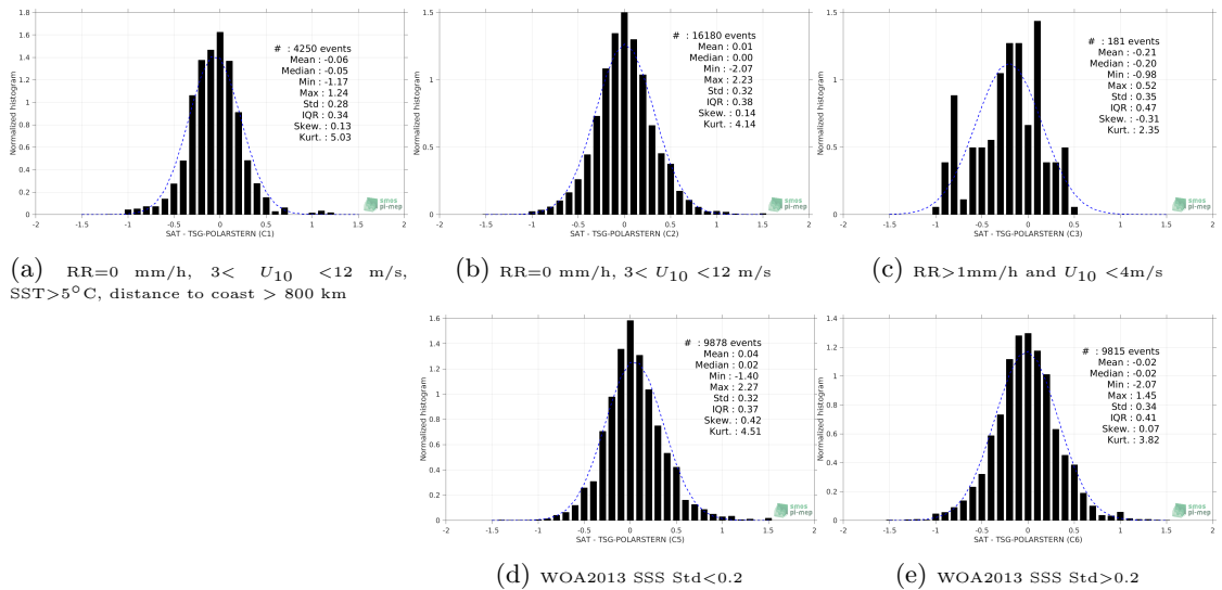
Figure 13: Normalized histogram of \Delta SSS (SMAP-L3-RSS-V3-8DAY-RUNNING-40KM - TSG-POLARSTERN) for 5 different subdatasets corresponding to: RR=0 mm/h, 3 < U_{10} < 12 m/s, SST >5^\circ\text{C} , distance to coast > 800 km (a), RR=0 mm/h, 3 < U_{10} < 12 m/s (b), RR >1 mm/h and U_{10} < 4 m/s (c), WOA2013 SSS Std <0.2 (d), WOA2013 SSS Std >0.2 (e).
