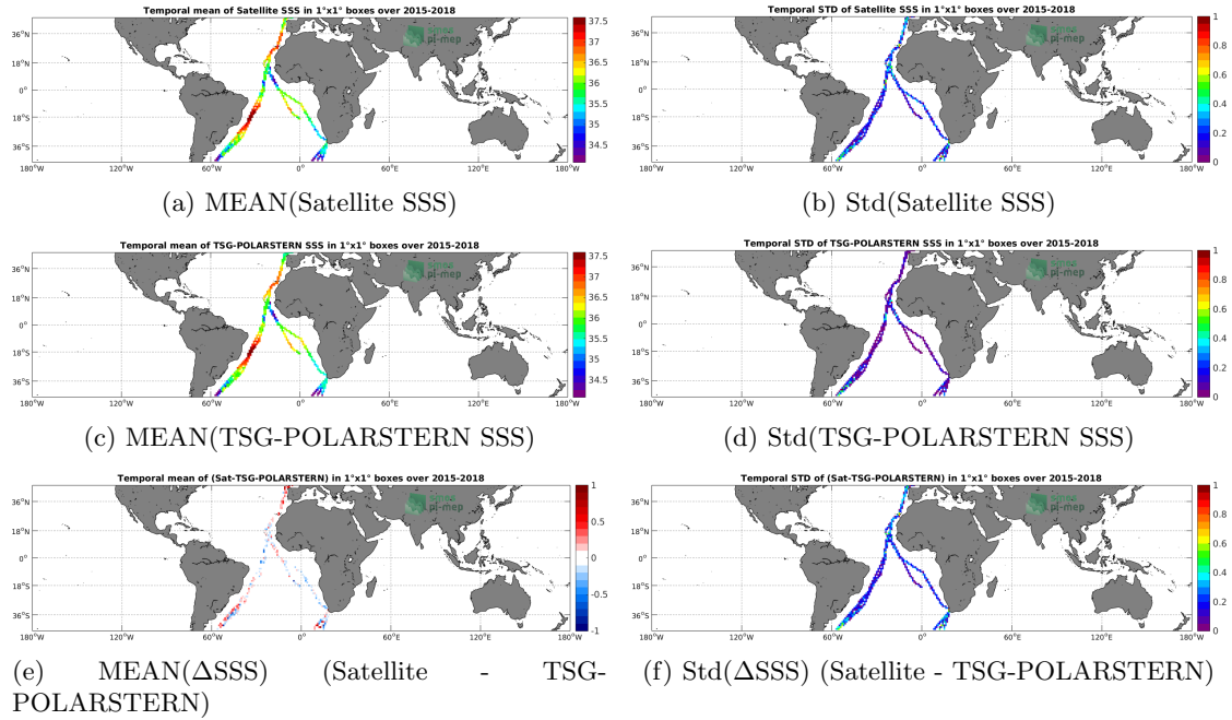
Figure 6: Temporal mean (left) and Std (right) of SSS from SMAP-L3-RSS-V3-8DAY-RUNNING-40KM (top), TSG-POLARSTERN (middle), and of \Delta SSS (Satellite - TSG-POLARSTERN). Only match-up pairs are used to generate these maps.
