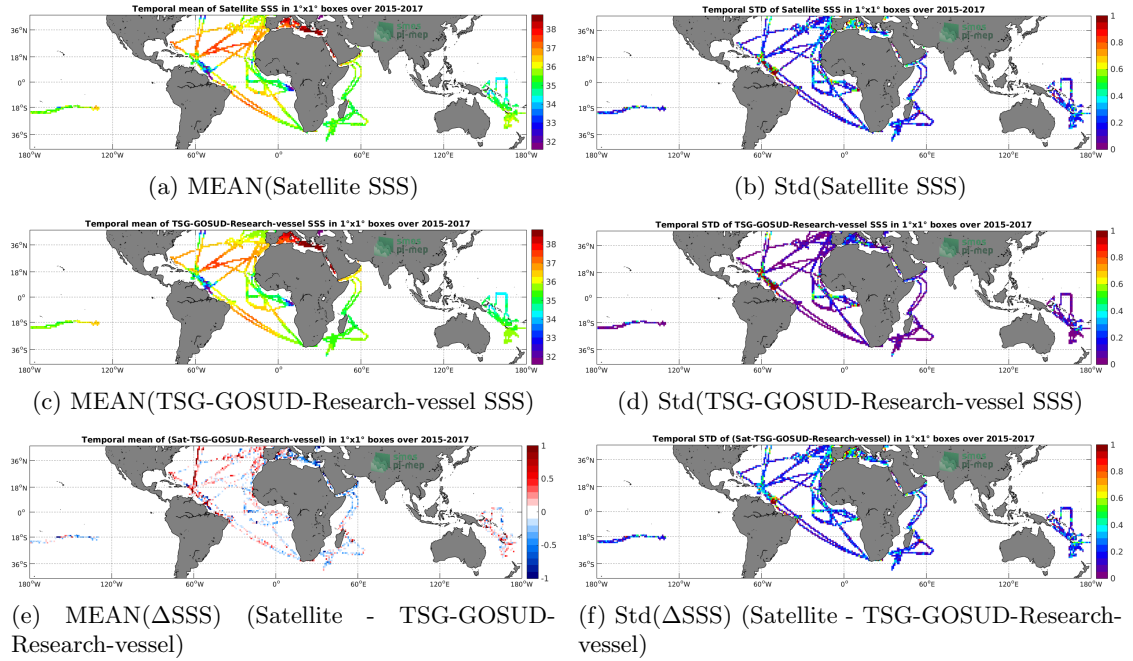
Figure 6: Temporal mean (left) and Std (right) of SSS from SMAP-L3-RSS-V3-8DAY-RUNNING-40KM (top), TSG-GOSUD-Research-vessel (middle), and of \Delta SSS (Satellite - TSG-GOSUD-Research-vessel). Only match-up pairs are used to generate these maps.
