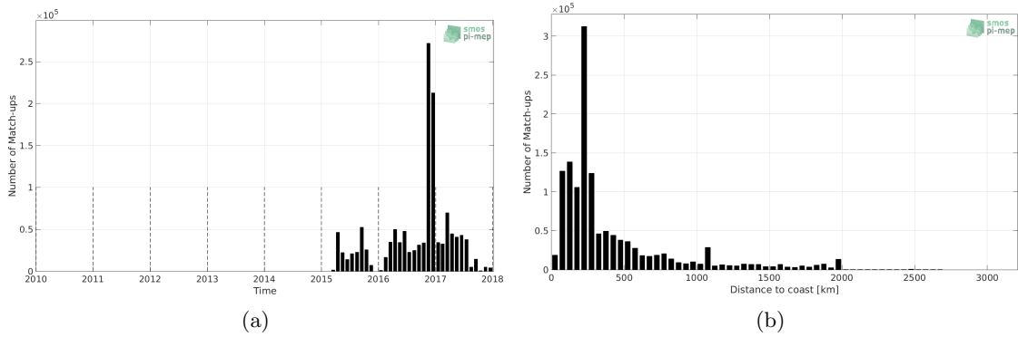
Figure 1: Number of match-ups between TSG-GOSUD-Research-vessel and SMAP-L3-RSS-V3-8DAY-RUNNING-40KM SSS as a function of time (a) and as function of the distance to coast (b) over the Mid-Low Latitudes 45N-45S Pi-MEP region and for the full satellite product period.
