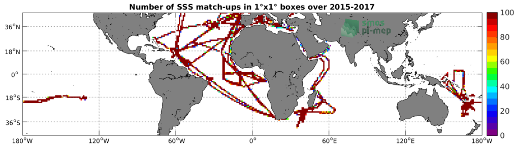
Figure 4: Number of SSS match-ups between TSG-GOSUD-Research-vessel SSS and the SMAP-L3-RSS-V3-8DAY-RUNNING-40KM SSS product for the Mid-Low Latitudes 45N-45S Pi-MEP region over 1^\circ \times 1^\circ boxes and for the full satellite product period.
