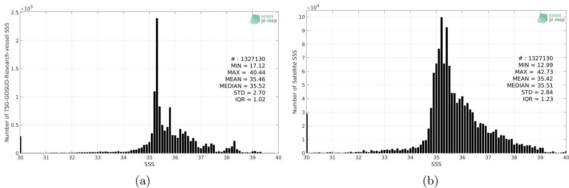
Figure 2: Histograms of SSS from TSG-GOSUD-Research-vessel (a) and SMAP-L3-RSS-V3-8DAY-RUNNING-40KM (b) considering all match-up pairs per bins of 0.1 over the Mid-Low Latitudes 45N-45S Pi-MEP region and for the full satellite product period.
