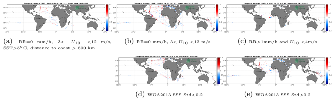
Figure 12: Temporal mean gridded over spatial boxes of size 1^\circ \times 1^\circ of \Delta SSS (SMAP-L3-RSS-V3-8DAY-RUNNING-40KM - TSG-GOSUD-Research-vessel) for 5 different subdatasets corresponding to:RR=0 mm/h, 3 < U_{10} < 12 m/s, SST >5^\circ C, distance to coast > 800 km (a), RR=0 mm/h, 3 < U_{10} < 12 m/s (b), RR >1 mm/h and U_{10} < 4 m/s (c), WOA2013 SSS Std <0.2 (d), WOA2013 SSS Std >0.2 (e).
