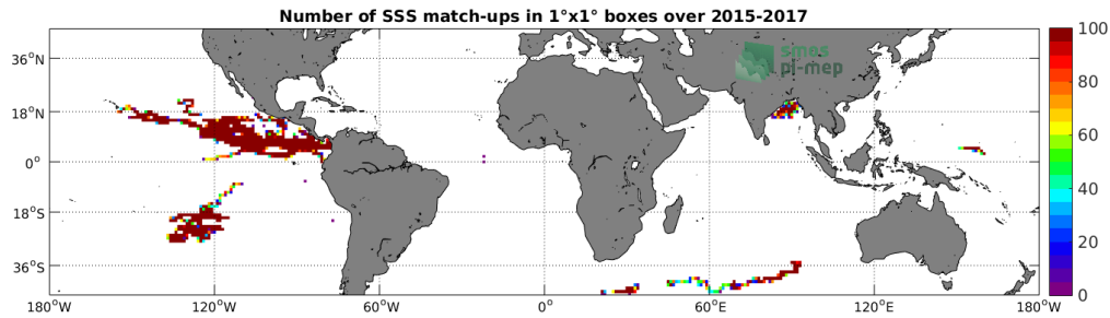
Figure 3: Number of SSS match-ups between Surface drifters SSS and the SMAP-L3-RSS-V3-8DAY-RUNNING-40KM SSS product for the Mid-Low Latitudes 45N-45S Pi-MEP region over 1^\circ \times 1^\circ boxes and for the full satellite product period.
