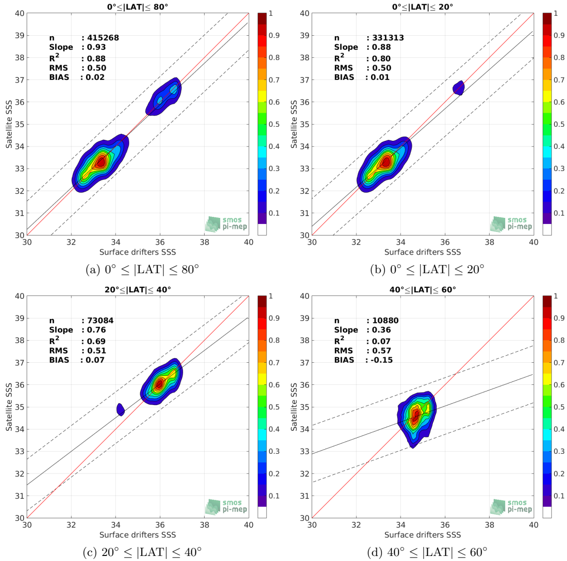
Figure 8: Contour maps of the concentration of SMAP-L3-RSS-V3-8DAY-RUNNING-40KM SSS (y-axis) versus Surface drifters SSS (x-axis) at match-up pairs for different latitude bands. For each plot, the red line shows x=y . The black thin and dashed lines indicate a linear fit through the data cloud and the \pm 95\% confidence levels, respectively. The number match-up pairs n , the slope and R^2 coefficient of the linear fit, the root mean square (RMS) and the mean bias between satellite and in situ data are indicated for each latitude band in each plots.
