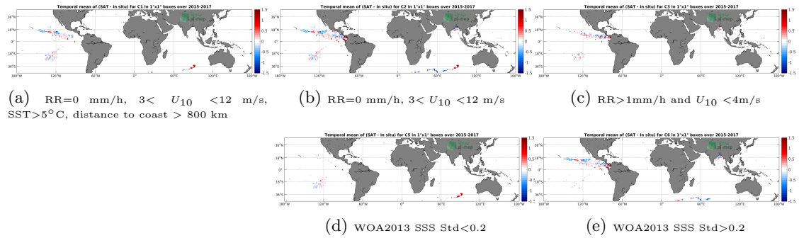
Figure 11: Temporal mean gridded over spatial boxes of size 1^\circ \times 1^\circ of \Delta SSS (SMAP-L3-RSS-V3-8DAY-RUNNING-40KM - Surface drifters) for 5 different subdatasets corresponding to:RR=0 mm/h, 3 < U_{10} < 12 m/s, SST > 5^\circ\text{C} , distance to coast > 800 km (a), RR=0 mm/h, 3 < U_{10} < 12 m/s (b), RR > 1 mm/h and U_{10} < 4 m/s (c), WOA2013 SSS Std < 0.2 (d), WOA2013 SSS Std > 0.2 (e).
