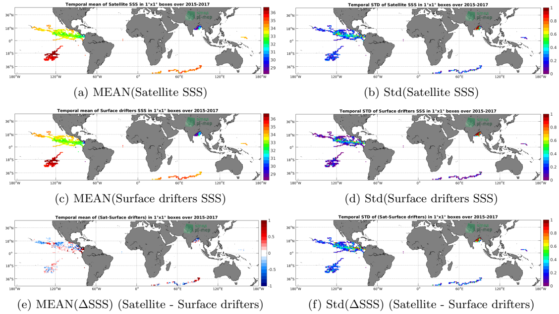
Figure 5: Temporal mean (left) and Std (right) of SSS from SMAP-L3-RSS-V3-8DAY-RUNNING-40KM (top), Surface drifters (middle), and of \Delta SSS (Satellite - Surface drifters). Only match-up pairs are used to generate these maps.
