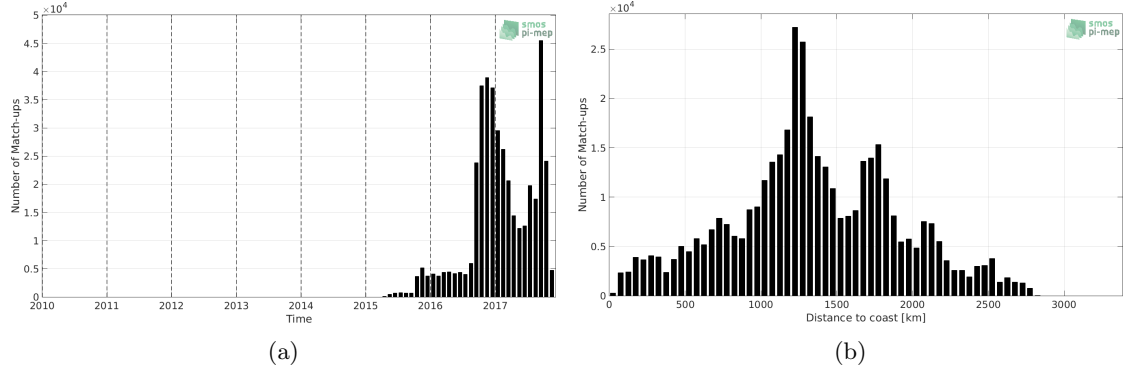
Figure 1: Number of match-ups between Surface drifters and SMAP-L3-RSS-V3-8DAY-RUNNING-40KM SSS as a function of time (a) and as function of the distance to coast (b) over the Mid-Low Latitudes 45N-45S Pi-MEP region and for the full satellite product period.
