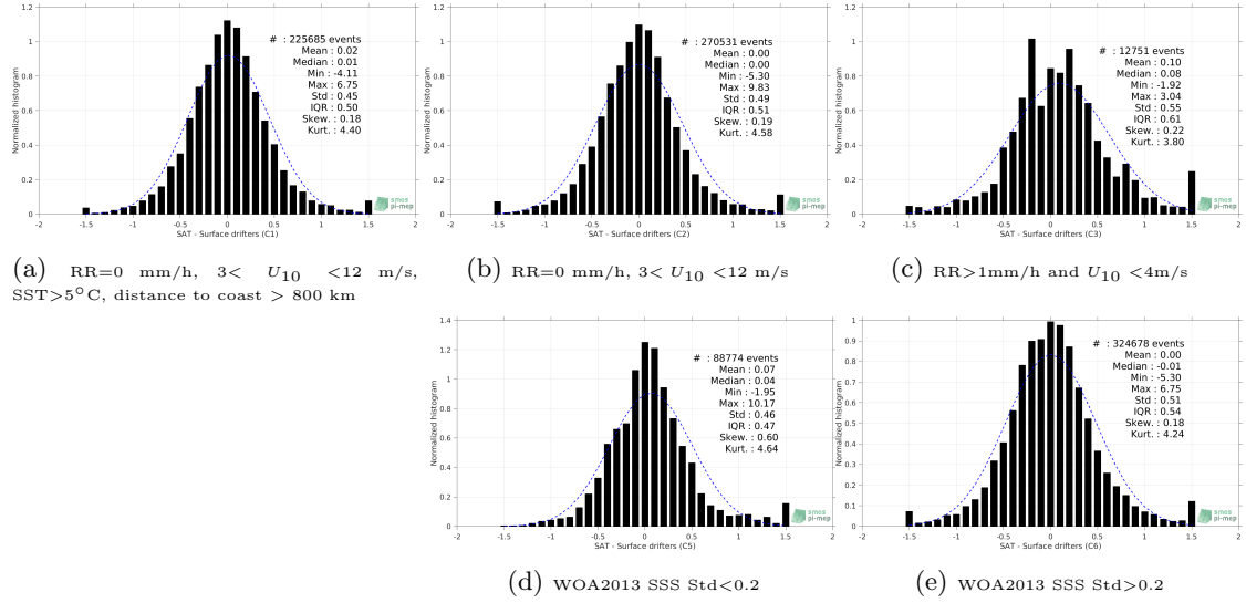
Figure 12: Normalized histogram of \Delta SSS (SMAP-L3-RSS-V3-8DAY-RUNNING-40KM - Surface drifters) for 5 different subdatasets corresponding to: RR=0 mm/h, 3 < U_{10} < 12 m/s, SST > 5°C, distance to coast > 800 km (a), RR=0 mm/h, 3 < U_{10} < 12 m/s (b), RR > 1mm/h and U_{10} < 4 m/s (c), WOA2013 SSS Std < 0.2 (d), WOA2013 SSS Std > 0.2 (e).
