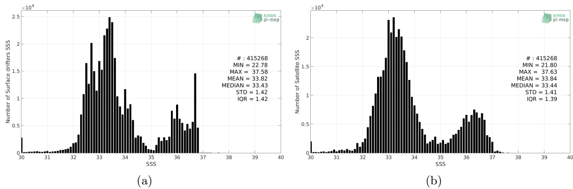
Figure 2: Histograms of SSS from Surface drifters (a) and SMAP-L3-RSS-V3-8DAY-RUNNING-40KM (b) considering all match-up pairs per bins of 0.1 over the Mid-Low Latitudes 45N-45S Pi-MEP region and for the full satellite product period.
