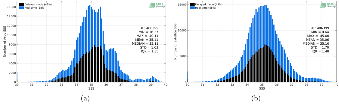
Figure 2: Histograms of SSS from Argo (a) and SMAP-L3-RSS-V3-8DAY-RUNNING-40KM (b) considering all match-up pairs per bins of 0.1 over the Mid-Low Latitudes 45N-45S Pi-MEP region and for the full satellite product period.
