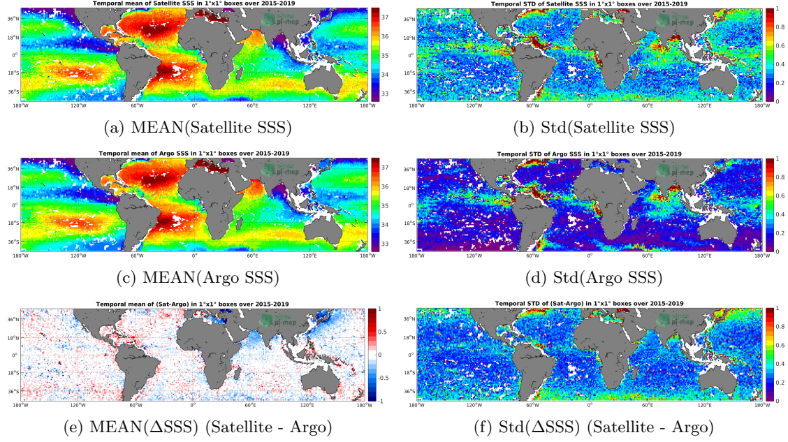
Figure 6: Temporal mean (left) and Std (right) of SSS from SMAP-L3-RSS-V3-8DAY-RUNNING-40KM satellite SSS product (in black) and the Argo in situ dataset (in blue) at the collected Pi-MEP match-up pairs. Only match-up pairs are used to generate these maps.
