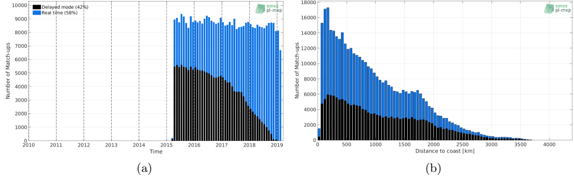
Figure 1: Number of match-ups between Argo and SMAP-L3-RSS-V3-8DAY-RUNNING-40KM SSS as a function of time (a) and as function of the distance to coast (b) over the Mid-Low Latitudes 45N-45S Pi-MEP region and for the full satellite product period.
