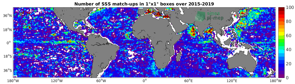
Figure 4: Number of SSS match-ups between Argo SSS and the SMAP-L3-RSS-V3-8DAY-RUNNING-40KM SSS product for the Mid-Low Latitudes 45N-45S Pi-MEP region over 1^\circ \times 1^\circ boxes and for the full satellite product period.
