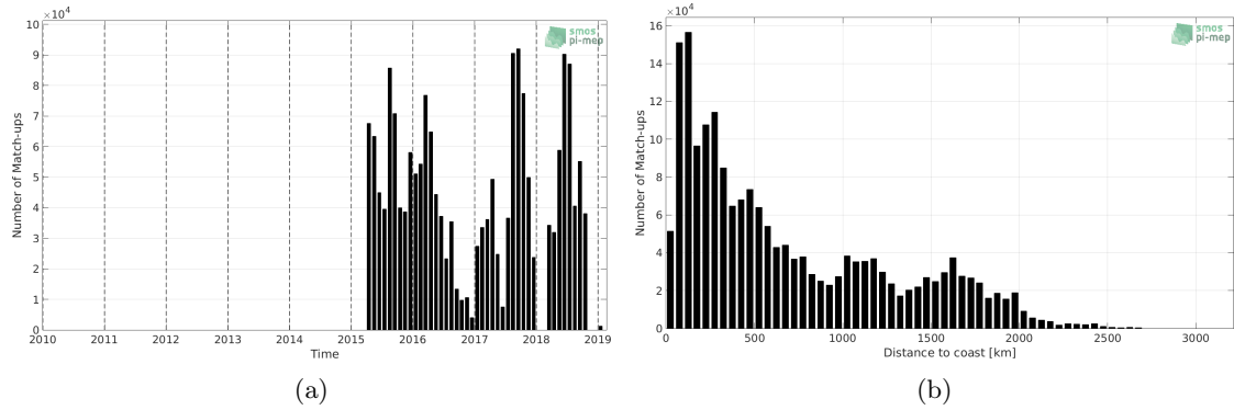
Figure 1: Number of match-ups between TSG-SAMOS and SMAP-L3-RSS-V3-MONTHLY-70KM SSS as a function of time (a) and as function of the distance to coast (b) over the Mid-Low Latitudes 45N-45S Pi-MEP region and for the full satellite product period.
