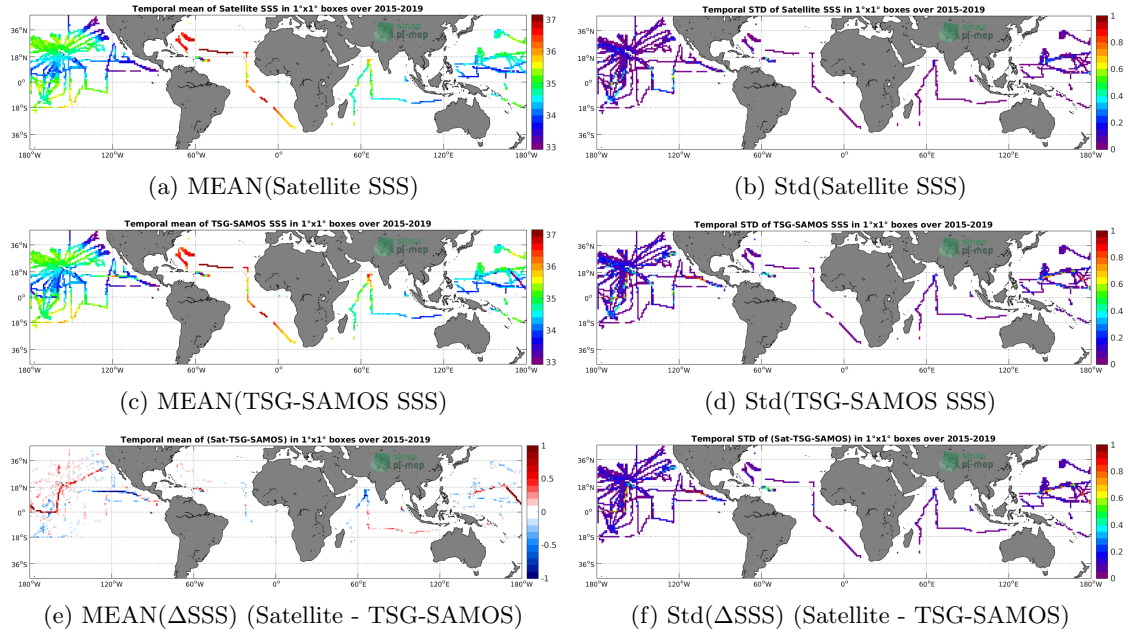
Figure 6: Temporal mean (left) and Std (right) of SSS from SMAP-L3-RSS-V3-MONTHLY-70KM (top), TSG-SAMOS (middle), and of \Delta SSS (Satellite - TSG-SAMOS). Only match-up pairs are used to generate these maps.
