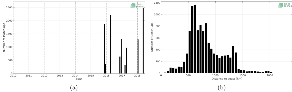
Figure 1: Number of match-ups between TSG-POLARSTERN and SMAP-L3-RSS-V3-MONTHLY-70KM SSS as a function of time (a) and as function of the distance to coast (b) over the Mid-Low Latitudes 45N-45S Pi-MEP region and for the full satellite product period.
