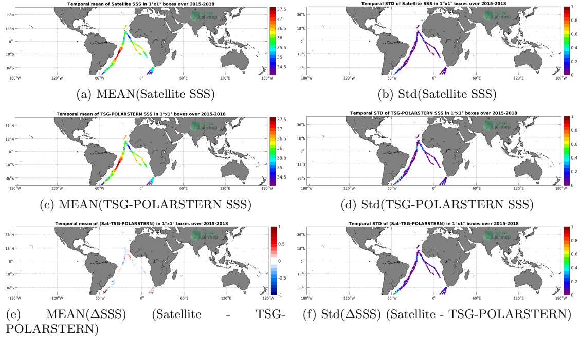
Figure 6: Temporal mean (left) and Std (right) of SSS from SMAP-L3-RSS-V3-MONTHLY-70KM (top), TSG-POLARSTERN (middle), and of \Delta SSS (Satellite - TSG-POLARSTERN). Only match-up pairs are used to generate these maps.
