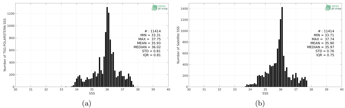
Figure 2: Histograms of SSS from TSG-POLARSTERN (a) and SMAP-L3-RSS-V3-MONTHLY-70KM (b) considering all match-up pairs per bins of 0.1 over the Mid-Low Latitudes 45N-45S Pi-MEP region and for the full satellite product period.
