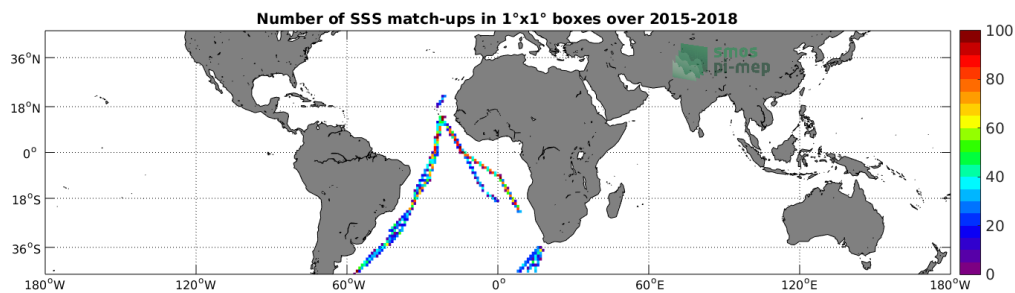
Figure 4: Number of SSS match-ups between TSG-POLARSTERN SSS and the SMAP-L3-RSS-V3-MONTHLY-70KM SSS product for the Mid-Low Latitudes 45N-45S Pi-MEP region over 1^\circ \times 1^\circ boxes and for the full satellite product period.
