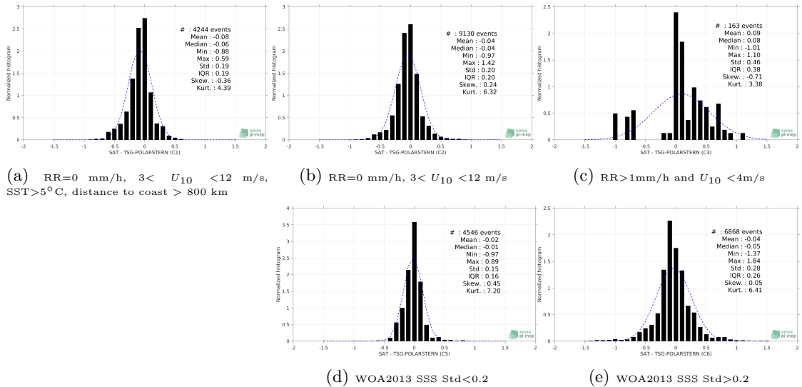
Figure 13: Normalized histogram of \Delta SSS (SMAP-L3-RSS-V3-MONTHLY-70KM - TSG-POLARSTERN) for 5 different subdatasets corresponding to: RR=0 mm/h, 3 < U_{10} < 12 m/s, SST >5^\circ\text{C} , distance to coast > 800 km (a), RR=0 mm/h, 3 < U_{10} < 12 m/s (b), RR >1 mm/h and U_{10} < 4 m/s (c), WOA2013 SSS Std <0.2 (d), WOA2013 SSS Std >0.2 (e).
