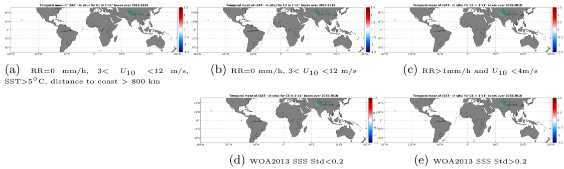
Figure 12: Temporal mean gridded over spatial boxes of size 1^\circ \times 1^\circ of \Delta SSS (SMAP-L3-RSS-V3-MONTHLY-70KM - TSG-POLARSTERN) for 5 different subdatasets corresponding to: RR=0 mm/h, 3 < U_{10} < 12 m/s, SST >5^\circ\text{C} , distance to coast > 800 km (a), RR=0 mm/h, 3 < U_{10} < 12 m/s (b), RR >1 mm/h and U_{10} < 4 m/s (c), WOA2013 SSS Std <0.2 (d), WOA2013 SSS Std >0.2 (e).
