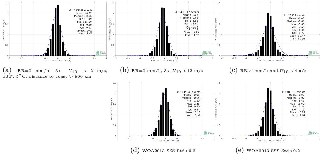
Figure 13: Normalized histogram of \Delta SSS (SMAP-L3-RSS-V3-MONTHLY-70KM - TSG-LEGOS-DM) for 5 different subdatasets corresponding to: RR=0 mm/h, 3 < U_{10} < 12 m/s, SST >5^\circ\text{C} , distance to coast > 800 km (a), RR=0 mm/h, 3 < U_{10} < 12 m/s (b), RR >1 mm/h and U_{10} < 4 m/s (c), WOA2013 SSS Std <0.2 (d), WOA2013 SSS Std >0.2 (e).
