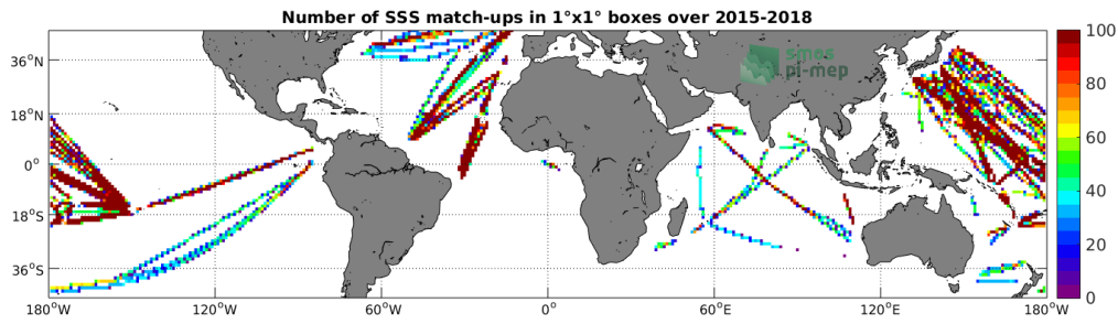
Figure 4: Number of SSS match-ups between TSG-LEGOS-DM SSS and the SMAP-L3-RSS-V3-MONTHLY-70KM SSS product for the Mid-Low Latitudes 45N-45S Pi-MEP region over 1^\circ \times 1^\circ boxes and for the full satellite product period.
