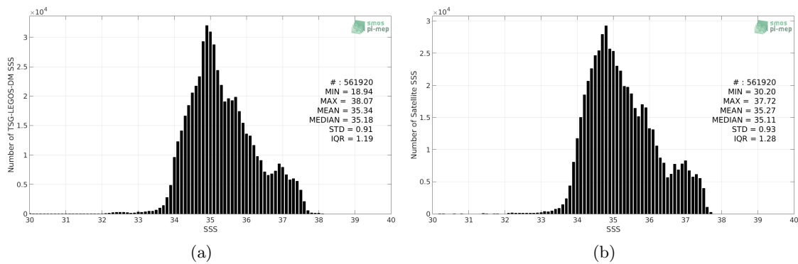
Figure 2: Histograms of SSS from TSG-LEGOS-DM (a) and SMAP-L3-RSS-V3-MONTHLY-70KM (b) considering all match-up pairs per bins of 0.1 over the Mid-Low Latitudes 45N-45S Pi-MEP region and for the full satellite product period.
