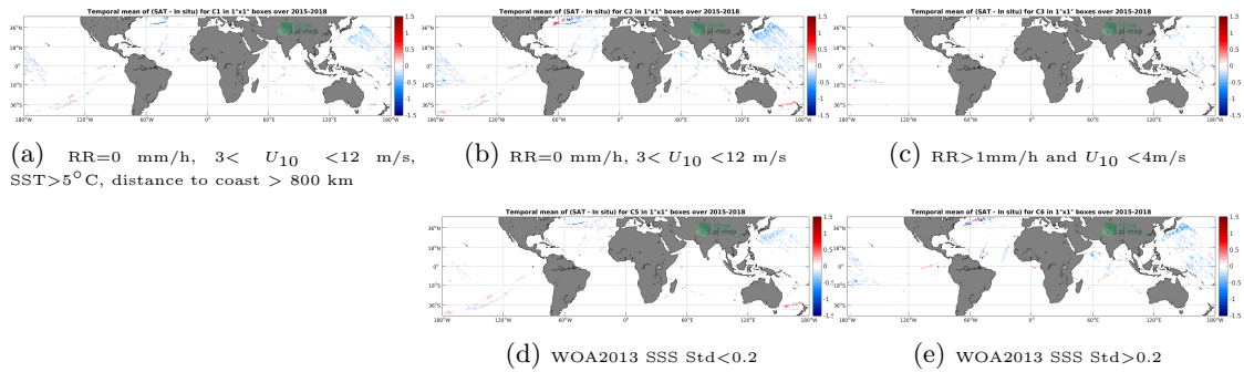
Figure 12: Temporal mean gridded over spatial boxes of size 1^\circ \times 1^\circ of \Delta SSS (SMAP-L3-RSS-V3-MONTHLY-70KM - TSG-LEGOS-DM) for 5 different subdatasets corresponding to:RR=0 mm/h, 3 < U_{10} < 12 m/s, SST >5^\circ\text{C} , distance to coast > 800 km (a), RR=0 mm/h, 3 < U_{10} < 12 m/s (b), RR >1 mm/h and U_{10} < 4 m/s (c), WOA2013 SSS Std <0.2 (d), WOA2013 SSS Std >0.2 (e).
