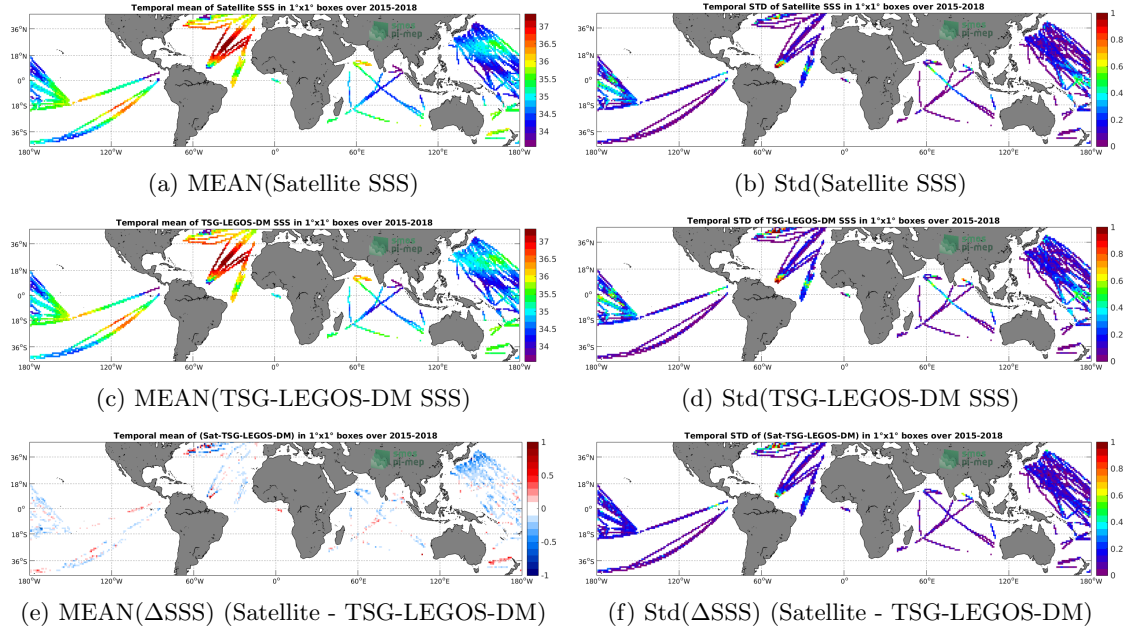
Figure 6: Temporal mean (left) and Std (right) of SSS from SMAP-L3-RSS-V3-MONTHLY-70KM (top), TSG-LEGOS-DM (middle), and of \Delta SSS (Satellite - TSG-LEGOS-DM). Only match-up pairs are used to generate these maps.
