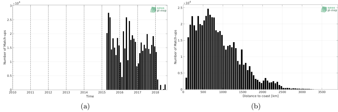
Figure 1: Number of match-ups between TSG-LEGOS-DM and SMAP-L3-RSS-V3-MONTHLY-70KM SSS as a function of time (a) and as function of the distance to coast (b) over the Mid-Low Latitudes 45N-45S Pi-MEP region and for the full satellite product period.
