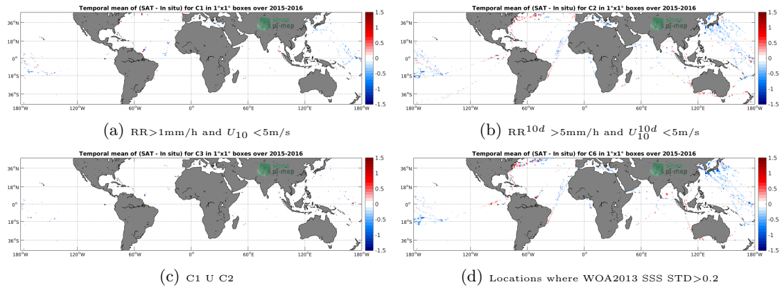
Figure 12: Temporal mean gridded over spatial boxes of size 1^\circ \times 1^\circ of \Delta SSS (SMAP-L3-RSS-V3-MONTHLY-70KM - TSG-LEGOS-DM) for 4 different subdatasets corresponding to: RR > 1\text{mm/h} and U_{10} < 5\text{m/s} (a), RR^{10d} > 5\text{mm/h} and U_{10}^{10d} < 5\text{m/s} (b), C1 U C2 (c), Locations where WOA2013 SSS STD > 0.2 (d).
