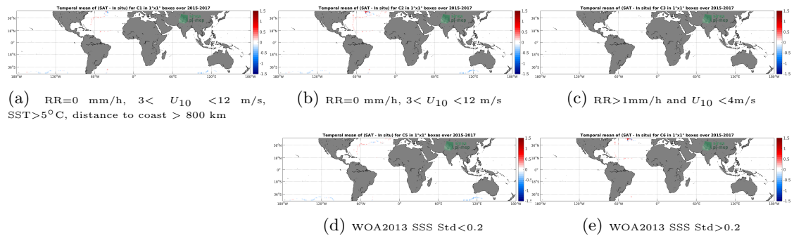
Figure 12: Temporal mean gridded over spatial boxes of size 1^\circ \times 1^\circ of \Delta SSS (SMAP-L3-RSS-V3-MONTHLY-70KM - TSG-GOSUD-Sailing-ship) for 5 different subdatasets corresponding to:RR=0 mm/h, 3 < U_{10} < 12 m/s, SST >5^\circ C, distance to coast > 800 km (a), RR=0 mm/h, 3 < U_{10} < 12 m/s (b), RR >1 mm/h and U_{10} < 4 m/s (c), WOA2013 SSS Std <0.2 (d), WOA2013 SSS Std >0.2 (e).
