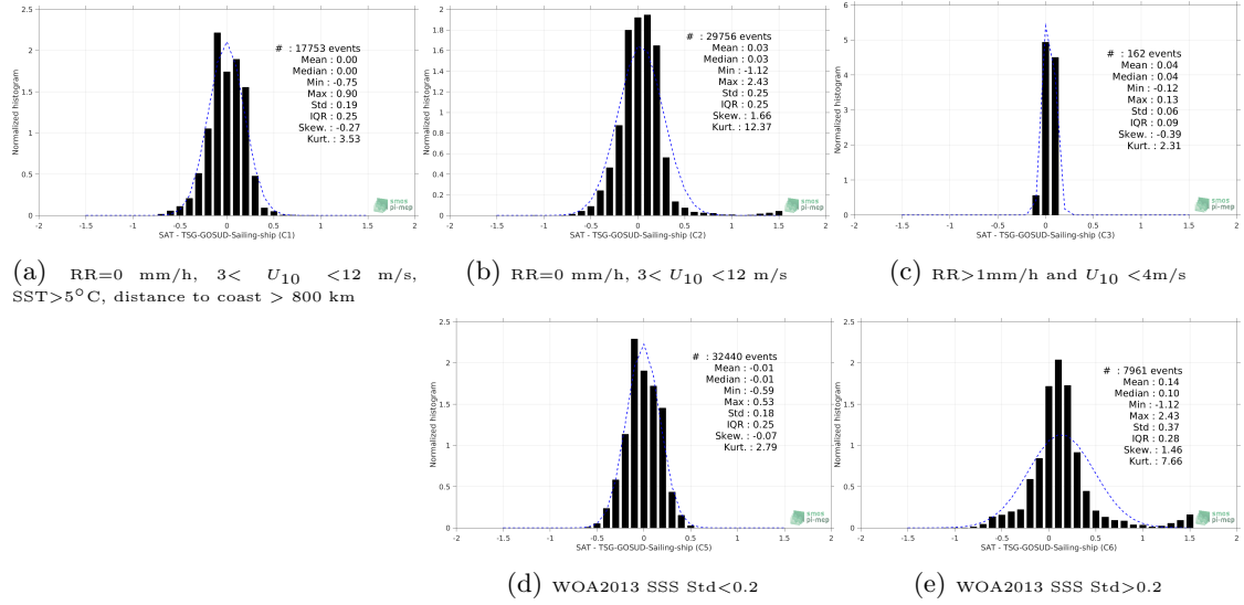
Figure 13: Normalized histogram of \Delta SSS (SMAP-L3-RSS-V3-MONTHLY-70KM - TSG-GOSUD-Sailing-ship) for 5 different subdatasets corresponding to: RR=0 mm/h, 3 < U_{10} < 12 m/s, SST>5°C, distance to coast > 800 km (a), RR=0 mm/h, 3 < U_{10} < 12 m/s (b), RR>1mm/h and U_{10} < 4 m/s (c), WOA2013 SSS Std<0.2 (d), WOA2013 SSS Std>0.2 (e).
