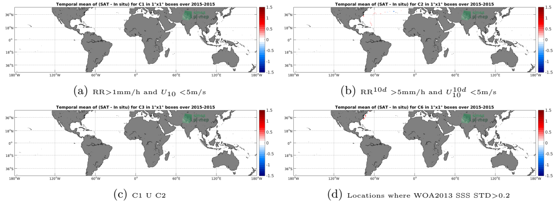
Figure 12: Temporal mean gridded over spatial boxes of size 1^\circ \times 1^\circ of \Delta SSS (SMAP-L3-RSS-V3-MONTHLY-70KM - TSG-GOSUD-Sailing-ship) for 4 different subdatasets corresponding to: RR > 1\text{mm/h} and U_{10} < 5\text{m/s} (a), RR^{10d} > 5\text{mm/h} and U_{10}^{10d} < 5\text{m/s} (b), C1 U C2 (c), Locations where WOA2013 SSS STD > 0.2 (d).
