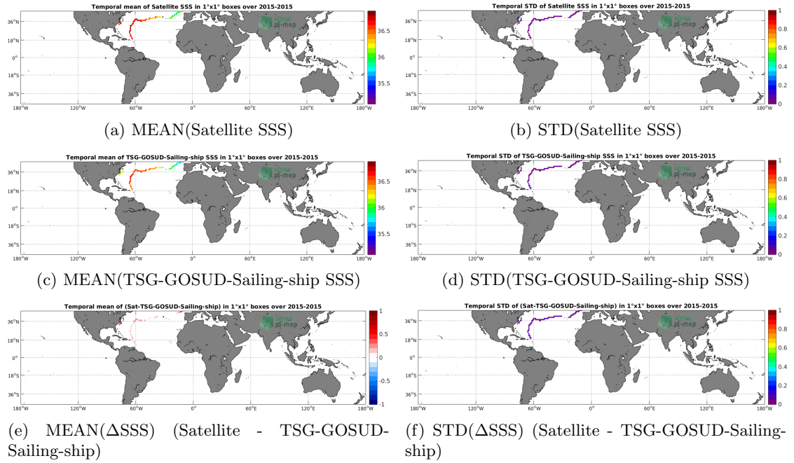
Figure 6: Temporal mean (left) and STD (right) of SSS from SMAP-L3-RSS-V3-MONTHLY-70KM (top), TSG-GOSUD-Sailing-ship (middle), and of \Delta SSS (Satellite - TSG-GOSUD-Sailing-ship). Only match-up pairs are used to generate these maps.
