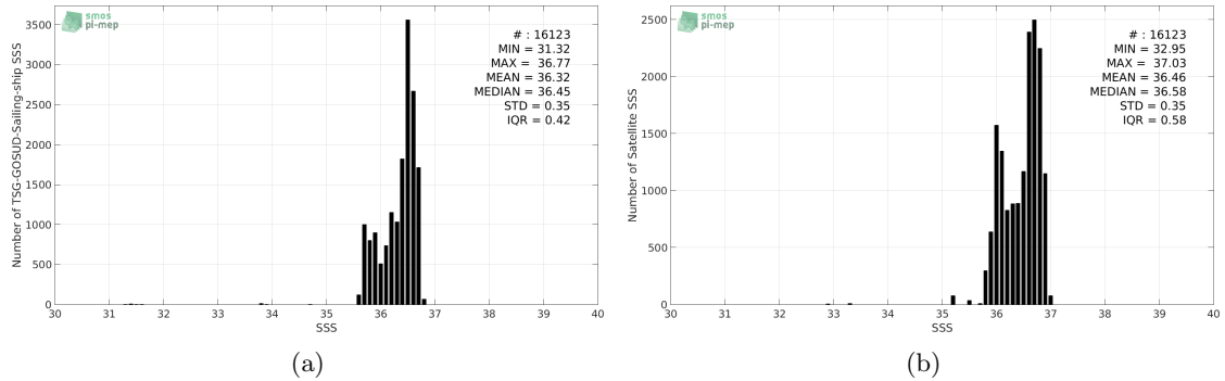
Figure 2: Histograms of SSS from TSG-GOSUD-Sailing-ship (a) and SMAP-L3-RSS-V3-MONTHLY-70KM (b) considering all match-up pairs per bins of 0.1 over the Mid-Low Latitudes 45N-45S Pi-MEP region and for the full satellite product period.
