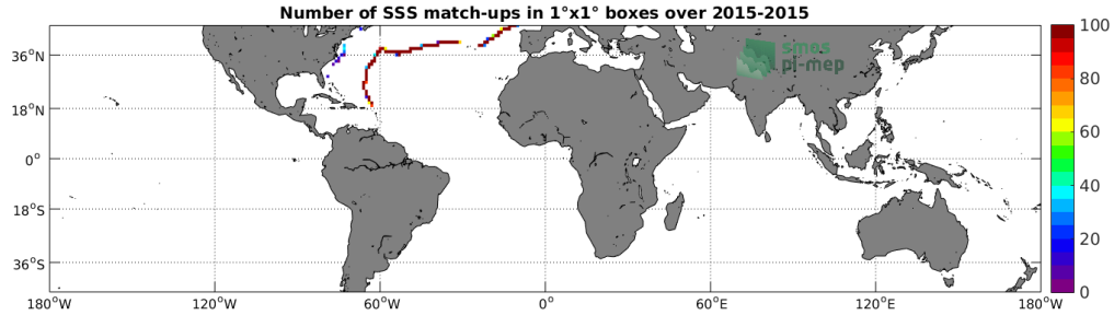
Figure 4: Number of SSS match-ups between TSG-GOSUD-Sailing-ship SSS and the SMAP-L3-RSS-V3-MONTHLY-70KM SSS product for the Mid-Low Latitudes 45N-45S Pi-MEP region over 1^\circ \times 1^\circ boxes and for the full satellite product period.
