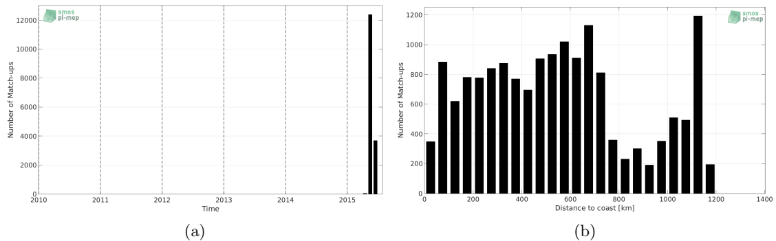
Figure 1: Number of match-ups between TSG-GOSUD-Sailing-ship and SMAP-L3-RSS-V3-MONTHLY-70KM SSS as a function of time (a) and as function of the distance to coast (b) over the Mid-Low Latitudes 45N-45S Pi-MEP region and for the full satellite product period.
