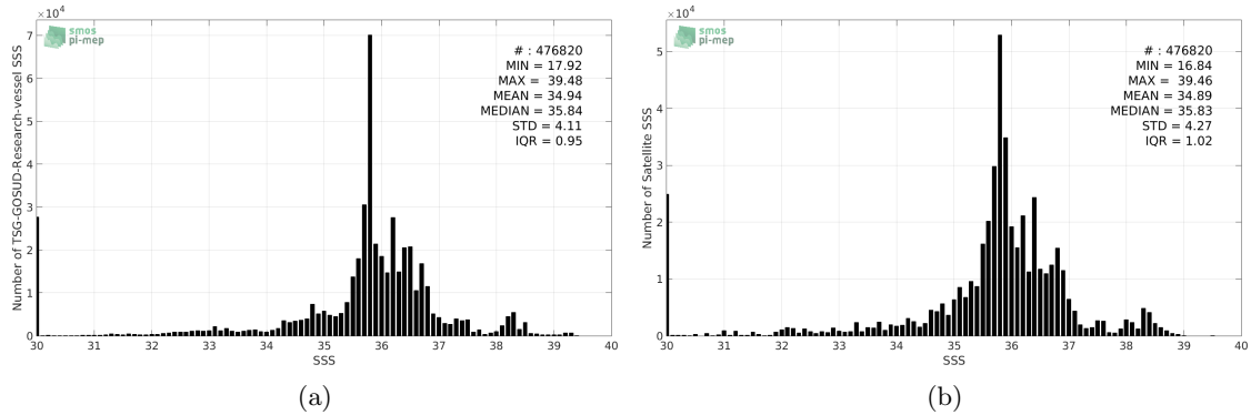
Figure 2: Histograms of SSS from TSG-GOSUD-Research-vessel (a) and SMAP-L3-RSS-V3-MONTHLY-70KM (b) considering all match-up pairs per bins of 0.1 over the Mid-Low Latitudes 45N-45S Pi-MEP region and for the full satellite product period.
