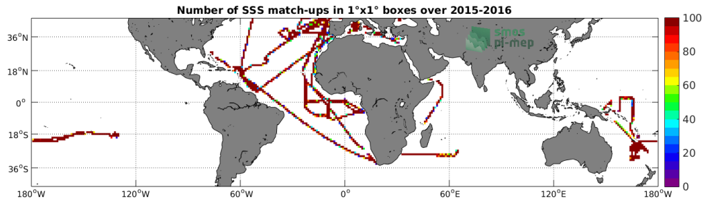
Figure 4: Number of SSS match-ups between TSG-GOSUD-Research-vessel SSS and the SMAP-L3-RSS-V3-MONTHLY-70KM SSS product for the Mid-Low Latitudes 45N-45S Pi-MEP region over 1^\circ \times 1^\circ boxes and for the full satellite product period.
