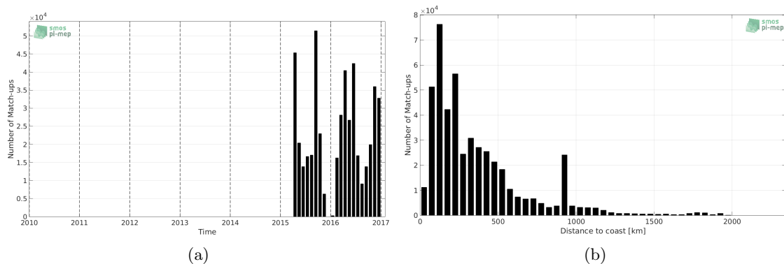
Figure 1: Number of match-ups between TSG-GOSUD-Research-vessel and SMAP-L3-RSS-V3-MONTHLY-70KM SSS as a function of time (a) and as function of the distance to coast (b) over the Mid-Low Latitudes 45N-45S Pi-MEP region and for the full satellite product period.
