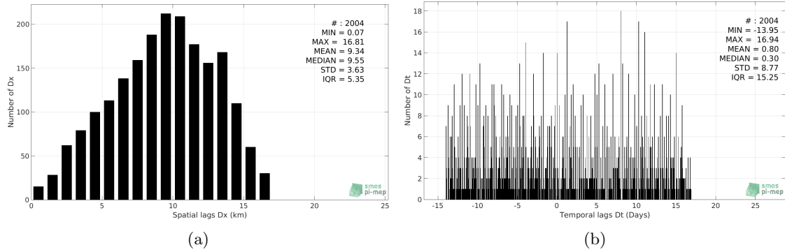
Figure 5: Histograms of the spatial (a) and temporal (b) lags between the time of the Sea mammals measurements and the date of the corresponding SMAP-L3-RSS-V3-MONTHLY-70KM SSS product.
