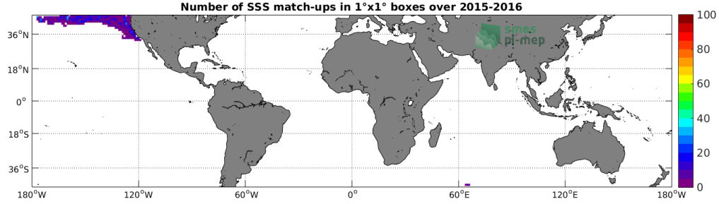
Figure 4: Number of SSS match-ups between Sea mammals SSS and the SMAP-L3-RSS-V3-MONTHLY-70KM SSS product for the Mid-Low Latitudes 45N-45S Pi-MEP region over 1°x1° boxes and for the full satellite product period.
