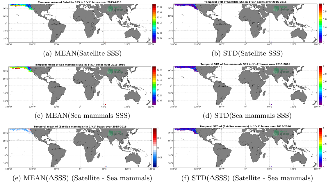
Figure 6: Temporal mean (left) and STD (right) of SSS from SMAP-L3-RSS-V3-MONTHLY-70KM (top), Sea mammals (middle), and of \Delta SSS (Satellite - Sea mammals). Only match-up pairs are used to generate these maps.
