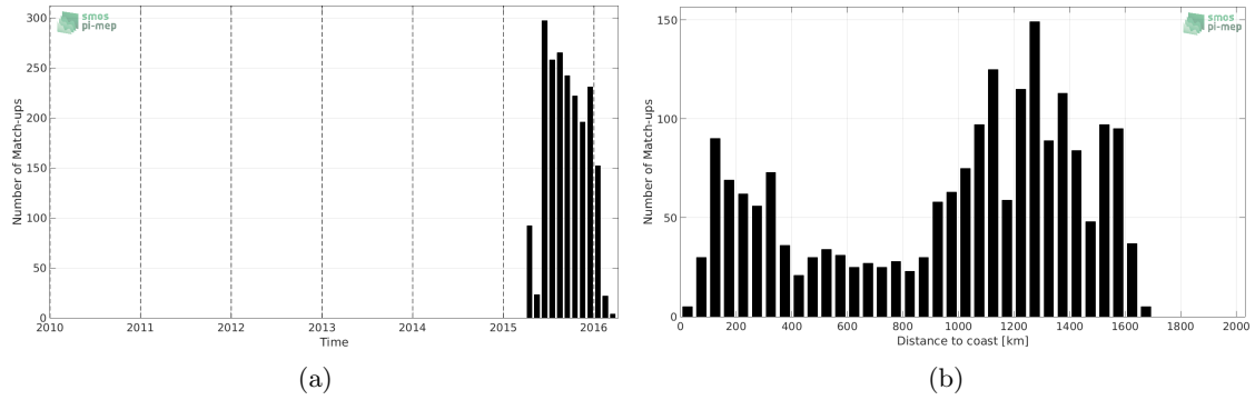
Figure 1: Number of match-ups between Sea mammals and SMAP-L3-RSS-V3-MONTHLY-70KM SSS as a function of time (a) and as function of the distance to coast (b) over the Mid-Low Latitudes 45N-45S Pi-MEP region and for the full satellite product period.
