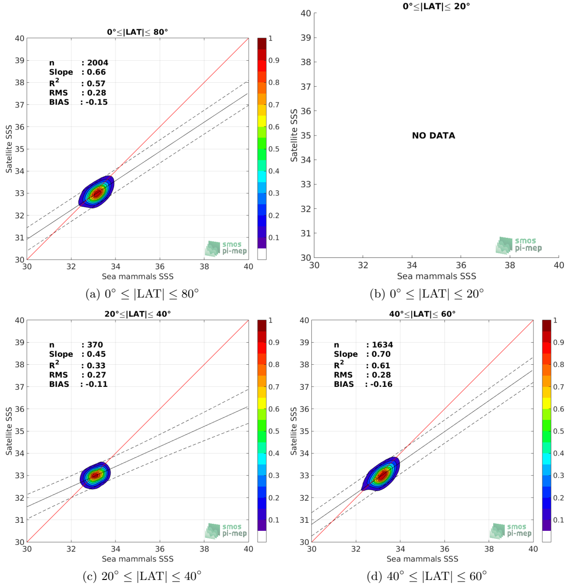
Figure 9: Contour maps of the concentration of SMAP-L3-RSS-V3-MONTHLY-70KM SSS (y-axis) versus Sea mammals SSS (x-axis) at match-up pairs for different latitude bands. For each plot, the red line shows x=y . The black thin and dashed lines indicate a linear fit through the data cloud and the \pm 95\% confidence levels, respectively. The number match-up pairs n , the slope and R^2 coefficient of the linear fit, the root mean square (RMS) and the mean bias between satellite and in situ data are indicated for each latitude band in each plots.
