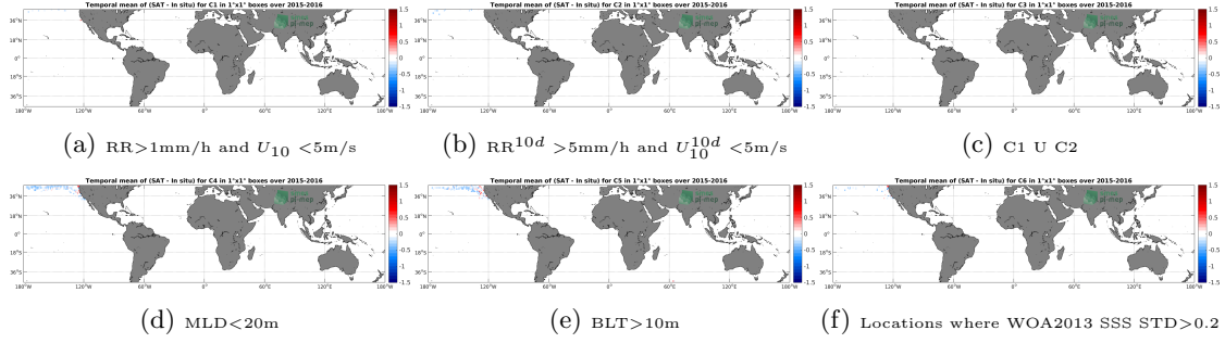
Figure 12: Temporal mean gridded over spatial boxes of size 1^\circ \times 1^\circ of \Delta\text{SSS} (SMAP-L3-RSS-V3-MONTHLY-70KM - Sea mammals) for 6 different subdatasets corresponding to: \text{RR} > 1\text{mm/h} and U_{10} < 5\text{m/s} (a), \text{RR}^{10d} > 5\text{mm/h} and U_{10}^{10d} < 5\text{m/s} (b), C1 U C2 (c), \text{MLD} < 20\text{m} (d), \text{BLT} > 10\text{m} (e), Locations where WOA2013 SSS STD > 0.2 (f).
