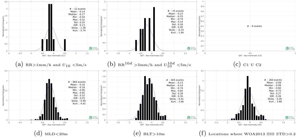
Figure 13: Normalized histogram of \Delta\text{SSS} (SMAP-L3-RSS-V3-MONTHLY-70KM - Sea mammals) for 6 different subdatasets corresponding to: \text{RR} > 1\text{mm/h} and U_{10} < 5\text{m/s} (a), \text{RR}^{10d} > 5\text{mm/h} and U_{10}^{10d} < 5\text{m/s} (b), C1 U C2 (c), \text{MLD} < 20\text{m} (d), \text{BLT} > 10\text{m} (e), Locations where WOA2013 SSS STD > 0.2 (f).
