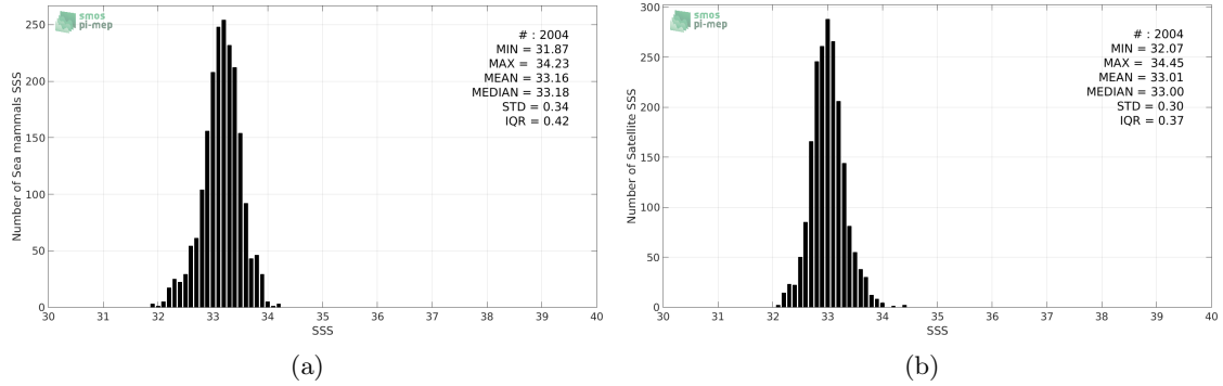
Figure 2: Histograms of SSS from Sea mammals (a) and SMAP-L3-RSS-V3-MONTHLY-70KM (b) considering all match-up pairs per bins of 0.1 over the Mid-Low Latitudes 45N-45S Pi-MEP region and for the full satellite product period.
