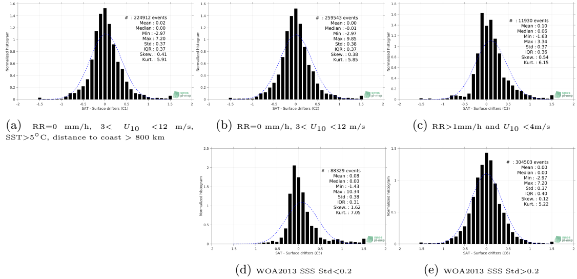
Figure 12: Normalized histogram of \Delta SSS (SMAP-L3-RSS-V3-MONTHLY-70KM - Surface drifters) for 5 different subdatasets corresponding to: RR=0 mm/h, 3 < U_{10} < 12 m/s, SST > 5^\circ C , distance to coast > 800 km (a), RR=0 mm/h, 3 < U_{10} < 12 m/s (b), RR > 1 mm/h and U_{10} < 4 m/s (c), WOA2013 SSS Std <0.2 (d), WOA2013 SSS Std >0.2 (e).
