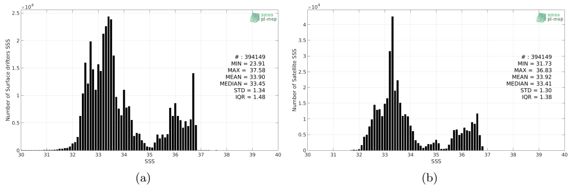
Figure 2: Histograms of SSS from Surface drifters (a) and SMAP-L3-RSS-V3-MONTHLY-70KM (b) considering all match-up pairs per bins of 0.1 over the Mid-Low Latitudes 45N-45S Pi-MEP region and for the full satellite product period.
