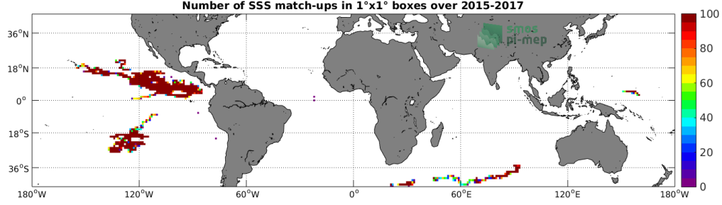
Figure 3: Number of SSS match-ups between Surface drifters SSS and the SMAP-L3-RSS-V3-MONTHLY-70KM SSS product for the Mid-Low Latitudes 45N-45S Pi-MEP region over 1^\circ \times 1^\circ boxes and for the full satellite product period.
