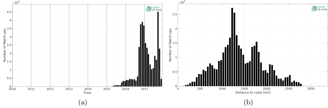
Figure 1: Number of match-ups between Surface drifters and SMAP-L3-RSS-V3-MONTHLY-70KM SSS as a function of time (a) and as function of the distance to coast (b) over the Mid-Low Latitudes 45N-45S Pi-MEP region and for the full satellite product period.
