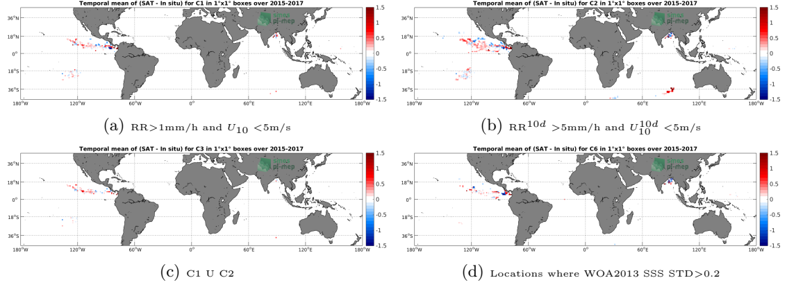
Figure 11: Temporal mean gridded over spatial boxes of size 1^\circ \times 1^\circ of \Delta SSS (SMAP-L3-RSS-V3-MONTHLY-70KM - Surface drifters) for 4 different subdatasets corresponding to: RR > 1\text{mm/h} and U_{10} < 5\text{m/s} (a), RR^{10d} > 5\text{mm/h} and U_{10}^{10d} < 5\text{m/s} (b), C1 U C2 (c), Locations where WOA2013 SSS STD > 0.2 (d).
