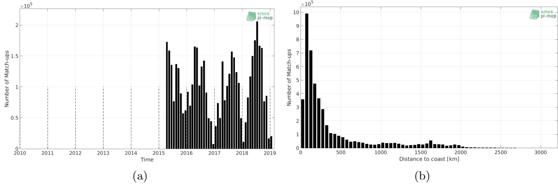
Figure 1: Number of match-ups between TSG-SAMOS and SMAP-L3-RSS-V3-MONTHLY-0.25DEG-40KM SSS as a function of time (a) and as function of the distance to coast (b) over the Mid-Low Latitudes 45N-45S Pi-MEP region and for the full satellite product period.
