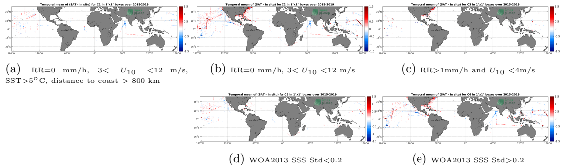
Figure 12: Temporal mean gridded over spatial boxes of size 1^\circ \times 1^\circ of \Delta SSS (SMAP-L3-RSS-V3-MONTHLY-0.25DEG-40KM - TSG-SAMOS) for 5 different subdatasets corresponding to:RR=0 mm/h, 3 < U_{10} < 12 m/s, SST > 5^\circ\text{C} , distance to coast > 800 km (a), RR=0 mm/h, 3 < U_{10} < 12 m/s (b), RR > 1 mm/h and U_{10} < 4 m/s (c), WOA2013 SSS Std < 0.2 (d), WOA2013 SSS Std > 0.2 (e).
