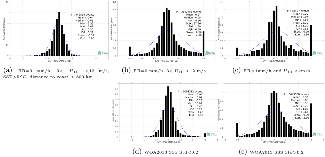
Figure 13: Normalized histogram of \Delta\text{SSS} (SMAP-L3-RSS-V3-MONTHLY-0.25DEG-40KM - TSG-SAMOS) for 5 different subdatasets corresponding to: RR=0 mm/h, 3 < U_{10} < 12 m/s, SST >5^{\circ}\text{C} , distance to coast > 800 km (a), RR=0 mm/h, 3 < U_{10} < 12 m/s (b), RR >1 mm/h and U_{10} < 4 m/s (c), WOA2013 SSS Std <0.2 (d), WOA2013 SSS Std >0.2 (e).
