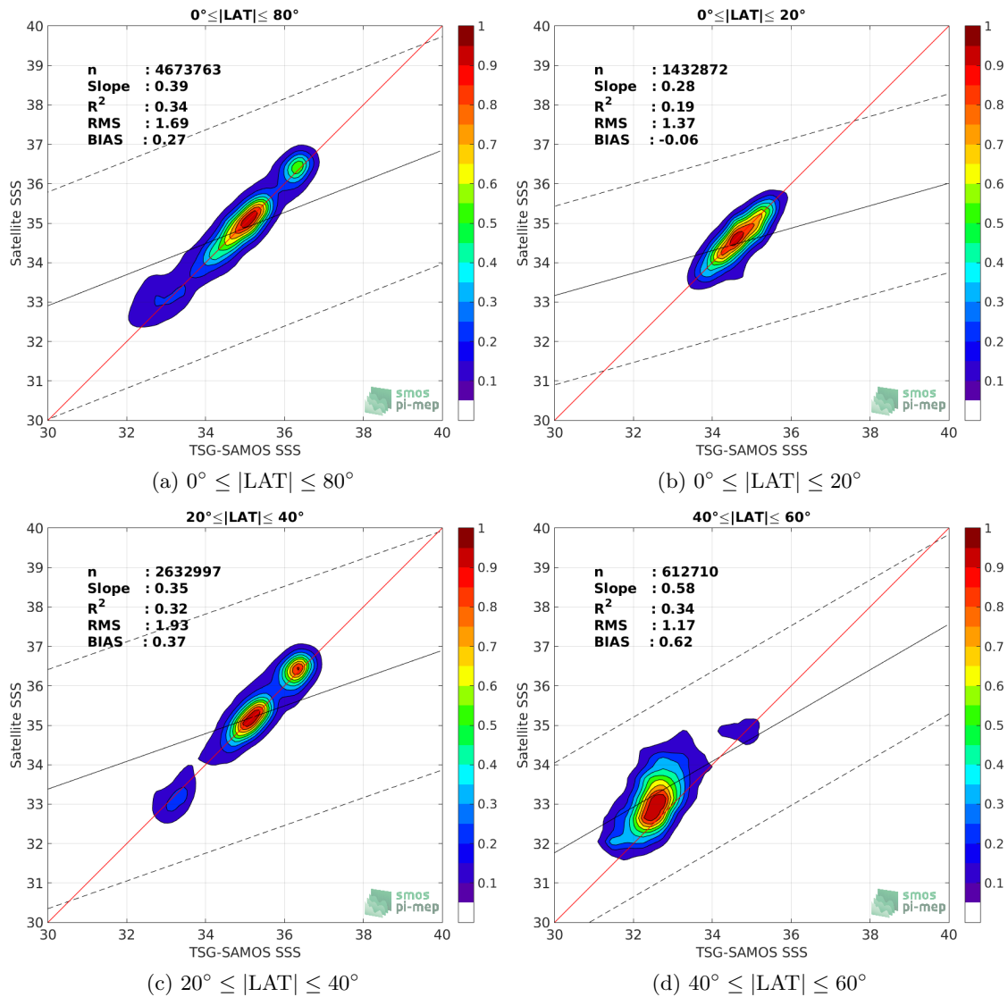
Figure 9: Contour maps of the concentration of SMAP-L3-RSS-V3-MONTHLY-0.25DEG-40KM SSS (y-axis) versus TSG-SAMOS SSS (x-axis) at match-up pairs for different latitude bands. For each plot, the red line shows x=y . The black thin and dashed lines indicate a linear fit through the data cloud and the \pm 95\% confidence levels, respectively. The number match-up pairs n , the slope and R^2 coefficient of the linear fit, the root mean square (RMS) and the mean bias between satellite and in situ data are indicated for each latitude band in each plots.
