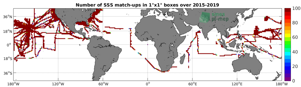
Figure 4: Number of SSS match-ups between TSG-SAMOS SSS and the SMAP-L3-RSS-V3-MONTHLY-0.25DEG-40KM SSS product for the Mid-Low Latitudes 45N-45S Pi-MEP region over 1^\circ \times 1^\circ boxes and for the full satellite product period.
