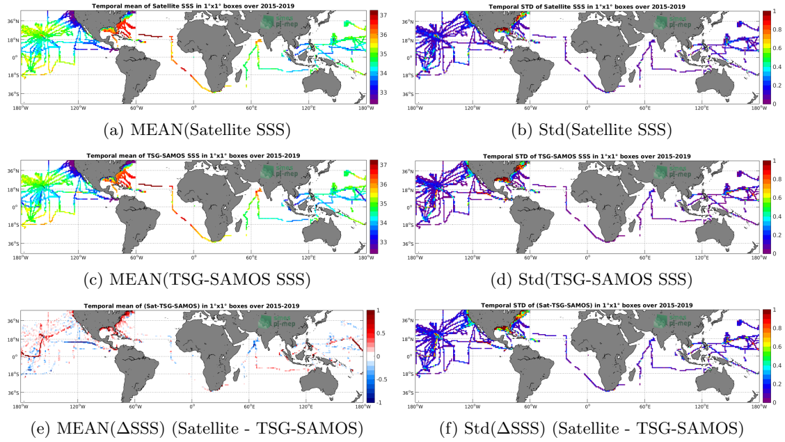
Figure 6: Temporal mean (left) and Std (right) of SSS from SMAP-L3-RSS-V3-MONTHLY-0.25DEG-40KM (top), TSG-SAMOS (middle), and of \Delta SSS (Satellite - TSG-SAMOS). Only match-up pairs are used to generate these maps.
