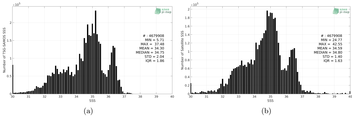
Figure 2: Histograms of SSS from TSG-SAMOS (a) and SMAP-L3-RSS-V3-MONTHLY-0.25DEG-40KM (b) considering all match-up pairs per bins of 0.1 over the Mid-Low Latitudes 45N-45S Pi-MEP region and for the full satellite product period.
