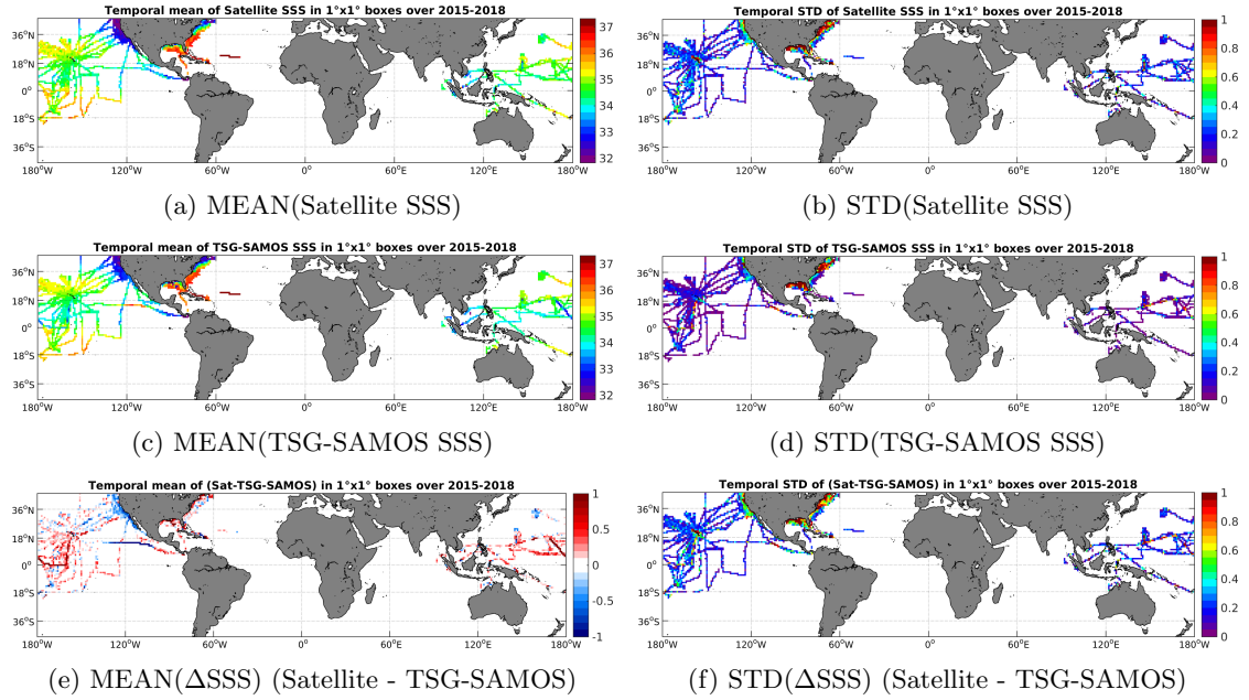
Figure 6: Temporal mean (left) and STD (right) of SSS from SMAP-L3-RSS-V2-8DAY-RUNNING-40KM satellite SSS (top), TSG-SAMOS (middle), and of \Delta SSS (Satellite - TSG-SAMOS). Only match-up pairs are used to generate these maps.
