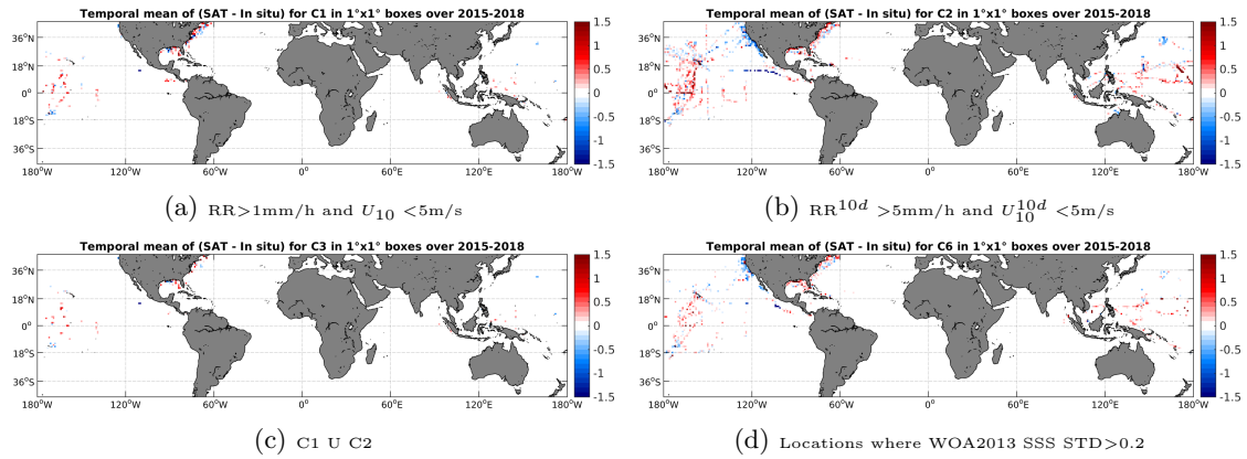
Figure 12: Temporal mean gridded over spatial boxes of size 1^\circ \times 1^\circ of \Delta SSS (SMAP-L3-RSS-V2-8DAY-RUNNING-40KM - TSG-SAMOS) for 4 different subdatasets corresponding to: RR > 1\text{mm/h} and U_{10} < 5\text{m/s} (a), RR^{10d} > 5\text{mm/h} and U_{10}^{10d} < 5\text{m/s} (b), C1 U C2 (c), Locations where WOA2013 SSS STD > 0.2 (d).
