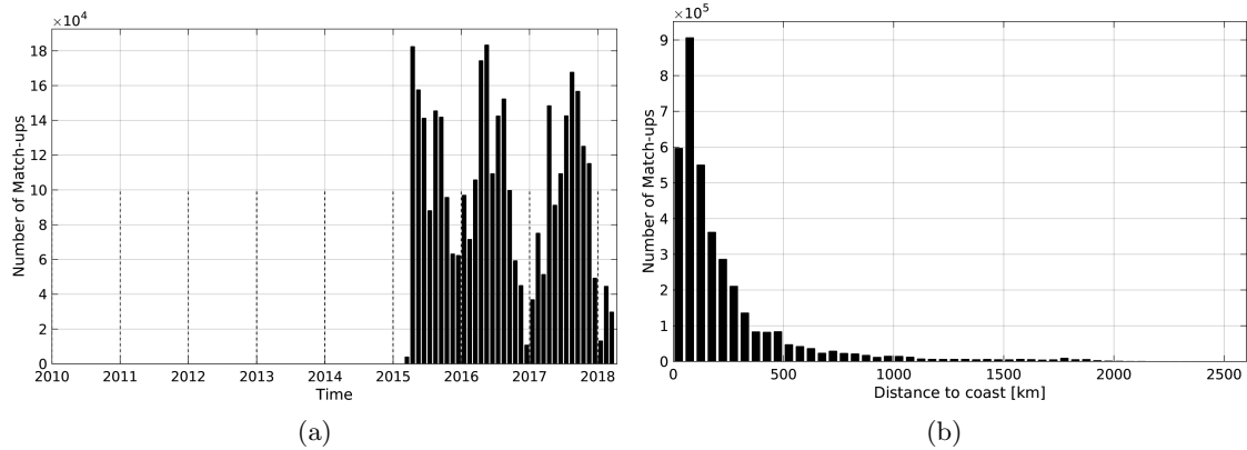
Figure 1: Number of match-ups between TSG-SAMOS and SMAP-L3-RSS-V2-8DAY-RUNNING-40KM SSS as a function of time (a) and as function of the distance to coast (b) over the Mid-Low Latitudes 45N-45S Pi-MEP region and for the full satellite product period.
