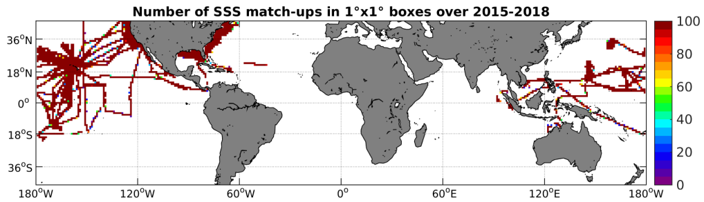
Figure 4: Number of SSS match-ups between TSG-SAMOS SSS and the SMAP-L3-RSS-V2-8DAY-RUNNING-40KM SSS product for the Mid-Low Latitudes 45N-45S Pi-MEP region over 1°x1° boxes and for the full satellite product period.
