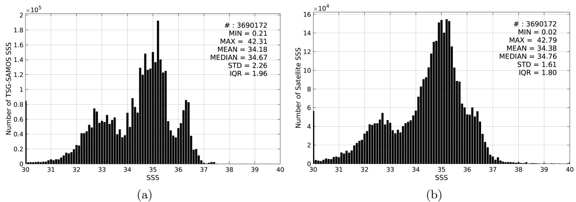
Figure 2: Histograms of SSS from TSG-SAMOS (a) and SMAP-L3-RSS-V2-8DAY-RUNNING-40KM (b) considering all match-up pairs per bins of 0.1 over the Mid-Low Latitudes 45N-45S Pi-MEP region and for the full satellite product period.
