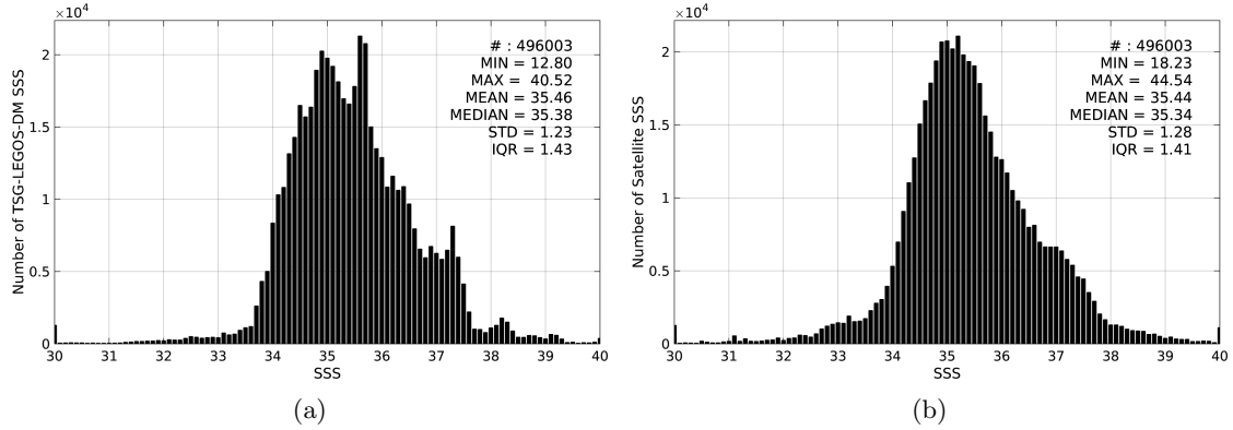
Figure 2: Histograms of SSS from TSG-LEGOS-DM (a) and SMAP-L3-RSS-V2-8DAY-RUNNING-40KM (b) considering all match-up pairs per bins of 0.1 over the Mid-Low Latitudes 45N-45S Pi-MEP region and for the full satellite product period.
