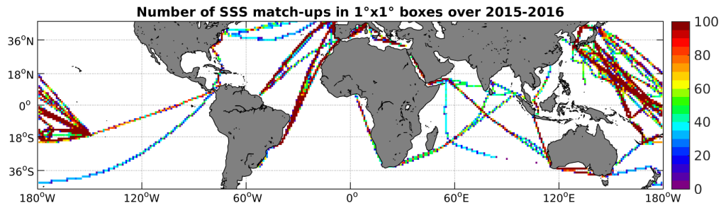
Figure 4: Number of SSS match-ups between TSG-LEGOS-DM SSS and the SMAP-L3-RSS-V2-8DAY-RUNNING-40KM SSS product for the Mid-Low Latitudes 45N-45S Pi-MEP region over 1^\circ \times 1^\circ boxes and for the full satellite product period.
