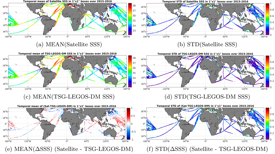
Figure 6: Temporal mean (left) and STD (right) of SSS from SMAP-L3-RSS-V2-8DAY-RUNNING-40KM satellite SSS product (in black), TSG-LEGOS-DM (middle), and of \Delta SSS (Satellite - TSG-LEGOS-DM). Only match-up pairs are used to generate these maps.
