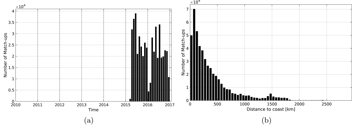
Figure 1: Number of match-ups between TSG-LEGOS-DM and SMAP-L3-RSS-V2-8DAY-RUNNING-40KM SSS as a function of time (a) and as function of the distance to coast (b) over the Mid-Low Latitudes 45N-45S Pi-MEP region and for the full satellite product period.
