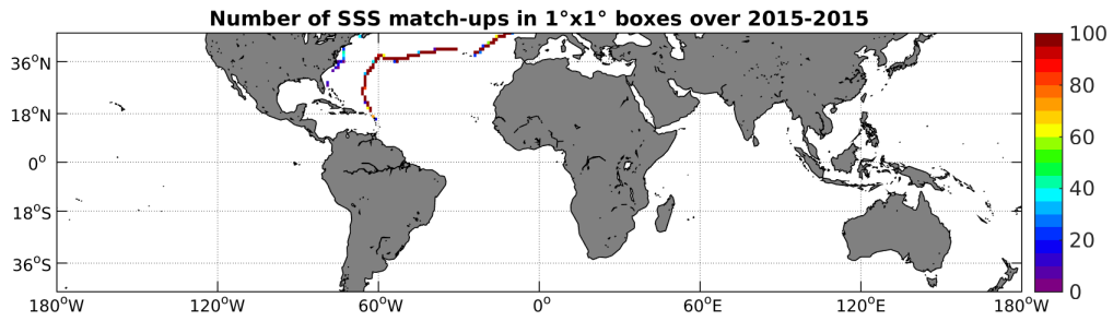
Figure 4: Number of SSS match-ups between TSG-GOSUD-Sailing-ship SSS and the SMAP-L3-RSS-V2-8DAY-RUNNING-40KM SSS product for the Mid-Low Latitudes 45N-45S Pi-MEP region over 1°x1° boxes and for the full satellite product period.
