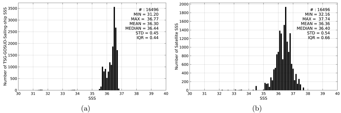
Figure 2: Histograms of SSS from TSG-GOSUD-Sailing-ship (a) and SMAP-L3-RSS-V2-8DAY-RUNNING-40KM (b) considering all match-up pairs per bins of 0.1 over the Mid-Low Latitudes 45N-45S Pi-MEP region and for the full satellite product period.
