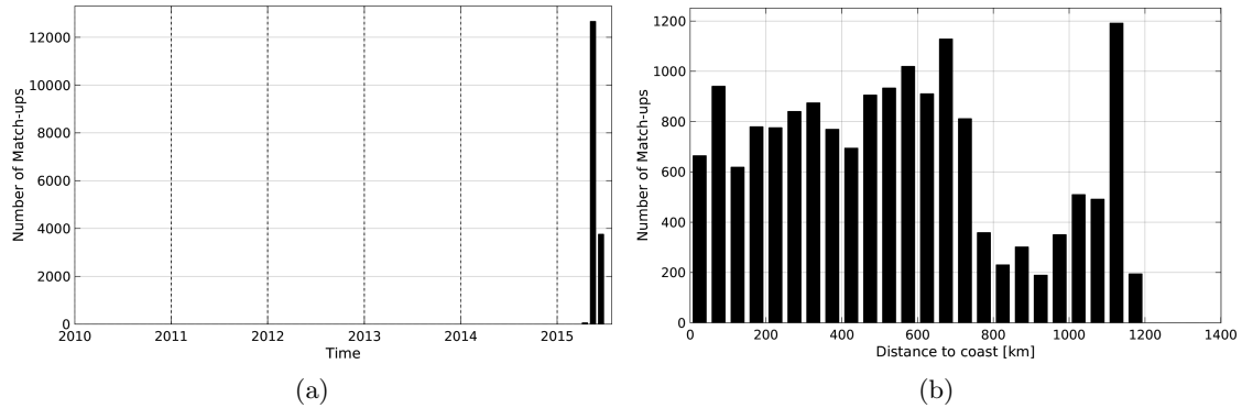
Figure 1: Number of match-ups between TSG-GOSUD-Sailing-ship and SMAP-L3-RSS-V2-8DAY-RUNNING-40KM SSS as a function of time (a) and as function of the distance to coast (b) over the Mid-Low Latitudes 45N-45S Pi-MEP region and for the full satellite product period.
