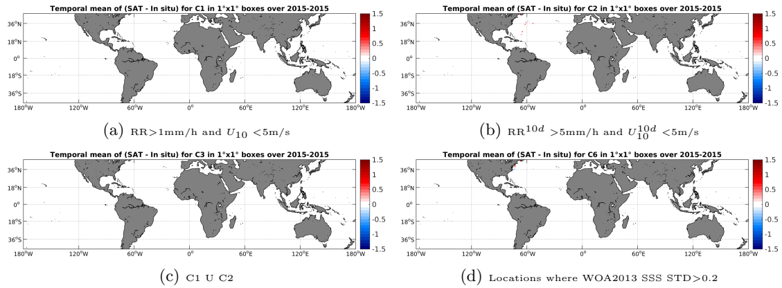
Figure 12: Temporal mean gridded over spatial boxes of size 1^\circ \times 1^\circ of \Delta SSS (SMAP-L3-RSS-V2-8DAY-RUNNING-40KM - TSG-GOSUD-Sailing-ship) for 4 different subdatasets corresponding to: RR > 1 mm/h and U_{10} < 5 m/s (a), RR^{10d} > 5 mm/h and U_{10}^{10d} < 5 m/s (b), C1 U C2 (c), Locations where WOA2013 SSS STD > 0.2 (d).
