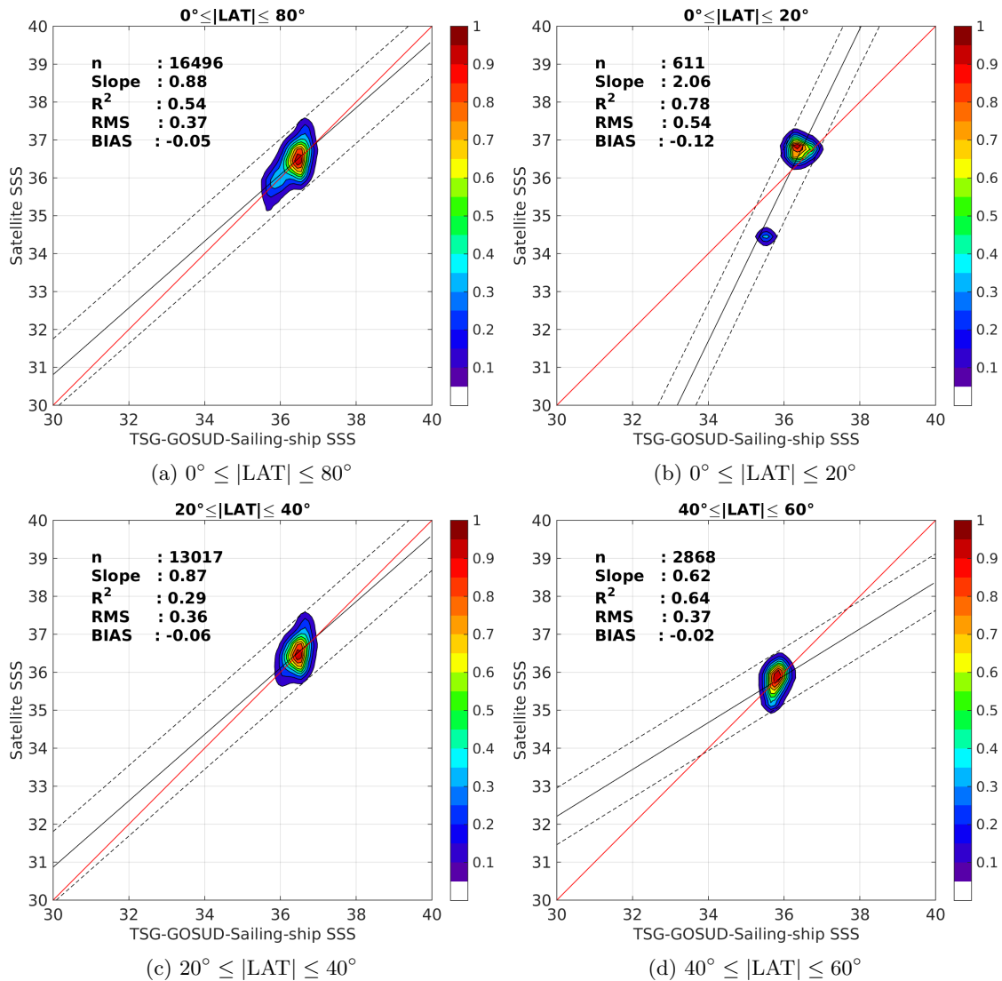
Figure 9: Contour maps of the concentration of SMAP-L3-RSS-V2-8DAY-RUNNING-40KM SSS (y-axis) versus TSG-GOSUD-Sailing-ship SSS (x-axis) at match-up pairs for different latitude bands. For each plot, the red line shows x=y . The black thin and dashed lines indicate a linear fit through the data cloud and the \pm 95\% confidence levels, respectively. The number match-up pairs n , the slope and R^2 coefficient of the linear fit, the root mean square (RMS) and the mean bias between satellite and in situ data are indicated for each latitude band in each plots.
