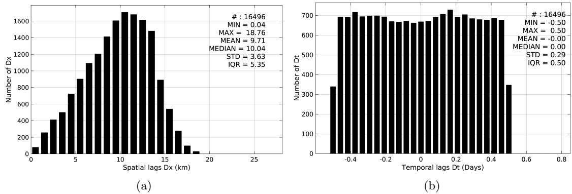
Figure 5: Histograms of the spatial (a) and temporal (b) lags between the time of the TSG-GOSUD-Sailing-ship measurements and the date of the corresponding SMAP-L3-RSS-V2-8DAY-RUNNING-40KM SSS product.
