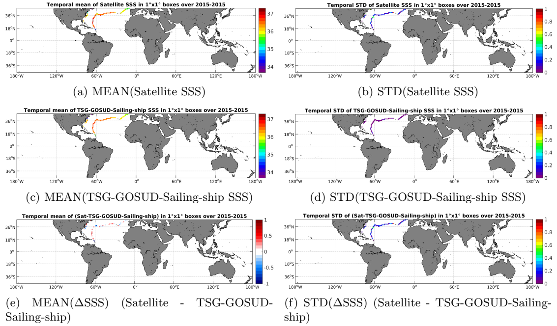
Figure 6: Temporal mean (left) and STD (right) of SSS from SMAP-L3-RSS-V2-8DAY-RUNNING-40KM (top), TSG-GOSUD-Sailing-ship (middle), and of \Delta SSS (Satellite - TSG-GOSUD-Sailing-ship). Only match-up pairs are used to generate these maps.
