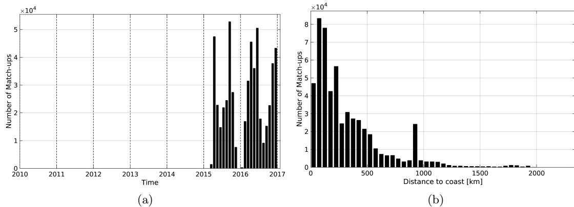
Figure 1: Number of match-ups between TSG-GOSUD-Research-vessel and SMAP-L3-RSS-V2-8DAY-RUNNING-40KM SSS as a function of time (a) and as function of the distance to coast (b) over the Mid-Low Latitudes 45N-45S Pi-MEP region and for the full satellite product period.
