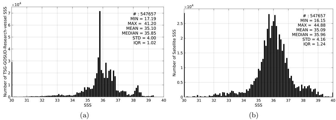
Figure 2: Histograms of SSS from TSG-GOSUD-Research-vessel (a) and SMAP-L3-RSS-V2-8DAY-RUNNING-40KM (b) considering all match-up pairs per bins of 0.1 over the Mid-Low Latitudes 45N-45S Pi-MEP region and for the full satellite product period.
