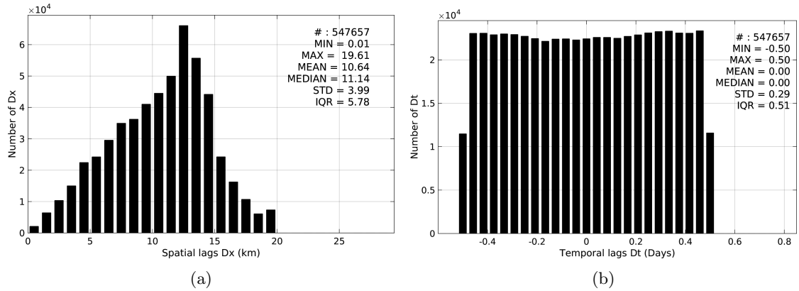
Figure 5: Histograms of the spatial (a) and temporal (b) lags between the time of the TSG-GOSUD-Research-vessel measurements and the date of the corresponding SMAP-L3-RSS-V2-8DAY-RUNNING-40KM SSS product.
