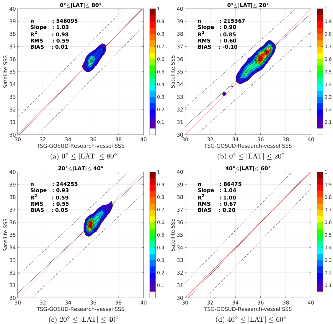
Figure 9: Contour maps of the concentration of SMAP-L3-RSS-V2-8DAY-RUNNING-40KM SSS (y-axis) versus TSG-GOSUD-Research-vessel SSS (x-axis) at match-up pairs for different latitude bands. For each plot, the red line shows x=y . The black thin and dashed lines indicate a linear fit through the data cloud and the \pm 95\% confidence levels, respectively. The number match-up pairs n , the slope and R^2 coefficient of the linear fit, the root mean square (RMS) and the mean bias between satellite and in situ data are indicated for each latitude band in each plots.
