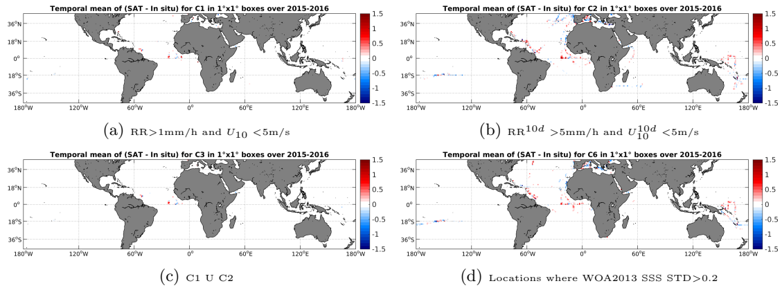
Figure 12: Temporal mean gridded over spatial boxes of size 1^\circ \times 1^\circ of \Delta SSS (SMAP-L3-RSS-V2-8DAY-RUNNING-40KM - TSG-GOSUD-Research-vessel) for 4 different subdatasets corresponding to: RR > 1\text{mm/h} and U_{10} < 5\text{m/s} (a), RR^{10d} > 5\text{mm/h} and U_{10}^{10d} < 5\text{m/s} (b), C1 U C2 (c), Locations where WOA2013 SSS STD > 0.2 (d).
