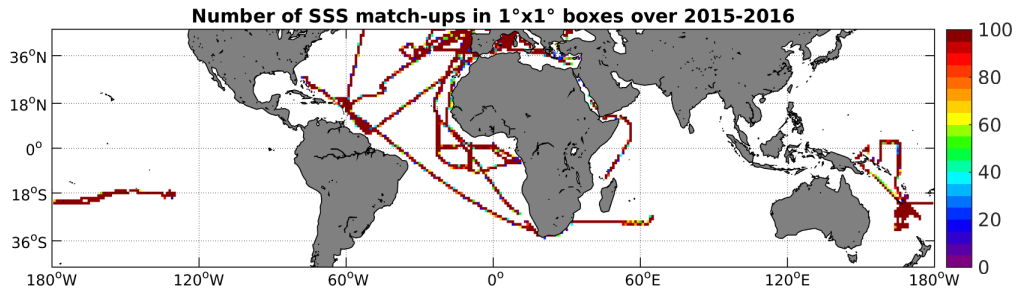
Figure 4: Number of SSS match-ups between TSG-GOSUD-Research-vessel SSS and the SMAP-L3-RSS-V2-8DAY-RUNNING-40KM SSS product for the Mid-Low Latitudes 45N-45S Pi-MEP region over 1^\circ \times 1^\circ boxes and for the full satellite product period.
