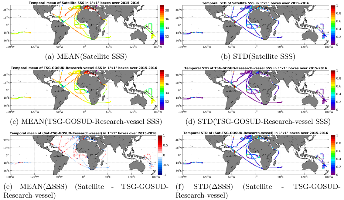
Figure 6: Temporal mean (left) and STD (right) of SSS from SMAP-L3-RSS-V2-8DAY-RUNNING-40KM satellite SSS product (in black) and the TSG-GOSUD-Research-vessel in situ dataset (in blue) at the collected Pi-MEP match-up pairs. Only match-up pairs are used to generate these maps.
