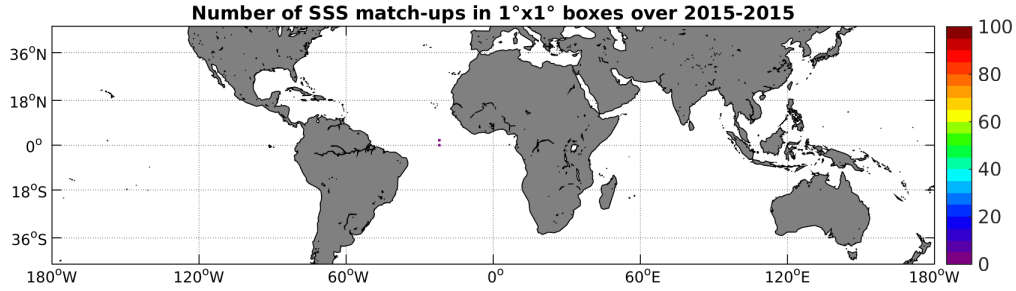
Figure 3: Number of SSS match-ups between Surface drifters SSS and the SMAP-L3-RSS-V2-8DAY-RUNNING-40KM SSS product for the Mid-Low Latitudes 45N-45S Pi-MEP region over 1^\circ \times 1^\circ boxes and for the full satellite product period.
