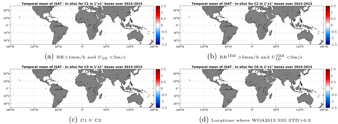
Figure 11: Temporal mean gridded over spatial boxes of size 1^\circ \times 1^\circ of \Delta SSS (SMAP-L3-RSS-V2-8DAY-RUNNING-40KM - Surface drifters) for 4 different subdatasets corresponding to: RR > 1\text{mm/h} and U_{10} < 5\text{m/s} (a), RR^{10d} > 5\text{mm/h} and U_{10}^{10d} < 5\text{m/s} (b), C1 U C2 (c), Locations where WOA2013 SSS STD > 0.2 (d).
