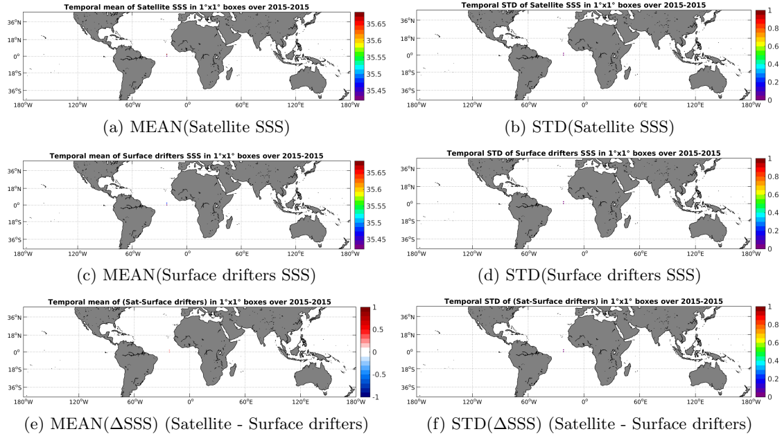
Figure 5: Temporal mean (left) and STD (right) of SSS from SMAP-L3-RSS-V2-8DAY-RUNNING-40KM (top), Surface drifters (middle), and of \Delta SSS (Satellite - Surface drifters). Only match-up pairs are used to generate these maps.
