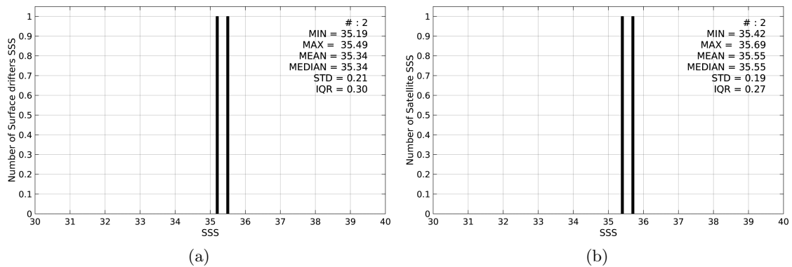
Figure 2: Histograms of SSS from Surface drifters (a) and SMAP-L3-RSS-V2-8DAY-RUNNING-40KM (b) considering all match-up pairs per bins of 0.1 over the Mid-Low Latitudes 45N-45S Pi-MEP region and for the full satellite product period.
