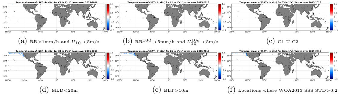
Figure 12: Temporal mean gridded over spatial boxes of size 1^\circ \times 1^\circ of \Delta SSS (SMAP-L3-RSS-V2-8DAY-RUNNING-70KM - Sea mammals) for 6 different subdatasets corresponding to: RR > 1\text{mm/h} and U_{10} < 5\text{m/s} (a), RR^{10d} > 5\text{mm/h} and U_{10}^{10d} < 5\text{m/s} (b), C1 U C2 (c), MLD < 20\text{m} (d), BLT > 10\text{m} (e), Locations where WOA2013 SSS STD > 0.2 (f).
