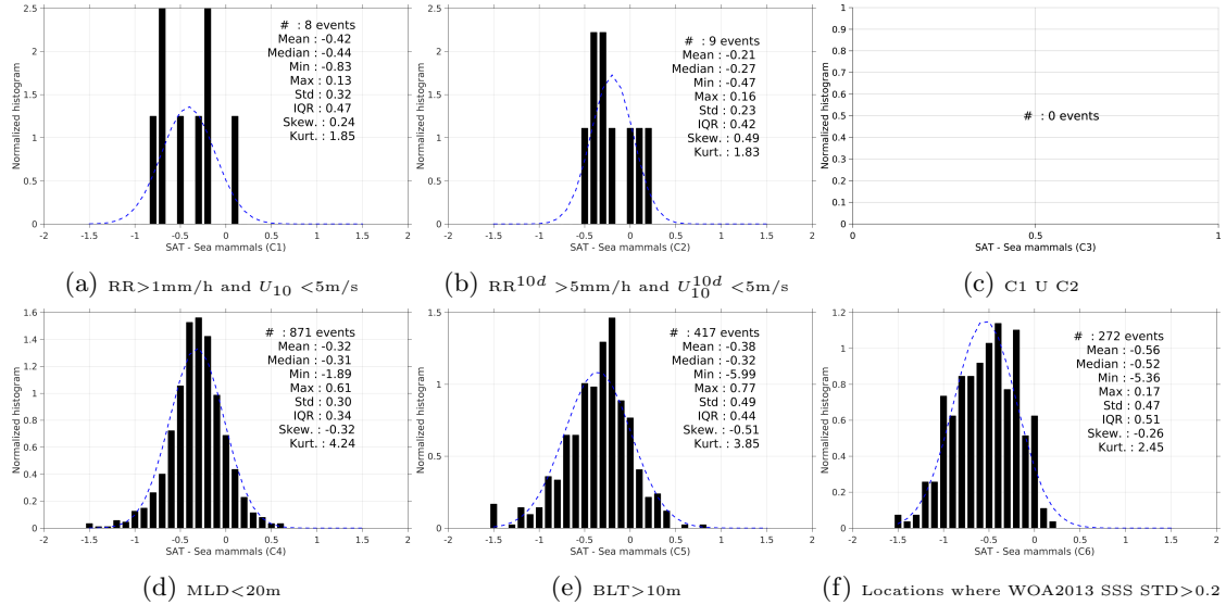
Figure 13: Normalized histogram of \Delta SSS (SMAP-L3-RSS-V2-8DAY-RUNNING-70KM - Sea mammals) for 6 different subdatasets corresponding to: RR > 1\text{mm/h} and U_{10} < 5\text{m/s} (a), RR^{10d} > 5\text{mm/h} and U_{10}^{10d} < 5\text{m/s} (b), C1 U C2 (c), MLD < 20\text{m} (d), BLT > 10\text{m} (e), Locations where WOA2013 SSS STD > 0.2 (f).
