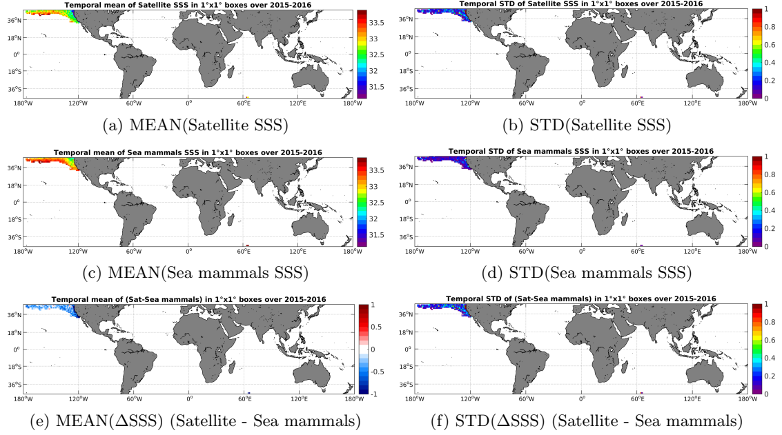
Figure 6: Temporal mean (left) and STD (right) of SSS from SMAP-L3-RSS-V2-8DAY-RUNNING-70KM (top), Sea mammals (middle), and of \Delta SSS (Satellite - Sea mammals). Only match-up pairs are used to generate these maps.
