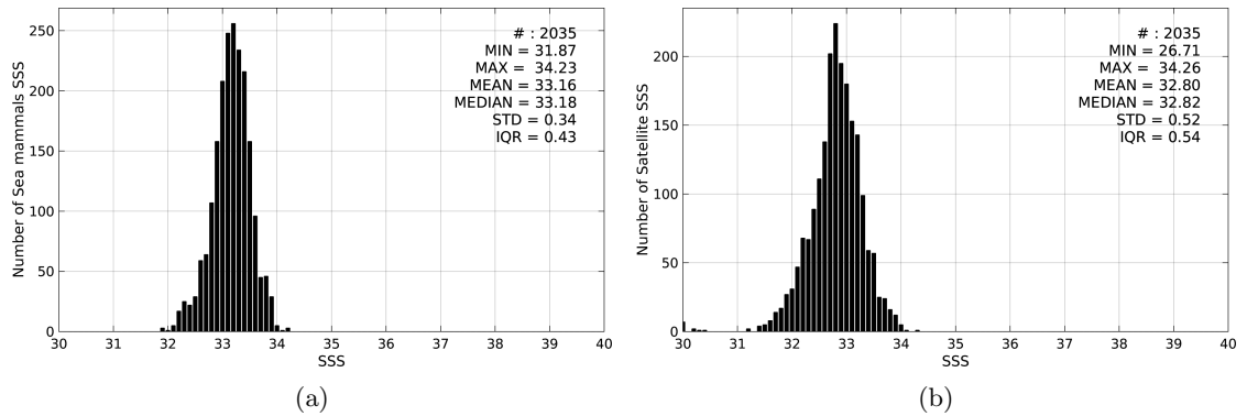
Figure 2: Histograms of SSS from Sea mammals (a) and SMAP-L3-RSS-V2-8DAY-RUNNING-70KM (b) considering all match-up pairs per bins of 0.1 over the Mid-Low Latitudes 45N-45S Pi-MEP region and for the full satellite product period.
