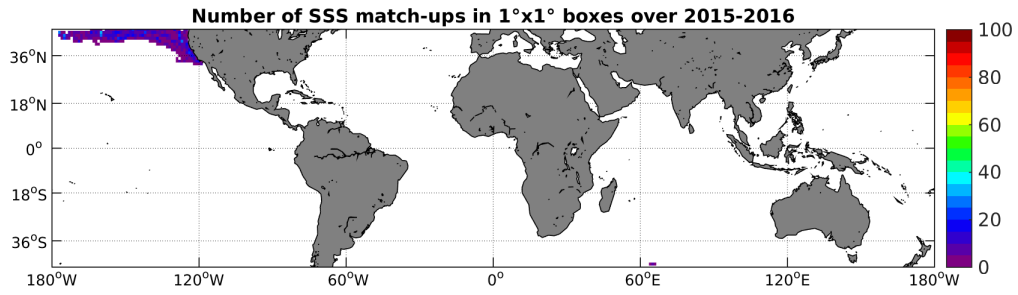
Figure 4: Number of SSS match-ups between Sea mammals SSS and the SMAP-L3-RSS-V2-8DAY-RUNNING-70KM SSS product for the Mid-Low Latitudes 45N-45S Pi-MEP region over 1^\circ \times 1^\circ boxes and for the full satellite product period.
