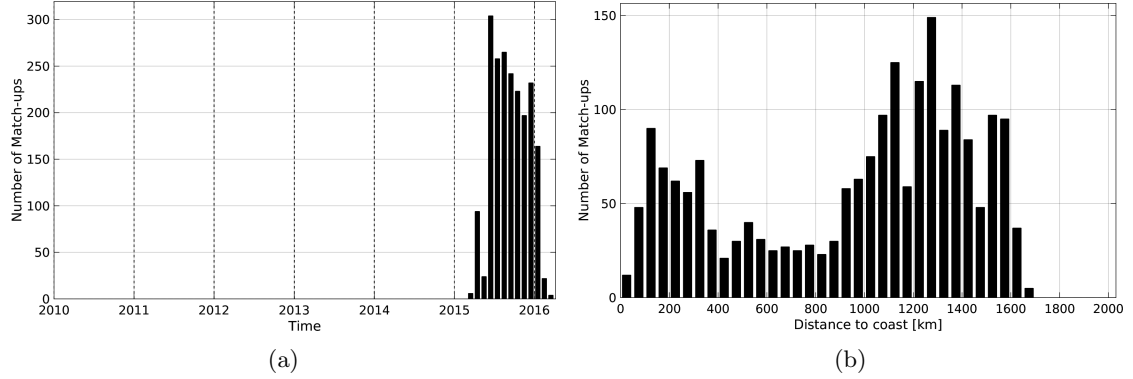
Figure 1: Number of match-ups between Sea mammals and SMAP-L3-RSS-V2-8DAY-RUNNING-70KM SSS as a function of time (a) and as function of the distance to coast (b) over the Mid-Low Latitudes 45N-45S Pi-MEP region and for the full satellite product period.
