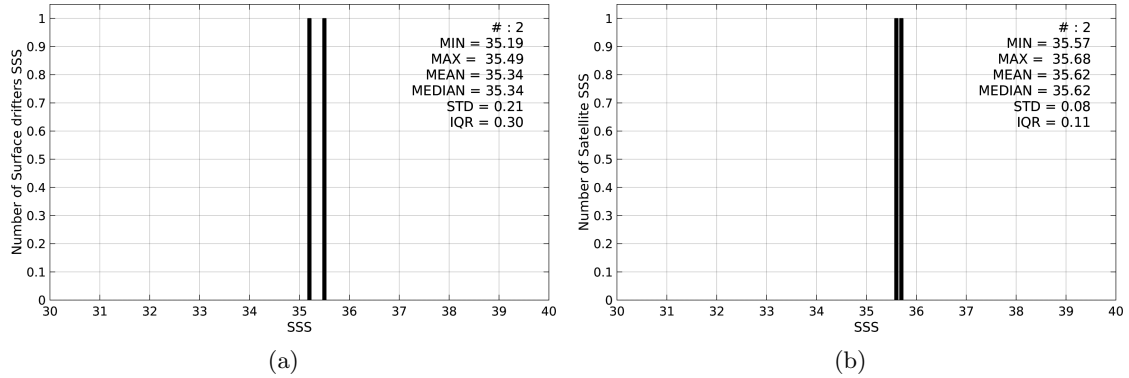
Figure 2: Histograms of SSS from Surface drifters (a) and SMAP-L3-RSS-V2-8DAY-RUNNING-70KM (b) considering all match-up pairs per bins of 0.1 over the Mid-Low Latitudes 45N-45S Pi-MEP region and for the full satellite product period.
