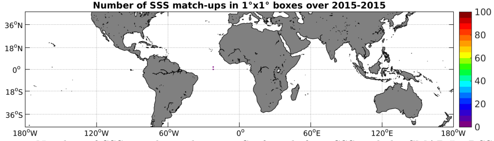
Figure 3: Number of SSS match-ups between Surface drifters SSS and the SMAP-L3-RSS-V2-8DAY-RUNNING-70KM SSS product for the Mid-Low Latitudes 45N-45S Pi-MEP region over 1°x1° boxes and for the full satellite product period.
