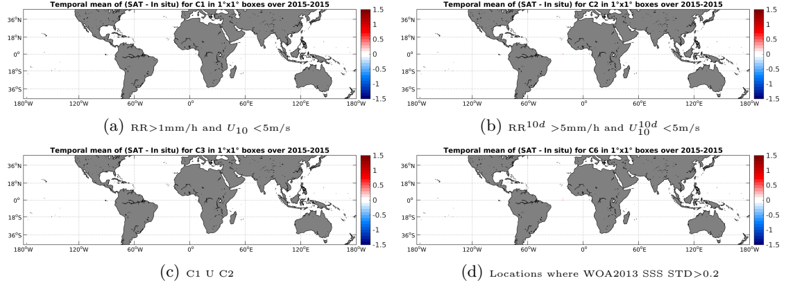
Figure 11: Temporal mean gridded over spatial boxes of size 1^\circ \times 1^\circ of \Delta SSS (SMAP-L3-RSS-V2-8DAY-RUNNING-70KM - Surface drifters) for 4 different subdatasets corresponding to: RR > 1\text{mm/h} and U_{10} < 5\text{m/s} (a), RR^{10d} > 5\text{mm/h} and U_{10}^{10d} < 5\text{m/s} (b), C1 U C2 (c), Locations where WOA2013 SSS STD > 0.2 (d).
