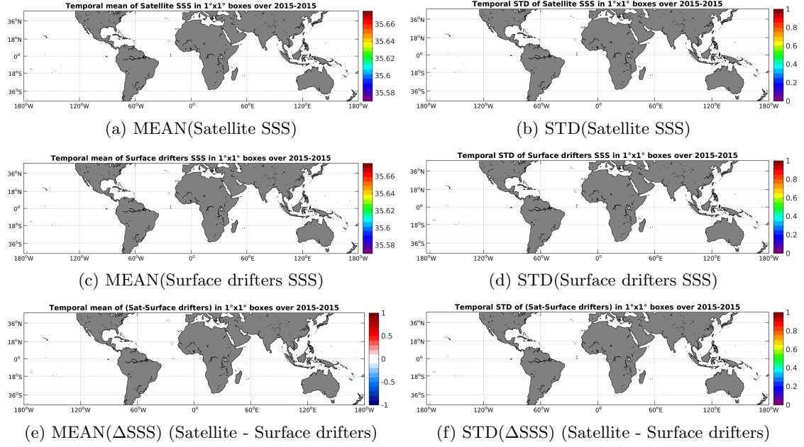
Figure 5: Temporal mean (left) and STD (right) of SSS from SMAP-L3-RSS-V2-8DAY-RUNNING-70KM (top), Surface drifters (middle), and of \Delta SSS (Satellite - Surface drifters). Only match-up pairs are used to generate these maps.
