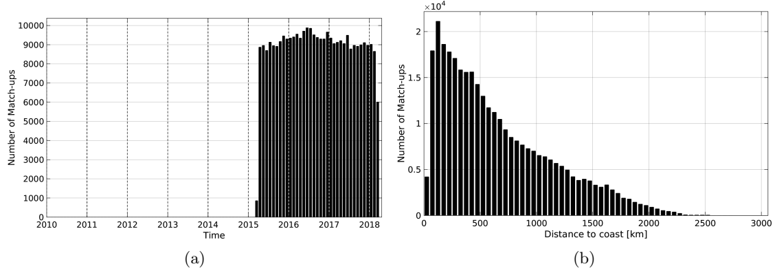
Figure 1: Number of match-ups between Argo and SMAP-L3-RSS-V2-8DAY-RUNNING-70KM SSS as a function of time (a) and as function of the distance to coast (b) over the Mid-Low Latitudes 45N-45S Pi-MEP region and for the full satellite product period.
