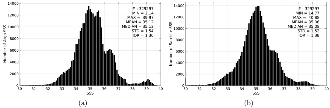
Figure 2: Histograms of SSS from Argo (a) and SMAP-L3-RSS-V2-8DAY-RUNNING-70KM (b) considering all match-up pairs per bins of 0.1 over the Mid-Low Latitudes 45N-45S Pi-MEP region and for the full satellite product period.
