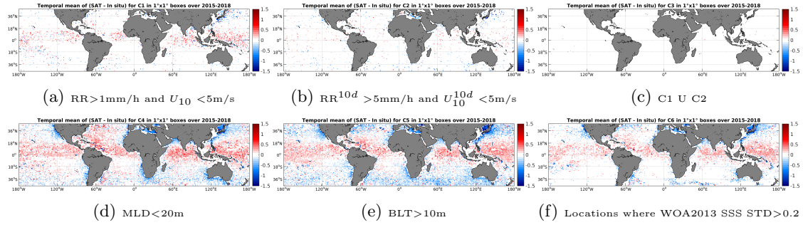
Figure 12: Temporal mean gridded over spatial boxes of size 1^\circ \times 1^\circ of \Delta SSS (SMAP-L3-RSS-V2-8DAY-RUNNING-70KM - Argo) for 6 different subdatasets corresponding to: RR>1mm/h and U_{10} < 5\text{m/s} (a), RR^{10d} > 5\text{mm/h} and U_{10}^{10d} < 5\text{m/s} (b), C1 U C2 (c), MLD<20m (d), BLT>10m (e), Locations where WOA2013 SSS STD>0.2 (f).
