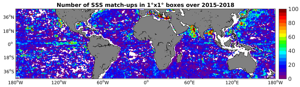
Figure 4: Number of SSS match-ups between Argo SSS and the SMAP-L3-RSS-V2-8DAY-RUNNING-70KM SSS product for the Mid-Low Latitudes 45N-45S Pi-MEP region over 1^\circ \times 1^\circ boxes and for the full satellite product period.
