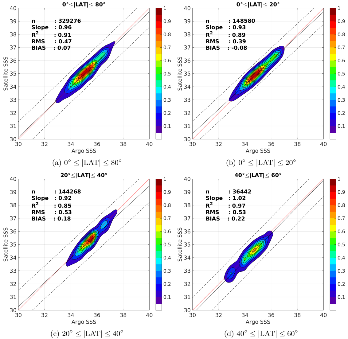
Figure 9: Contour maps of the concentration of SMAP-L3-RSS-V2-8DAY-RUNNING-70KM SSS (y-axis) versus Argo SSS (x-axis) at match-up pairs for different latitude bands. For each plot, the red line shows x=y . The black thin and dashed lines indicate a linear fit through the data cloud and the \pm 95\% confidence levels, respectively. The number match-up pairs n , the slope and R^2 coefficient of the linear fit, the root mean square (RMS) and the mean bias between satellite and in situ data are indicated for each latitude band in each plots.
