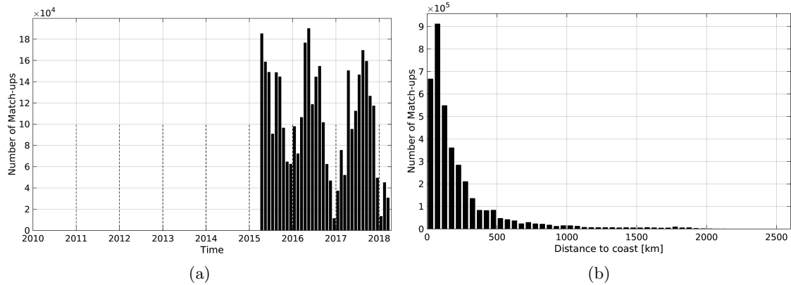
Figure 1: Number of match-ups between TSG-SAMOS and SMAP-L3-RSS-V2-MONTHLY-0.25DEG-40KM SSS as a function of time (a) and as function of the distance to coast (b) over the Mid-Low Latitudes 45N-45S Pi-MEP region and for the full satellite product period.
