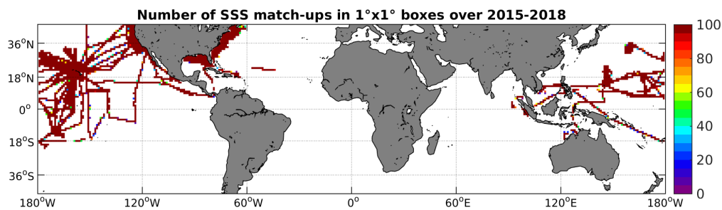
Figure 4: Number of SSS match-ups between TSG-SAMOS SSS and the SMAP-L3-RSS-V2-MONTHLY-0.25DEG-40KM SSS product for the Mid-Low Latitudes 45N-45S Pi-MEP region over 1^\circ \times 1^\circ boxes and for the full satellite product period.
