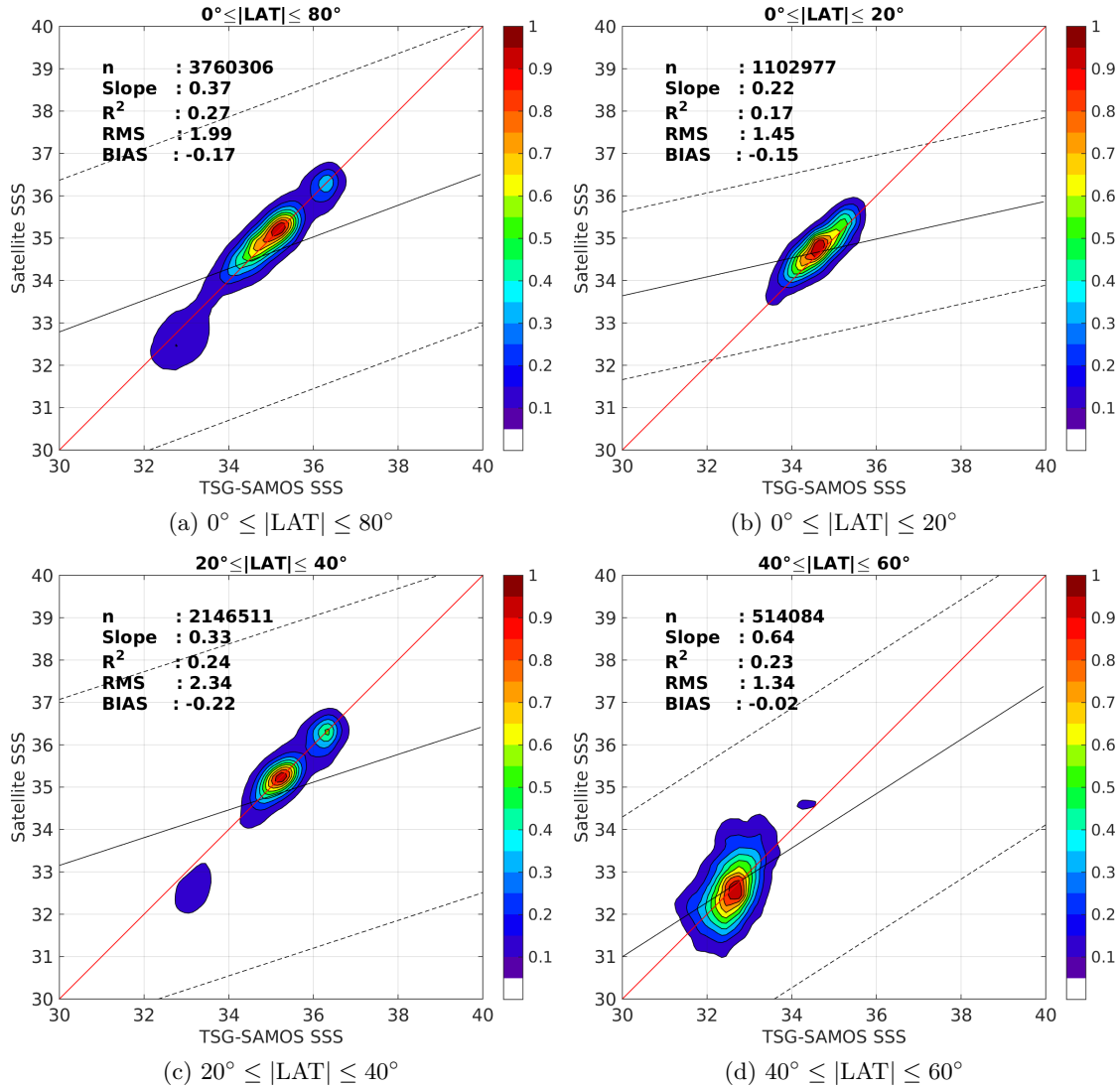
Figure 9: Contour maps of the concentration of SMAP-L3-RSS-V2-MONTHLY-0.25DEG-40KM SSS (y-axis) versus TSG-SAMOS SSS (x-axis) at match-up pairs for different latitude bands. For each plot, the red line shows x=y . The black thin and dashed lines indicate a linear fit through the data cloud and the \pm 95\% confidence levels, respectively. The number match-up pairs n , the slope and R^2 coefficient of the linear fit, the root mean square (RMS) and the mean bias between satellite and in situ data are indicated for each latitude band in each plots.
