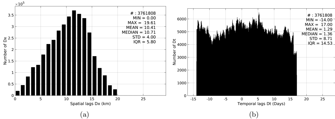
Figure 5: Histograms of the spatial (a) and temporal (b) lags between the time of the TSG-SAMOS measurements and the date of the corresponding SMAP-L3-RSS-V2-MONTHLY-0.25DEG-40KM SSS product.
