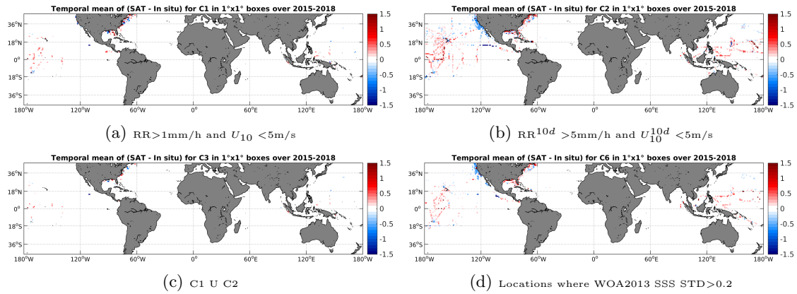
Figure 12: Temporal mean gridded over spatial boxes of size 1^\circ \times 1^\circ of \Delta SSS (SMAP-L3-RSS-V2-MONTHLY-0.25DEG-40KM - TSG-SAMOS) for 4 different subdatasets corresponding to: RR > 1\text{mm/h} and U_{10} < 5\text{m/s} (a), RR^{10d} > 5\text{mm/h} and U_{10}^{10d} < 5\text{m/s} (b), C1 U C2 (c), Locations where WOA2013 SSS STD > 0.2 (d).
