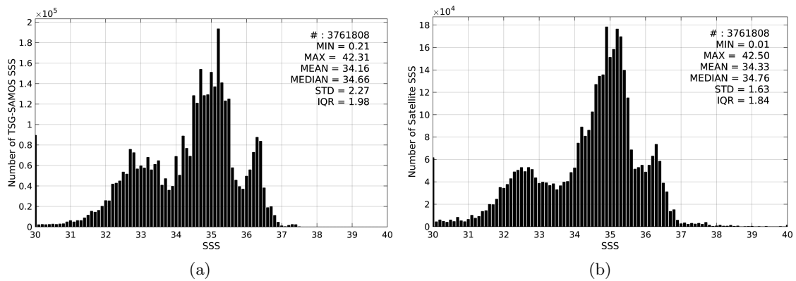
Figure 2: Histograms of SSS from TSG-SAMOS (a) and SMAP-L3-RSS-V2-MONTHLY-0.25DEG-40KM (b) considering all match-up pairs per bins of 0.1 over the Mid-Low Latitudes 45N-45S Pi-MEP region and for the full satellite product period.
