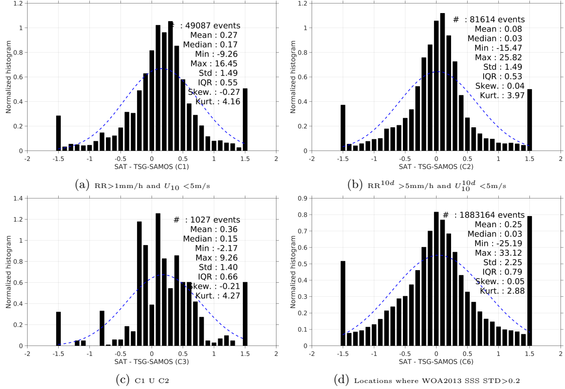
Figure 13: Normalized histogram of \Delta\text{SSS} (SMAP-L3-RSS-V2-MONTHLY-0.25DEG-40KM - TSG-SAMOS) for 6 different subdatasets corresponding to: RR>1mm/h and U_{10} < 5\text{m/s} (a), RR^{10d} > 5\text{mm/h} and U_{10}^{10d} < 5\text{m/s} (b), C1 U C2 (c), Locations where WOA2013 SSS STD>0.2 (d).
