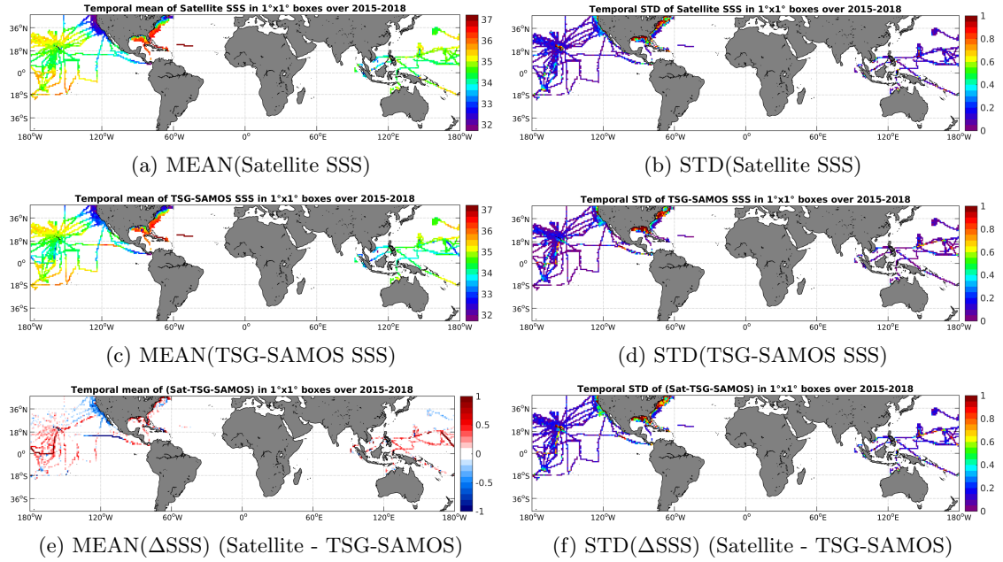
Figure 6: Temporal mean (left) and STD (right) of SSS from SMAP-L3-RSS-V2-MONTHLY-0.25DEG-40KM (top), TSG-SAMOS (middle), and of \Delta SSS (Satellite - TSG-SAMOS). Only match-up pairs are used to generate these maps.
