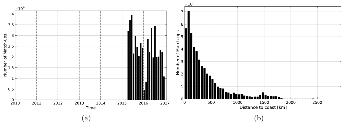
Figure 1: Number of match-ups between TSG-LEGOS-DM and SMAP-L3-RSS-V2-MONTHLY-0.25DEG-40KM SSS as a function of time (a) and as function of the distance to coast (b) over the Mid-Low Latitudes 45N-45S Pi-MEP region and for the full satellite product period.
