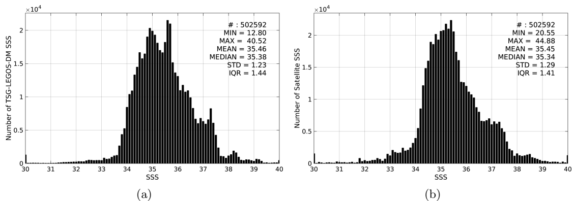
Figure 2: Histograms of SSS from TSG-LEGOS-DM (a) and SMAP-L3-RSS-V2-MONTHLY-0.25DEG-40KM (b) considering all match-up pairs per bins of 0.1 over the Mid-Low Latitudes 45N-45S Pi-MEP region and for the full satellite product period.
