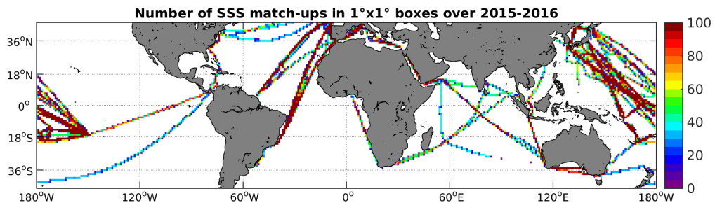
Figure 4: Number of SSS match-ups between TSG-LEGOS-DM SSS and the SMAP-L3-RSS-V2-MONTHLY-0.25DEG-40KM SSS product for the Mid-Low Latitudes 45N-45S Pi-MEP region over 1^\circ \times 1^\circ boxes and for the full satellite product period.
